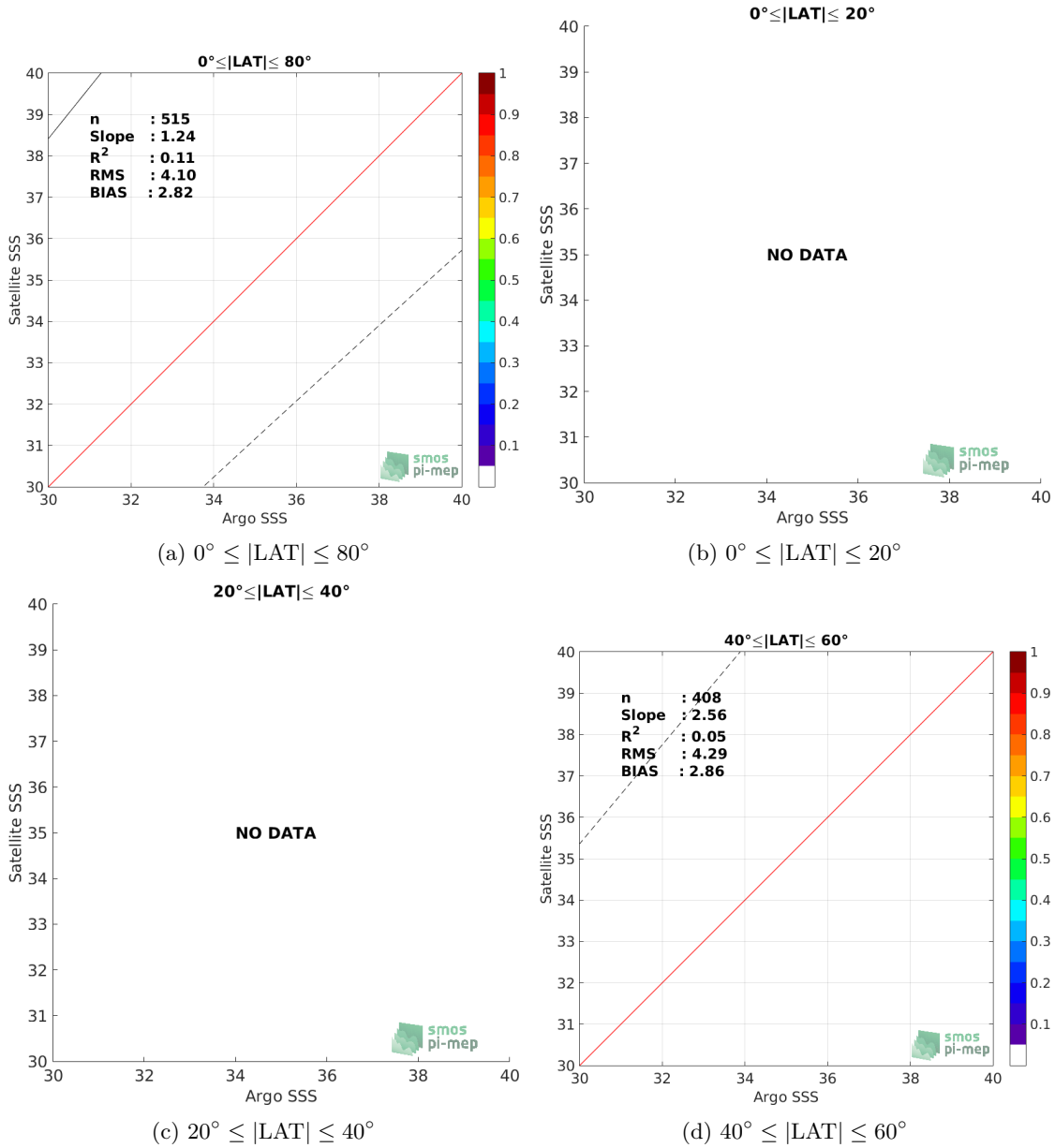
Figure 9: Contour maps of the concentration of SMAP-L2-JPL-V4 SSS (y-axis) versus Argo SSS (x-axis) at match-up pairs for different latitude bands. For each plot, the red line shows x=y . The black thin and dashed lines indicate a linear fit through the data cloud and the \pm 95\% confidence levels, respectively. The number match-up pairs n , the slope and R^2 coefficient of the linear fit, the root mean square (RMS) and the mean bias between satellite and in situ data are indicated for each latitude band in each plots.
