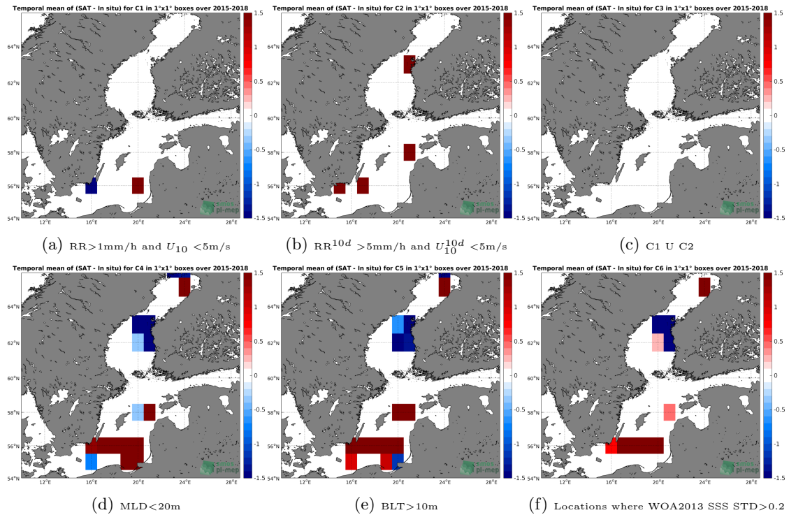
Figure 12: Temporal mean gridded over spatial boxes of size 1^\circ \times 1^\circ of \Delta\text{SSS} (SMAP-L2-JPL-V4 - Argo) for 6 different subdatasets corresponding to: \text{RR} > 1\text{mm/h} and U_{10} < 5\text{m/s} (a), \text{RR}^{10d} > 5\text{mm/h} and U_{10}^{10d} < 5\text{m/s} (b), C1 U C2 (c), \text{MLD} < 20\text{m} (d), \text{BLT} > 10\text{m} (e), Locations where WOA2013 SSS STD > 0.2 (f).
