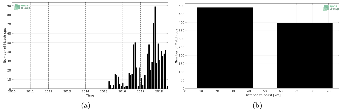
Figure 1: Number of match-ups between Argo and SMAP-L2-JPL-V4 SSS as a function of time (a) and as function of the distance to coast (b) over the Baltic Sea Pi-MEP region and for the full satellite product period.
