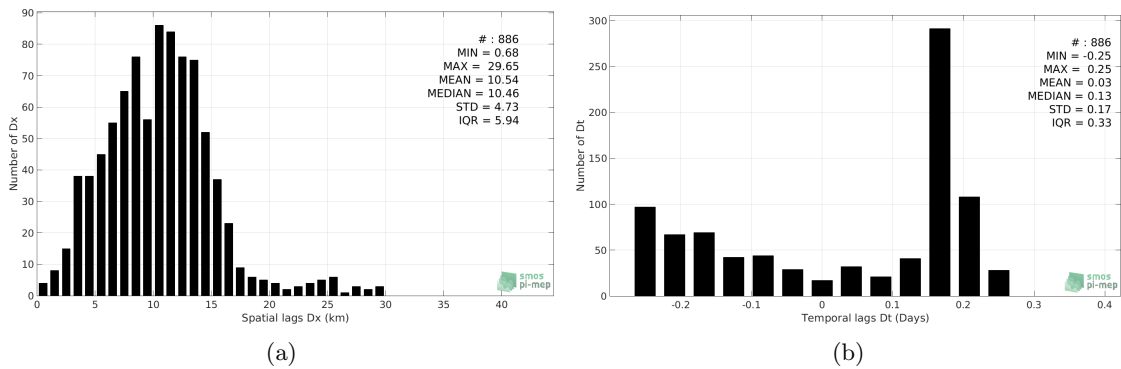
Figure 5: Histograms of the spatial (a) and temporal (b) lags between the time of the Argo measurements and the date of the corresponding SMAP-L2-JPL-V4 SSS product.
