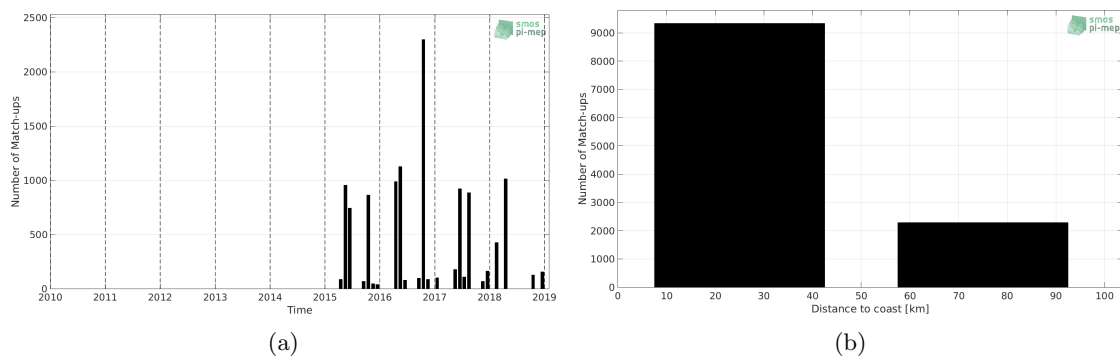
Figure 1: Number of match-ups between TSG-LEGOS-DM and SMAP-L2-JPL-V4.3 SSS as a function of time (a) and as function of the distance to coast (b) over the Baltic Sea Pi-MEP region and for the full satellite product period.
