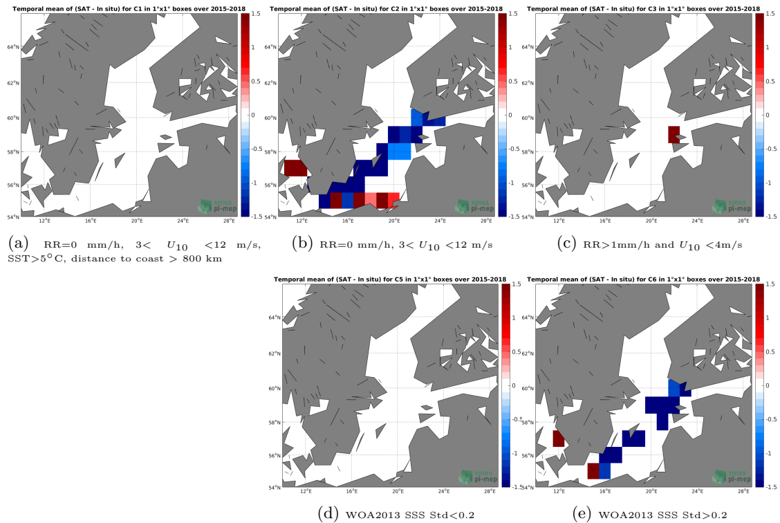
Figure 12: Temporal mean gridded over spatial boxes of size 1^\circ \times 1^\circ of \Delta SSS (SMAP-L2-JPL-V4.3 - TSG-LEGOS-DM) for 5 different subdatasets corresponding to:RR=0 mm/h, 3 < U_{10} < 12 m/s, SST >5^\circ C, distance to coast > 800 km (a), RR=0 mm/h, 3 < U_{10} < 12 m/s (b), RR >1 mm/h and U_{10} < 4 m/s (c), WOA2013 SSS Std <0.2 (d), WOA2013 SSS Std >0.2 (e).
