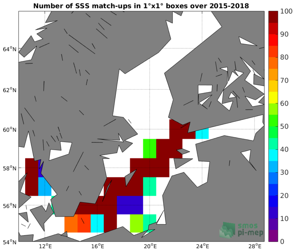
Figure 4: Number of SSS match-ups between TSG-LEGOS-DM SSS and the SMAP-L2-JPL-V4.3 SSS product for the Baltic Sea Pi-MEP region over 1°x1° boxes and for the full satellite product period.
