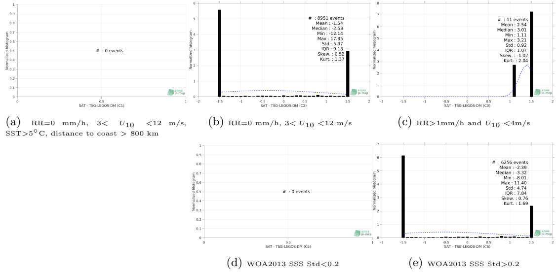
Figure 13: Normalized histogram of \Delta SSS (SMAP-L2-JPL-V4.3 - TSG-LEGOS-DM) for 5 different subdatasets corresponding to: RR=0 mm/h, 3 < U_{10} < 12 m/s, SST > 5°C, distance to coast > 800 km (a), RR=0 mm/h, 3 < U_{10} < 12 m/s (b), RR > 1mm/h and U_{10} < 4 m/s (c), WOA2013 SSS Std < 0.2 (d), WOA2013 SSS Std > 0.2 (e).
