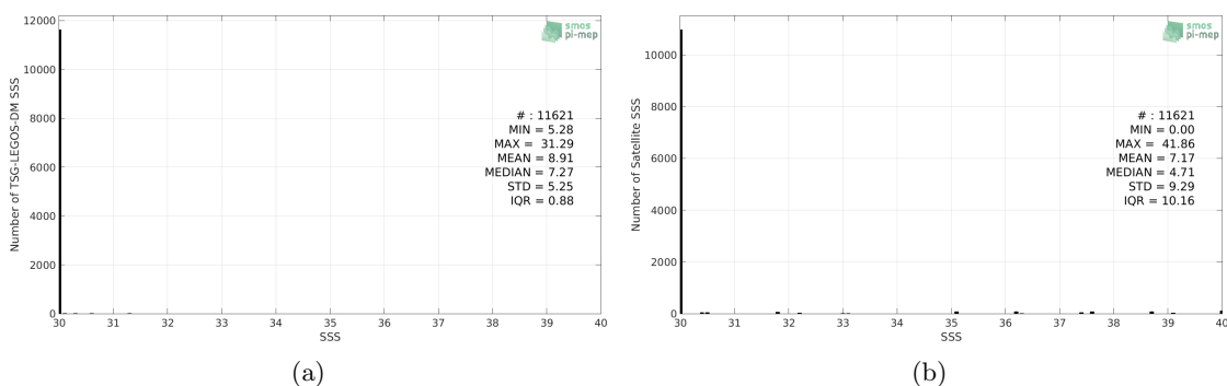
Figure 2: Histograms of SSS from TSG-LEGOS-DM (a) and SMAP-L2-JPL-V4.3 (b) considering all match-up pairs per bins of 0.1 over the Baltic Sea Pi-MEP region and for the full satellite product period.
