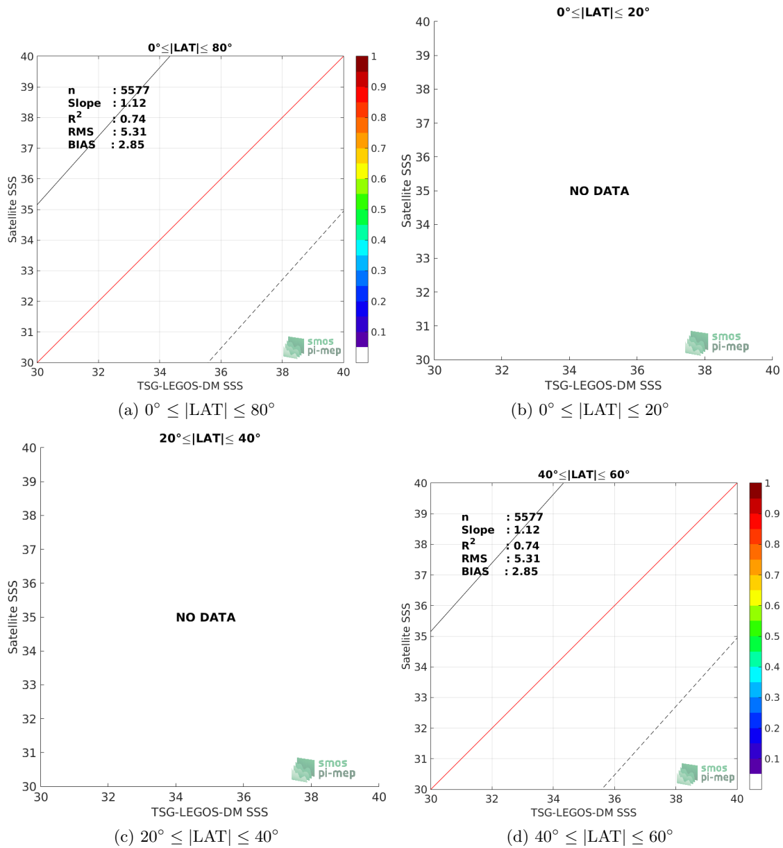
Figure 9: Contour maps of the concentration of SMAP-L2-JPL-V4.3 SSS (y-axis) versus TSG-LEGOS-DM SSS (x-axis) at match-up pairs for different latitude bands. For each plot, the red line shows x=y . The black thin and dashed lines indicate a linear fit through the data cloud and the \pm 95\% confidence levels, respectively. The number match-up pairs n , the slope and R^2 coefficient of the linear fit, the root mean square (RMS) and the mean bias between satellite and in situ data are indicated for each latitude band in each plots.
