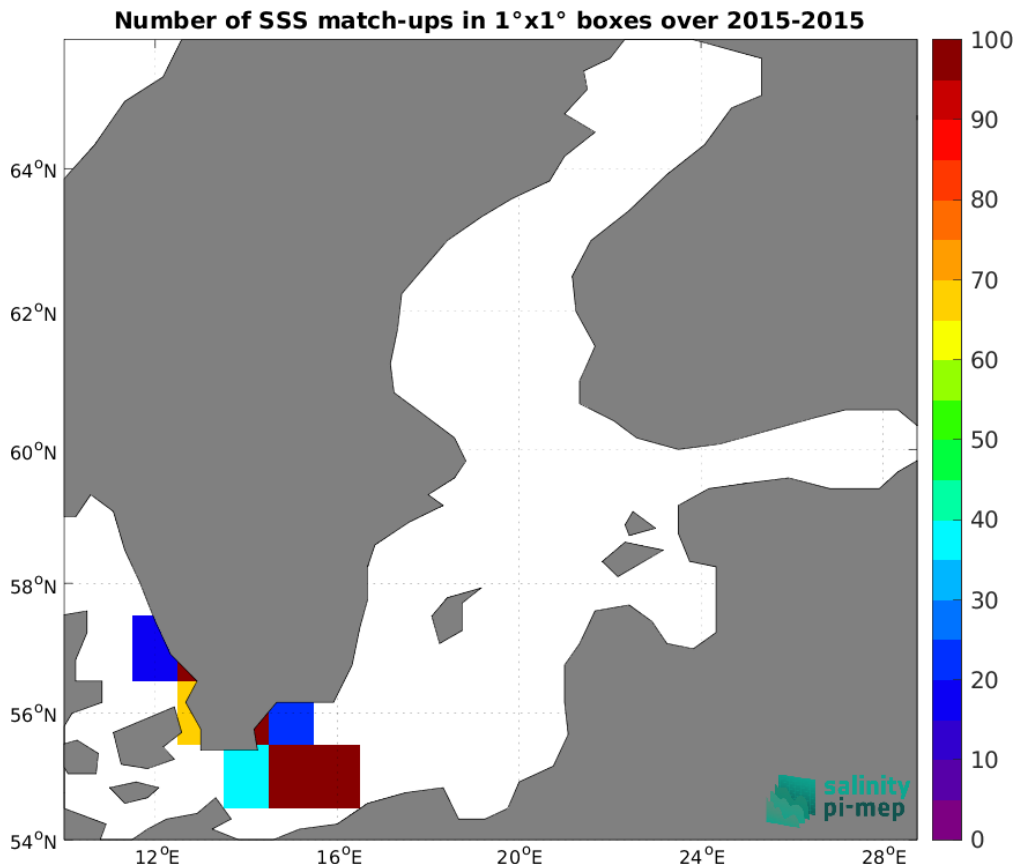
Figure 5: Number of SSS match-ups between TSG (GOSUD-Research-vessel) SSS and the ISAS SSS product for the Baltic Sea Pi-MEP region over 1^\circ \times 1^\circ boxes and for the full satellite product period.
