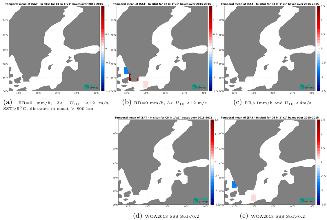
Figure 14: Temporal mean gridded over spatial boxes of size 1^\circ \times 1^\circ of \Delta SSS (ISAS - TSG (GOSUD-Research-vessel)) for 5 different subdatasets corresponding to:RR=0 mm/h, 3 < U_{10} < 12 m/s, SST > 5°C, distance to coast > 800 km (a), RR=0 mm/h, 3 < U_{10} < 12 m/s (b), RR > 1mm/h and U_{10} < 4 m/s (c), WOA2013 SSS Std < 0.2 (d), WOA2013 SSS Std > 0.2 (e).
