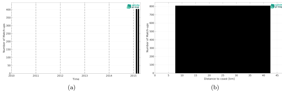
Figure 2: Number of match-ups between TSG (GOSUD-Research-vessel) and ISAS SSS as a function of time (a) and as function of the distance to coast (b) over the Baltic Sea Pi-MEP region and for the full satellite product period.
