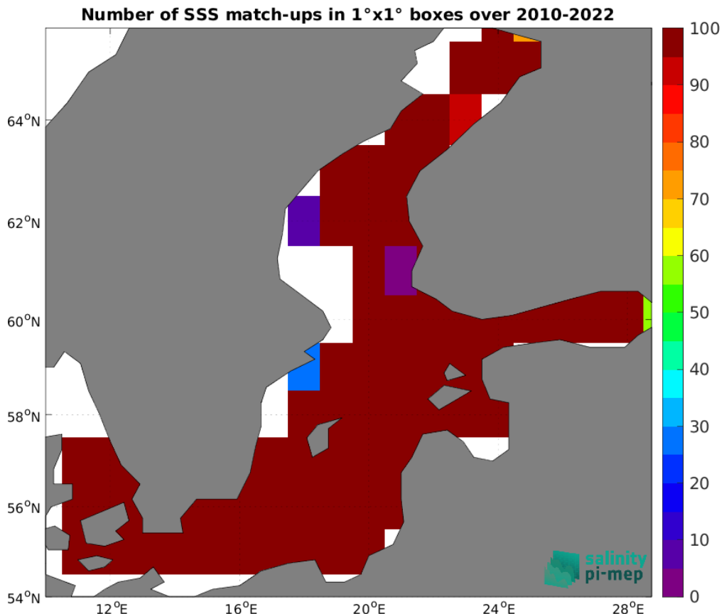
Figure 5: Number of SSS match-ups between ICES SSS and the ISAS v7 - Monthly (Ifremer-LOPS-CMEMS) SSS product for the Baltic Sea Pi-MEP region over 1°x1° boxes and for the full satellite product period.
