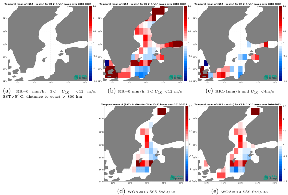
Figure 14: Temporal mean gridded over spatial boxes of size 1^\circ \times 1^\circ of \Delta SSS (ISAS v7 - Monthly (Ifremer-LOPS-CMEMS) - ICES) for 5 different subdatasets corresponding to:RR=0 mm/h, 3 < U_{10} < 12 m/s, SST >5^\circ\text{C} , distance to coast > 800 km (a), RR=0 mm/h, 3 < U_{10} < 12 m/s (b), RR >1 mm/h and U_{10} < 4 m/s (c), WOA2013 SSS Std <0.2 (d), WOA2013 SSS Std >0.2 (e).
