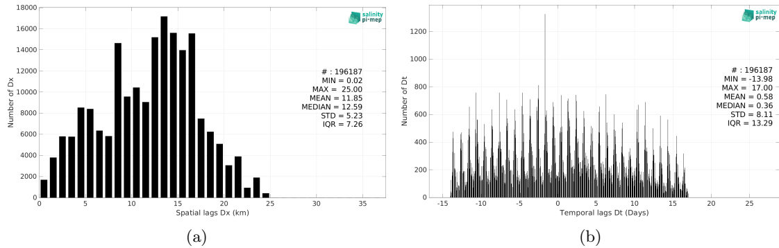
Figure 6: Histograms of the spatial (a) and temporal (b) lags between the location/time of the ICES measurement and the date of the corresponding ISAS v7 - Monthly (Ifremer-LOPS-CMEMS) SSS pixel.
