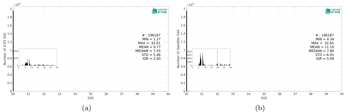
Figure 3: Histograms of SSS from ICES (a) and ISAS v7 - Monthly (Ifremer-LOPS-CMEMS) (b) considering all match-up pairs per bins of 0.1 over the Baltic Sea Pi-MEP region and for the full satellite product period.
