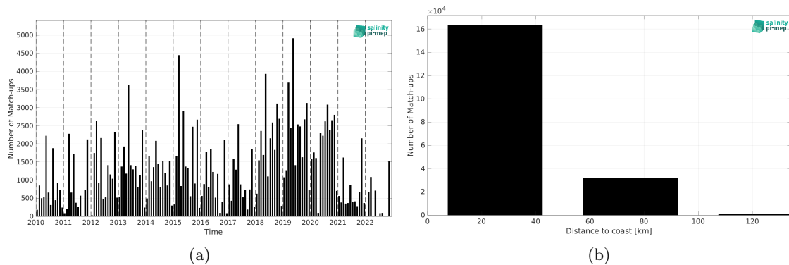
Figure 2: Number of match-ups between ICES and ISAS v7 - Monthly (Ifremer-LOPS-CMEMS) SSS as a function of time (a) and as function of the distance to coast (b) over the Baltic Sea Pi-MEP region and for the full satellite product period.
