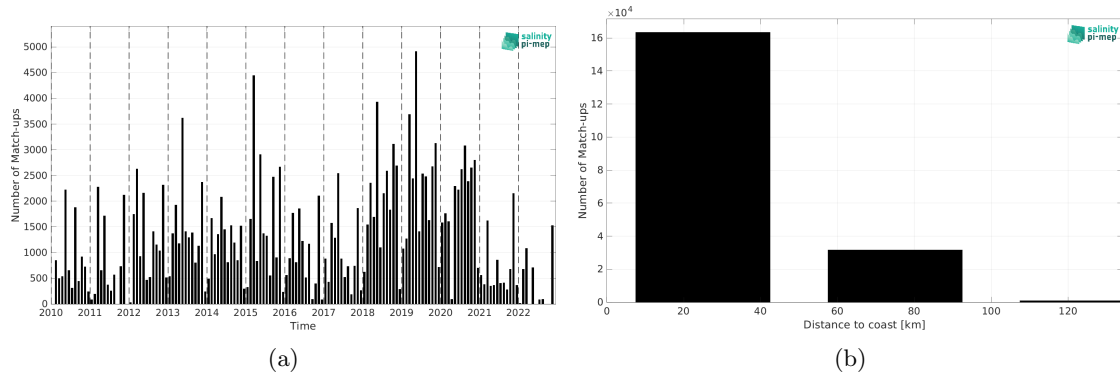
Figure 2: Number of match-ups between ICES and ISAS SSS as a function of time (a) and as function of the distance to coast (b) over the Baltic Sea Pi-MEP region and for the full satellite product period.
