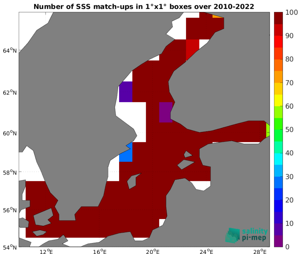
Figure 5: Number of SSS match-ups between ICES SSS and the ISAS SSS product for the Baltic Sea Pi-MEP region over 1^\circ \times 1^\circ boxes and for the full satellite product period.
