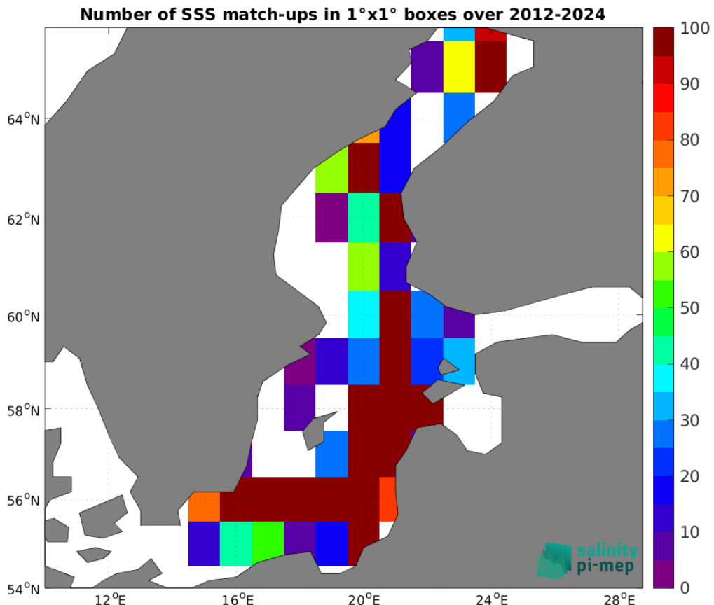
Figure 5: Number of SSS match-ups between Argo SSS and the ISAS v7 - Monthly (Ifremer-LOPS-CMEMS) SSS product for the Baltic Sea Pi-MEP region over 1^\circ \times 1^\circ boxes and for the full satellite product period.
