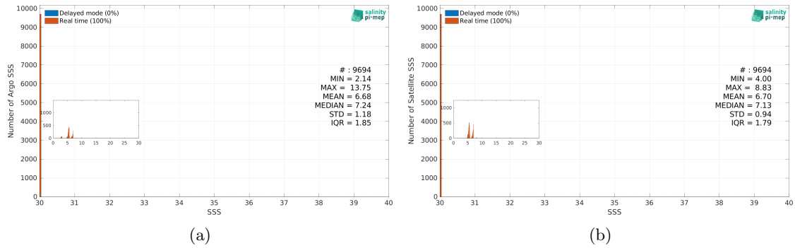
Figure 3: Histograms of SSS from Argo (a) and ISAS v7 - Monthly (Ifremer-LOPS-CMEMS) (b) considering all match-up pairs per bins of 0.1 over the Baltic Sea Pi-MEP region and for the full satellite product period.
