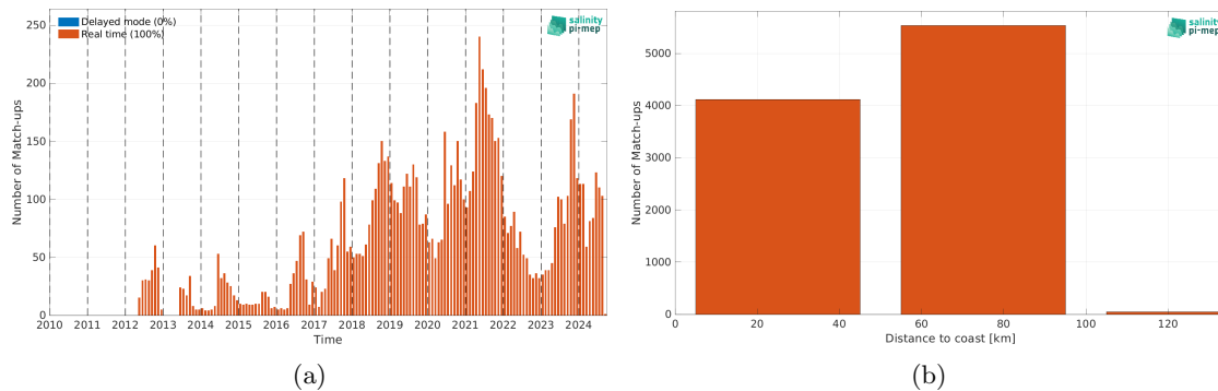
Figure 2: Number of match-ups between Argo and ISAS v7 - Monthly (Ifremer-LOPS-CMEMS) SSS as a function of time (a) and as function of the distance to coast (b) over the Baltic Sea Pi-MEP region and for the full satellite product period.
