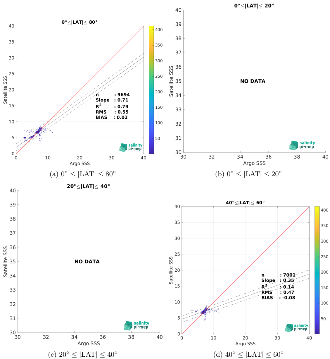
Figure 10: Contour maps of the concentration of ISAS v7 - Monthly (Ifremer-LOPS-CMEMS) SSS (y-axis) versus Argo SSS (x-axis) at match-up pairs for different latitude bands. For each plot, the red line shows x=y . The black thin and dashed lines indicate a linear fit through the data cloud and the \pm 95\% confidence levels, respectively. The number match-up pairs n , the slope and R^2 coefficient of the linear fit, the root mean square (RMS) and the mean bias between satellite and in situ data are indicated for each latitude band in each plots.
