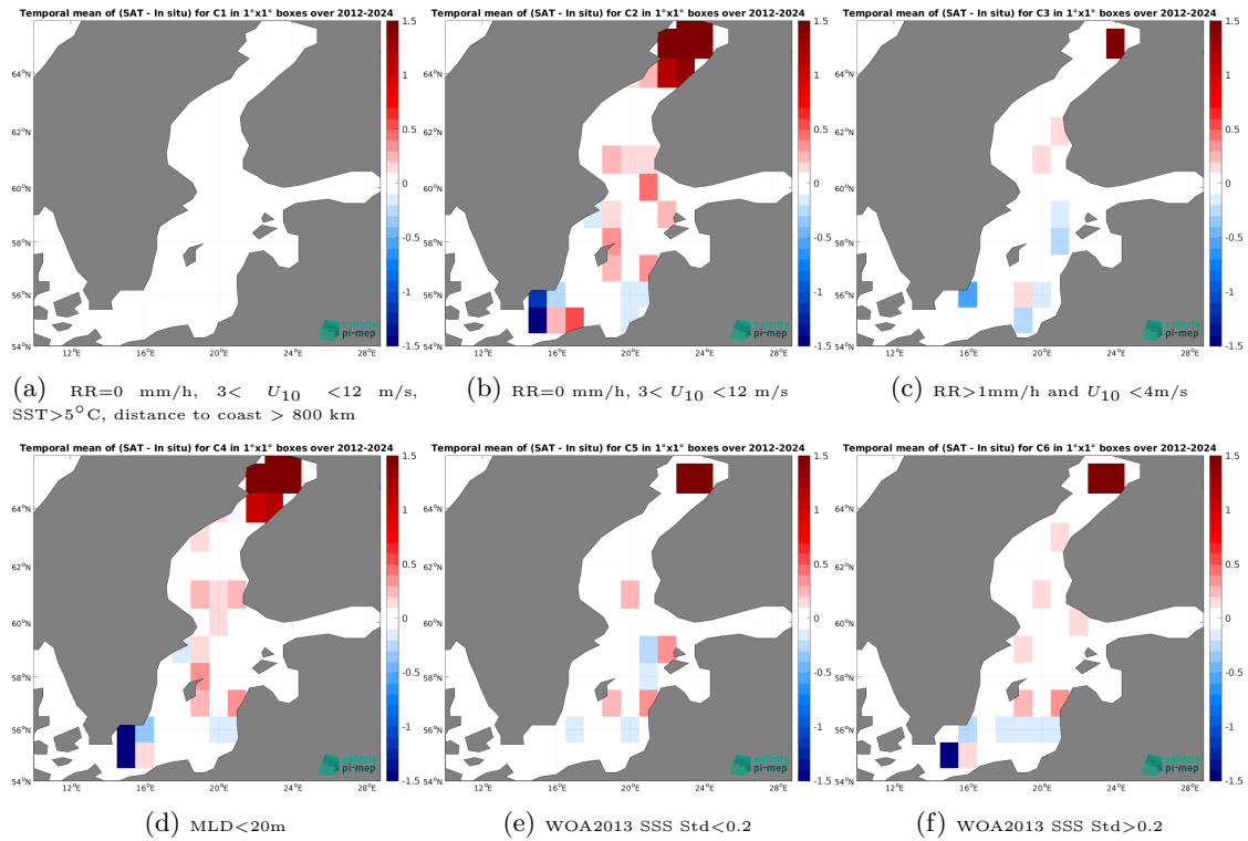
Figure 14: Temporal mean gridded over spatial boxes of size 1^\circ \times 1^\circ of \Delta\text{SSS} (ISAS v7 - Monthly (Ifremer-LOPS-CMEMS) - Argo) for 6 different subdatasets corresponding to:RR=0 mm/h, 3 < U_{10} < 12 m/s, SST>5°C, distance to coast > 800 km (a), RR=0 mm/h, 3 < U_{10} < 12 m/s (b), RR>1mm/h and U_{10} < 4 m/s (c),MLD<20m (d),WOA2013 SSS Std<0.2 (e),WOA2013 SSS Std>0.2 (f).
