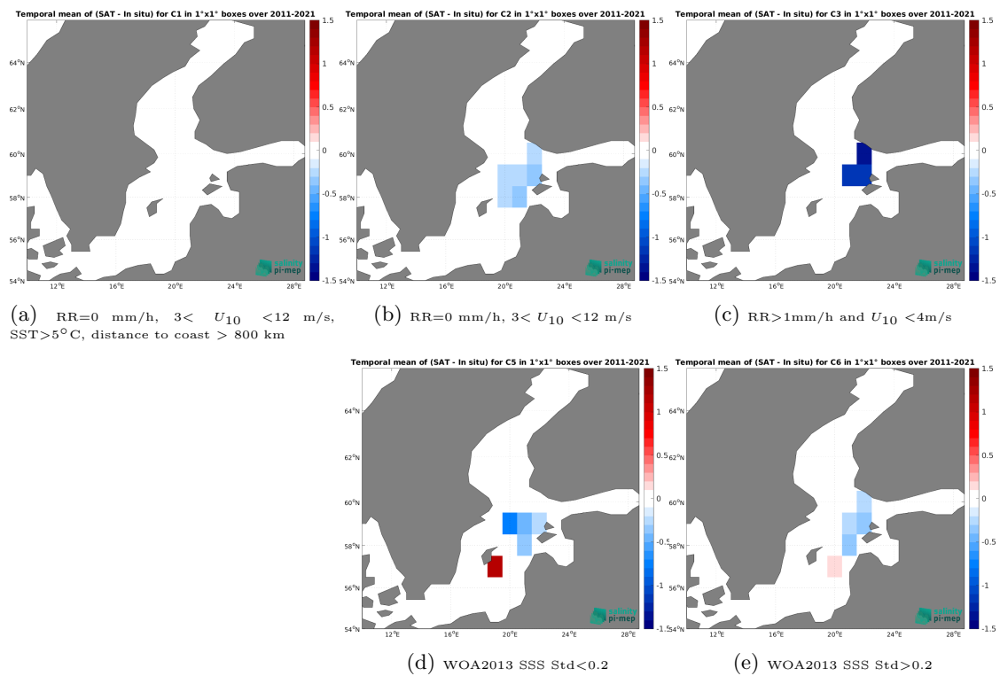
Figure 14: Temporal mean gridded over spatial boxes of size 1^\circ \times 1^\circ of \Delta SSS (CCI SSS L4 POLAR NH Merged-OI v4.41 - 7-day running (ESA) - TSG (LEGOS-DM)) for 5 different subdatasets corresponding to:RR=0 mm/h, 3 < U_{10} < 12 m/s, SST >5^\circ C, distance to coast > 800 km (a), RR=0 mm/h, 3 < U_{10} < 12 m/s (b), RR >1 mm/h and U_{10} < 4 m/s (c), WOA2013 SSS Std <0.2 (d), WOA2013 SSS Std >0.2 (e).
