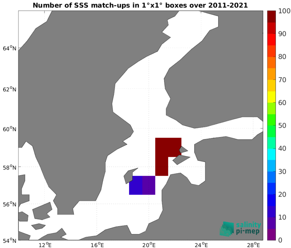
Figure 5: Number of SSS match-ups between TSG (LEGOS-DM) SSS and the CCI SSS L4 POLAR NH Merged-OI v4.41 - 7-day running (ESA) SSS product for the Baltic Sea Pi-MEP region over 1^\circ \times 1^\circ boxes and for the full satellite product period.
