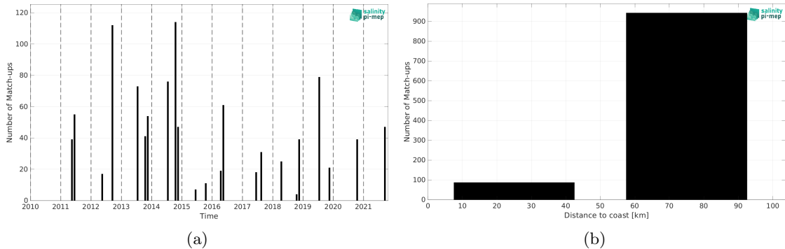
Figure 2: Number of match-ups between TSG (LEGOS-DM) and CCI SSS L4 POLAR NH Merged-OI v4.41 - 7-day running (ESA) SSS as a function of time (a) and as function of the distance to coast (b) over the Baltic Sea Pi-MEP region and for the full satellite product period.
