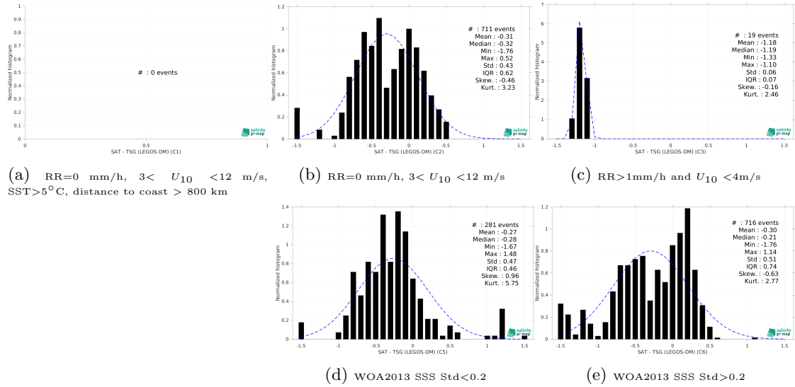
Figure 15: Normalized histogram of \Delta\text{SSS} (CCI SSS L4 POLAR NH Merged-OI v4.41 - 7-day running (ESA) - TSG (LEGOS-DM)) for 5 different subdatasets corresponding to: RR=0 mm/h, 3 < U_{10} < 12 m/s, SST > 5^{\circ}\text{C} , distance to coast > 800 km (a), RR=0 mm/h, 3 < U_{10} < 12 m/s (b), RR > 1\text{mm/h} and U_{10} < 4\text{m/s} (c), WOA2013 SSS Std < 0.2 (d), WOA2013 SSS Std > 0.2 (e).
