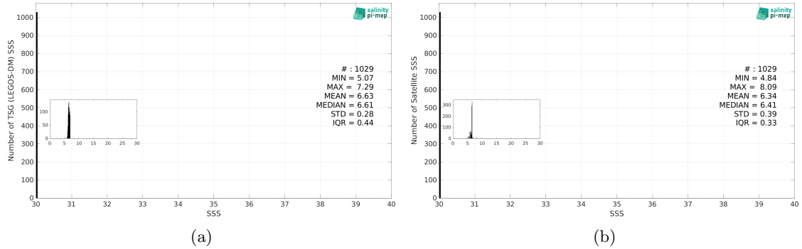
Figure 3: Histograms of SSS from TSG (LEGOS-DM) (a) and CCI SSS L4 POLAR NH Merged-OI v4.41 - 7-day running (ESA) (b) considering all match-up pairs per bins of 0.1 over the Baltic Sea Pi-MEP region and for the full satellite product period.
