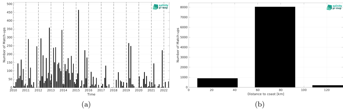
Figure 2: Number of match-ups between ICES and CCI SSS L4 POLAR NH Merged-OI v4.41 - 7-day running (ESA) SSS as a function of time (a) and as function of the distance to coast (b) over the Baltic Sea Pi-MEP region and for the full satellite product period.
