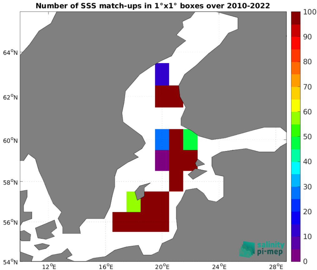
Figure 5: Number of SSS match-ups between ICES SSS and the CCI SSS L4 POLAR NH Merged-OI v4.41 - 7-day running (ESA) SSS product for the Baltic Sea Pi-MEP region over 1^\circ \times 1^\circ boxes and for the full satellite product period.
