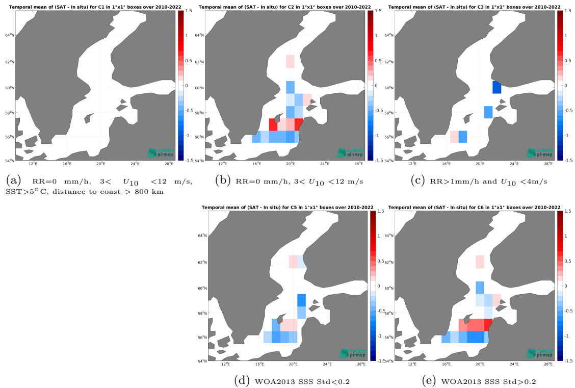
Figure 14: Temporal mean gridded over spatial boxes of size 1^\circ \times 1^\circ of \Delta SSS (CCI SSS L4 POLAR NH Merged-OI v4.41 - 7-day running (ESA) - ICES) for 5 different subdatasets corresponding to: RR=0 mm/h, 3 < U_{10} < 12 m/s, SST >5^\circ\text{C} , distance to coast > 800 km (a), RR=0 mm/h, 3 < U_{10} < 12 m/s (b), RR >1 mm/h and U_{10} < 4 m/s (c), WOA2013 SSS Std <0.2 (d), WOA2013 SSS Std >0.2 (e).
