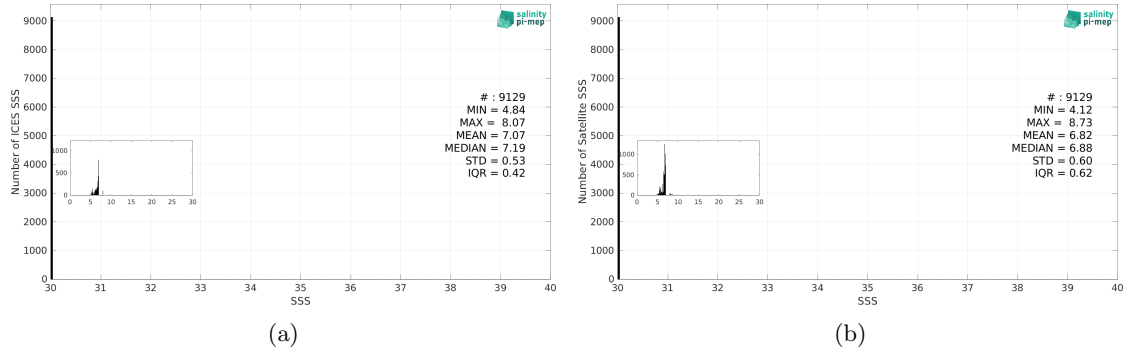
Figure 3: Histograms of SSS from ICES (a) and CCI SSS L4 POLAR NH Merged-OI v4.41 - 7-day running (ESA) (b) considering all match-up pairs per bins of 0.1 over the Baltic Sea Pi-MEP region and for the full satellite product period.
