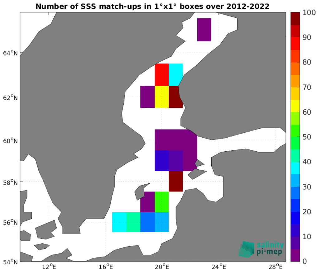
Figure 5: Number of SSS match-ups between Argo SSS and the CCI SSS L4 POLAR NH Merged-OI v4.41 - 7-day running (ESA) SSS product for the Baltic Sea Pi-MEP region over 1°×1° boxes and for the full satellite product period.
