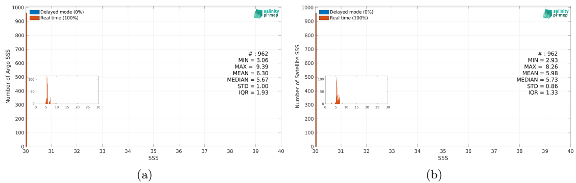
Figure 3: Histograms of SSS from Argo (a) and CCI SSS L4 POLAR NH Merged-OI v4.41 - 7-day running (ESA) (b) considering all match-up pairs per bins of 0.1 over the Baltic Sea Pi-MEP region and for the full satellite product period.
