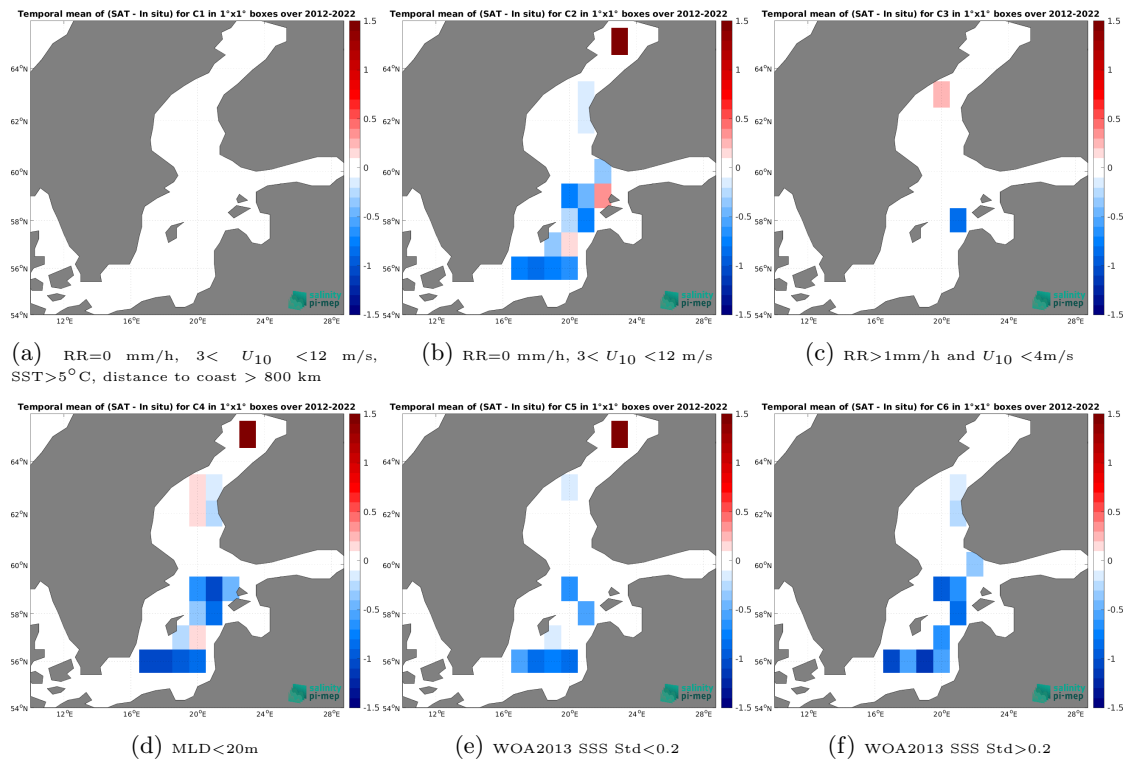
Figure 14: Temporal mean gridded over spatial boxes of size 1^\circ \times 1^\circ of \Delta SSS (CCI SSS L4 POLAR NH Merged-OI v4.41 - 7-day running (ESA) - Argo) for 6 different subdatasets corresponding to:RR=0 mm/h, 3 < U_{10} < 12 m/s, SST>5°C, distance to coast > 800 km (a), RR=0 mm/h, 3 < U_{10} < 12 m/s (b), RR>1mm/h and U_{10} < 4 m/s (c),MLD<20m (d),WOA2013 SSS Std<0.2 (e),WOA2013 SSS Std>0.2 (f).
