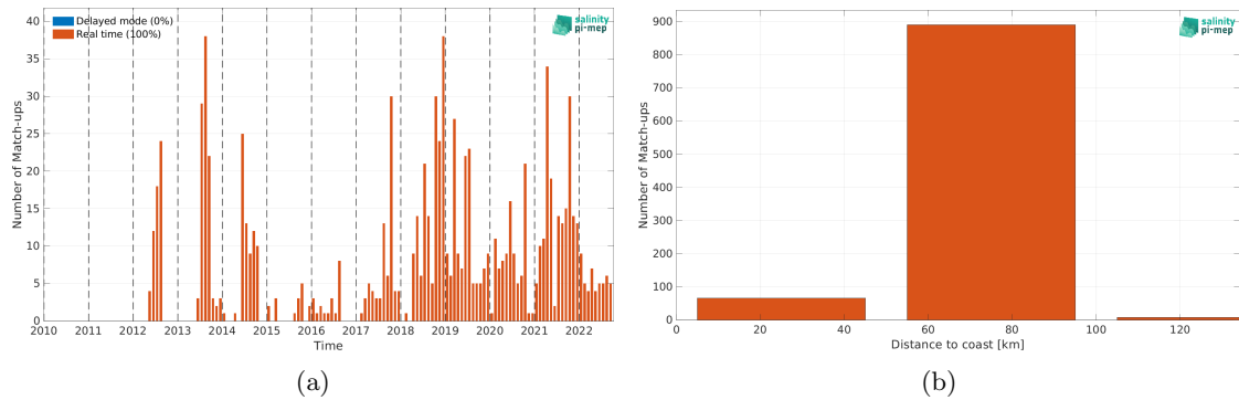
Figure 2: Number of match-ups between Argo and CCI SSS L4 POLAR NH Merged-OI v4.41 - 7-day running (ESA) SSS as a function of time (a) and as function of the distance to coast (b) over the Baltic Sea Pi-MEP region and for the full satellite product period.
