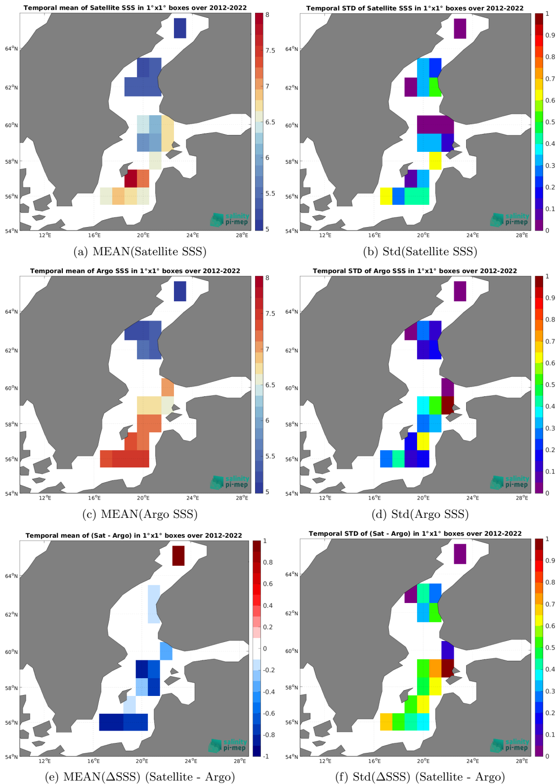
Figure 7: Temporal mean (left) and Std (right) of SSS from CCI SSS L4 POLAR NH Merged-OI v4.41 - 7-day running (ESA) (top), Argo (middle), and of \Delta SSS (Satellite - Argo). Only match-up pairs are used to generate these maps.
