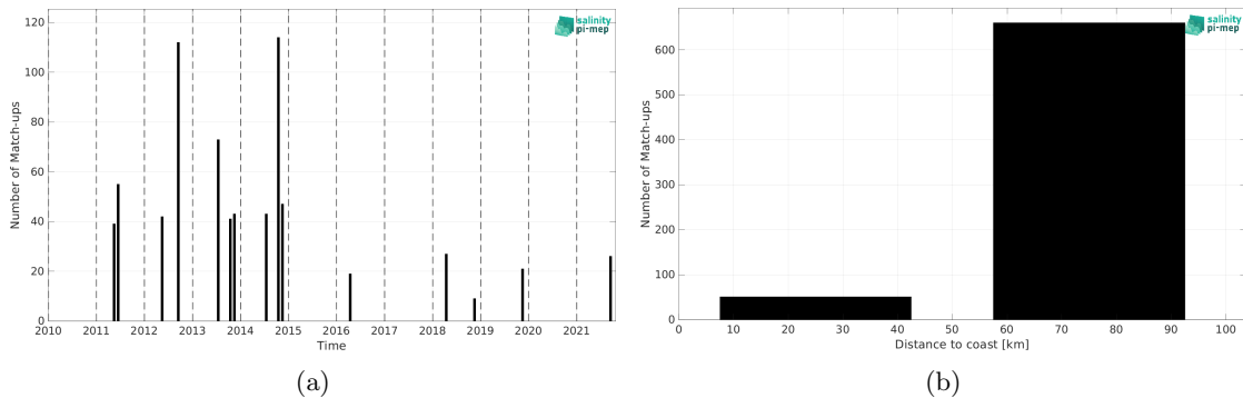
Figure 2: Number of match-ups between TSG (LEGOS-DM) and CCI SSS L4 POLAR NH Merged-OI v4.41 - 30-day running (ESA) SSS as a function of time (a) and as function of the distance to coast (b) over the Baltic Sea Pi-MEP region and for the full satellite product period.
