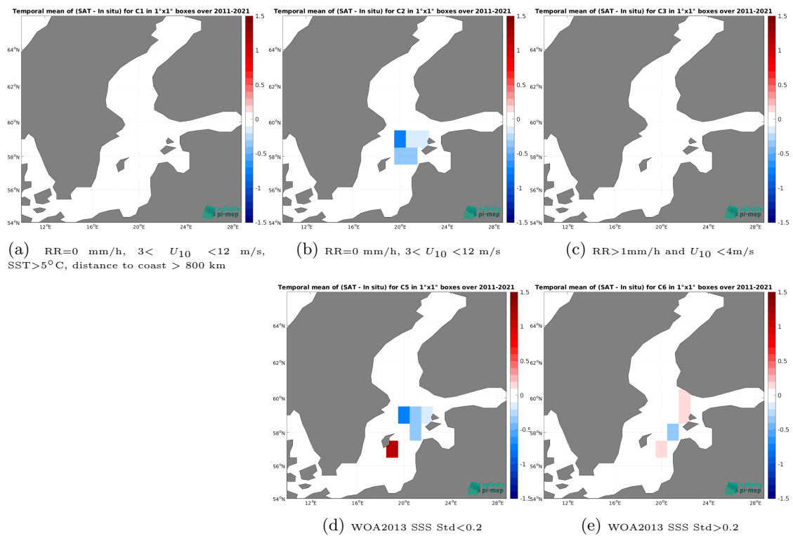
Figure 14: Temporal mean gridded over spatial boxes of size 1^\circ \times 1^\circ of \Delta SSS (CCI SSS L4 POLAR NH Merged-OI v4.41 - 30-day running (ESA) - TSG (LEGOS-DM)) for 5 different subdatasets corresponding to:RR=0 mm/h, 3 < U_{10} < 12 m/s, SST >5^\circ\text{C} , distance to coast > 800 km (a), RR=0 mm/h, 3 < U_{10} < 12 m/s (b), RR >1 mm/h and U_{10} < 4 m/s (c), WOA2013 SSS Std <0.2 (d), WOA2013 SSS Std >0.2 (e).
