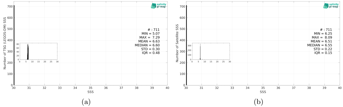
Figure 3: Histograms of SSS from TSG (LEGOS-DM) (a) and CCI SSS L4 POLAR NH Merged-OI v4.41 - 30-day running (ESA) (b) considering all match-up pairs per bins of 0.1 over the Baltic Sea Pi-MEP region and for the full satellite product period.
