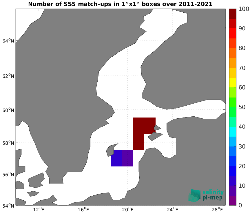
Figure 5: Number of SSS match-ups between TSG (LEGOS-DM) SSS and the CCI SSS L4 POLAR NH Merged-OI v4.41 - 30-day running (ESA) SSS product for the Baltic Sea Pi-MEP region over 1^\circ \times 1^\circ boxes and for the full satellite product period.
