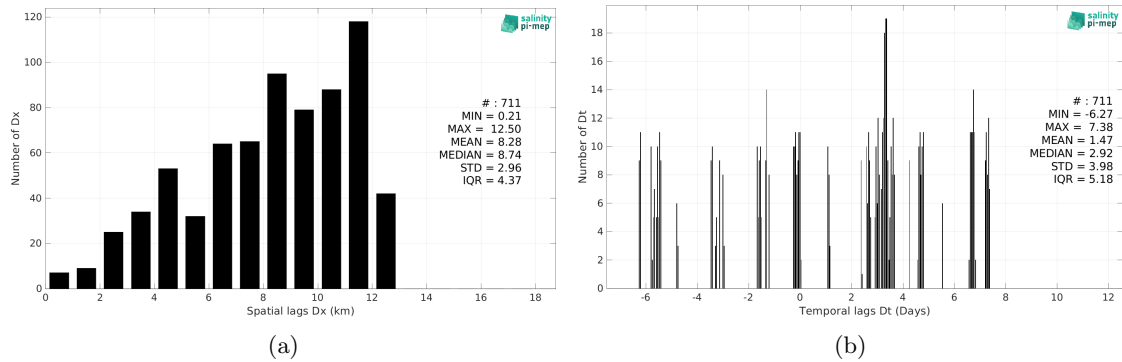
Figure 6: Histograms of the spatial (a) and temporal (b) lags between the location/time of the TSG (LEGOS-DM) measurement and the date of the corresponding CCI SSS L4 POLAR NH Merged-OI v4.41 - 30-day running (ESA) SSS pixel.
