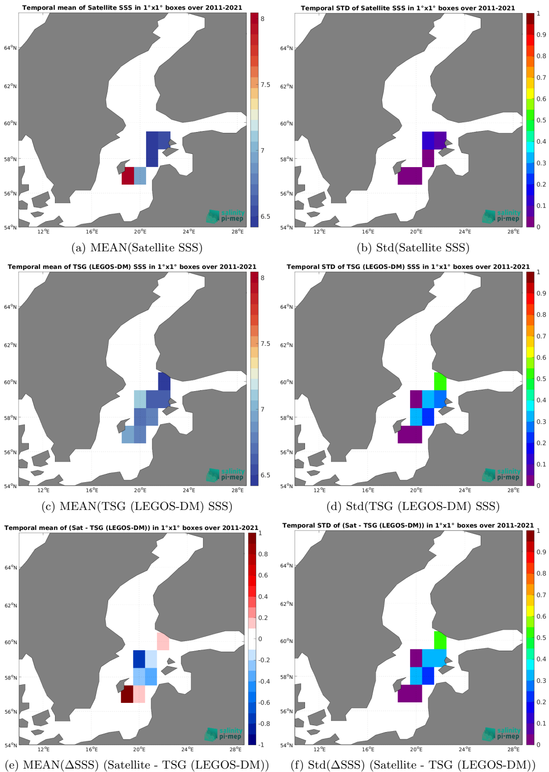
(e) MEAN( \Delta SSS) (Satellite - TSG (LEGOS-DM)) (f) Std( \Delta SSS) (Satellite - TSG (LEGOS-DM)) Figure 7: Temporal mean (left) and Std (right) of SSS from CCI SSS L4 POLAR NH Merged-OI v4.41 - 30-day running (ESA) (top), TSG (LEGOS-DM) (middle), and of \Delta SSS (Satellite - TSG (LEGOS-DM)). Only match-up pairs are used to generate these maps.
