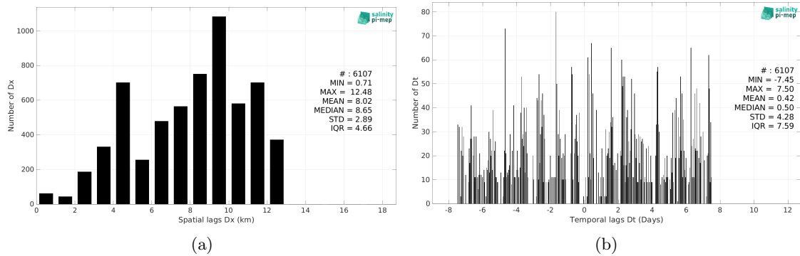
Figure 6: Histograms of the spatial (a) and temporal (b) lags between the location/time of the ICES measurement and the date of the corresponding CCI SSS L4 POLAR NH Merged-OI v4.41 - 30-day running (ESA) SSS pixel.
