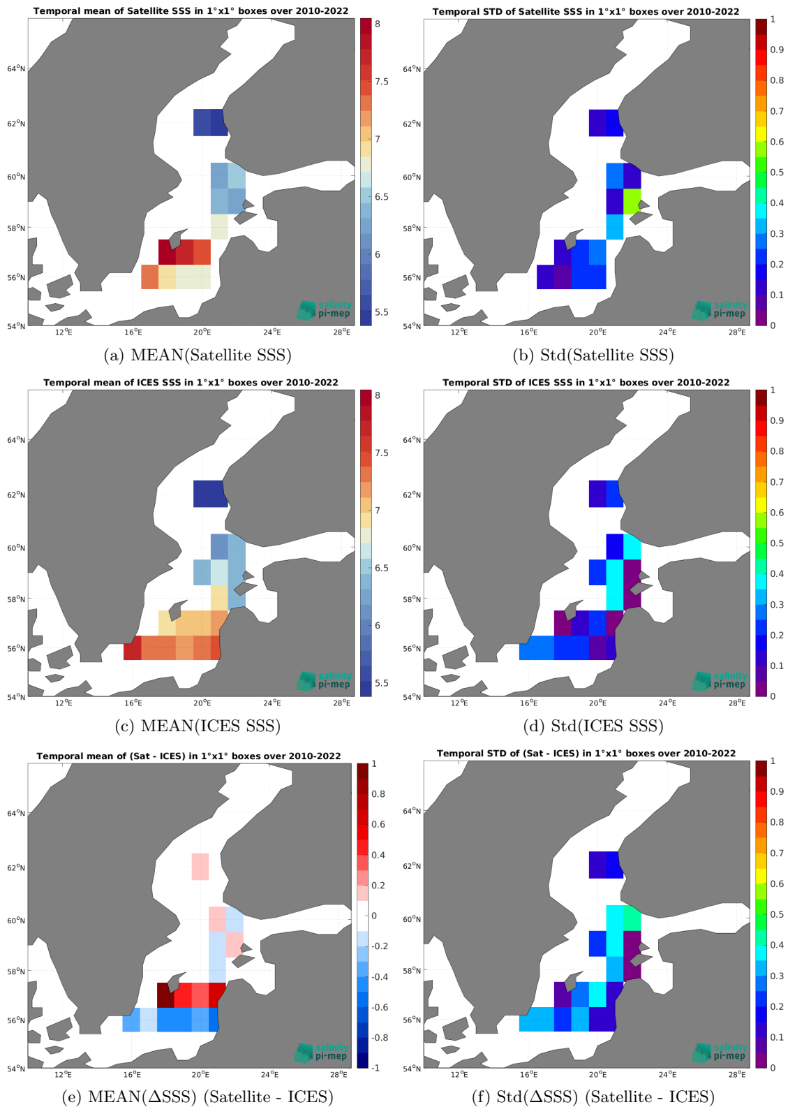
Figure 7: Temporal mean (left) and Std (right) of SSS from CCI SSS L4 POLAR NH Merged-OI v4.41 - 30-day running (ESA) (top), ICES 16 (middle), and of \Delta SSS (Satellite - ICES). Only match-up pairs are used to generate these maps.
