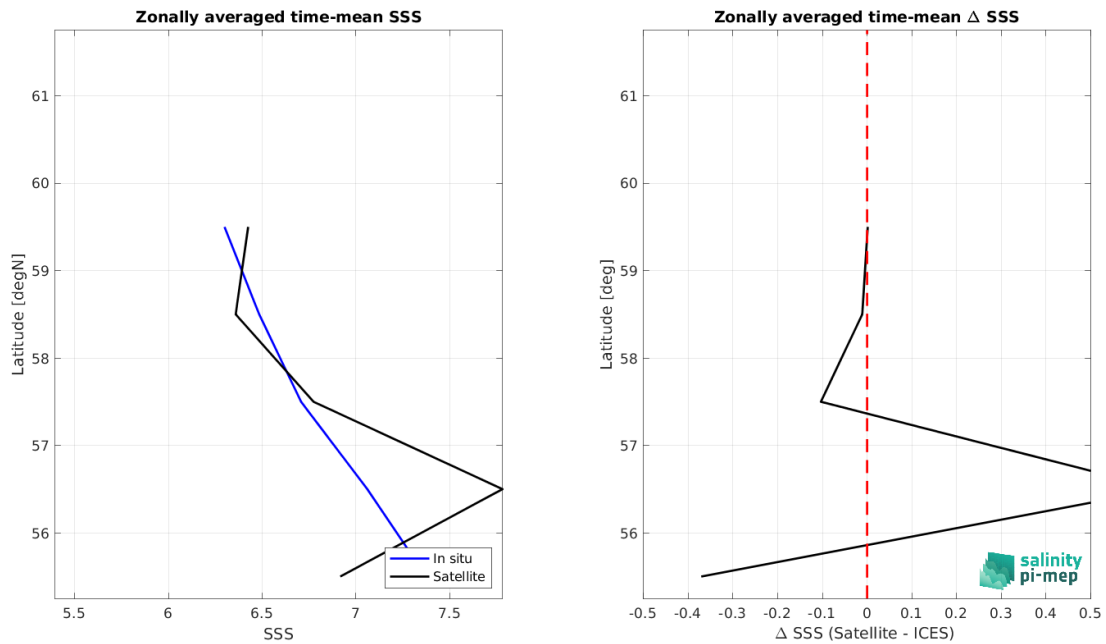
Figure 9: Left panel: Zonal mean SSS from CCI SSS L4 POLAR NH Merged-OI v4.41 - 30-day running (ESA) satellite product (black) and from ICES (blue). Right panel: Zonal mean of \Delta SSS (Satellite - ICES) for all the collected Pi-MEP match-up pairs estimated over the full satellite product period.
