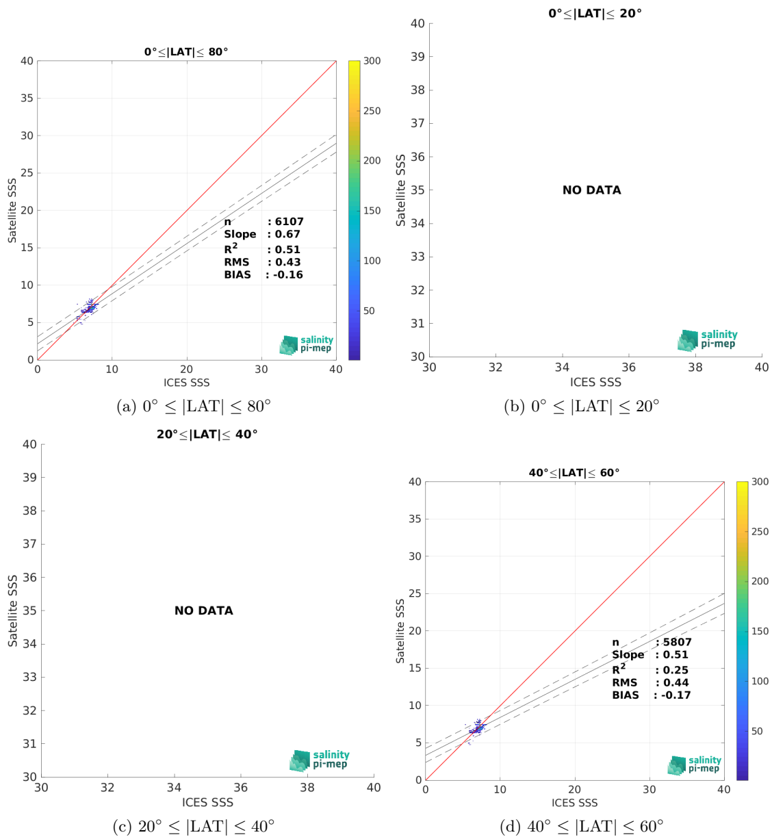
Figure 10: Contour maps of the concentration of CCI SSS L4 POLAR NH Merged-OI v4.41 - 30-day running (ESA) SSS (y-axis) versus ICES SSS (x-axis) at match-up pairs for different latitude bands. For each plot, the red line shows x=y . The black thin and dashed lines indicate a linear fit through the data cloud and the \pm 95\% confidence levels, respectively. The number match-up pairs n , the slope and R^2 coefficient of the linear fit, the root mean square (RMS) and the mean bias between satellite and in situ data are indicated for each latitude band in each plots.
