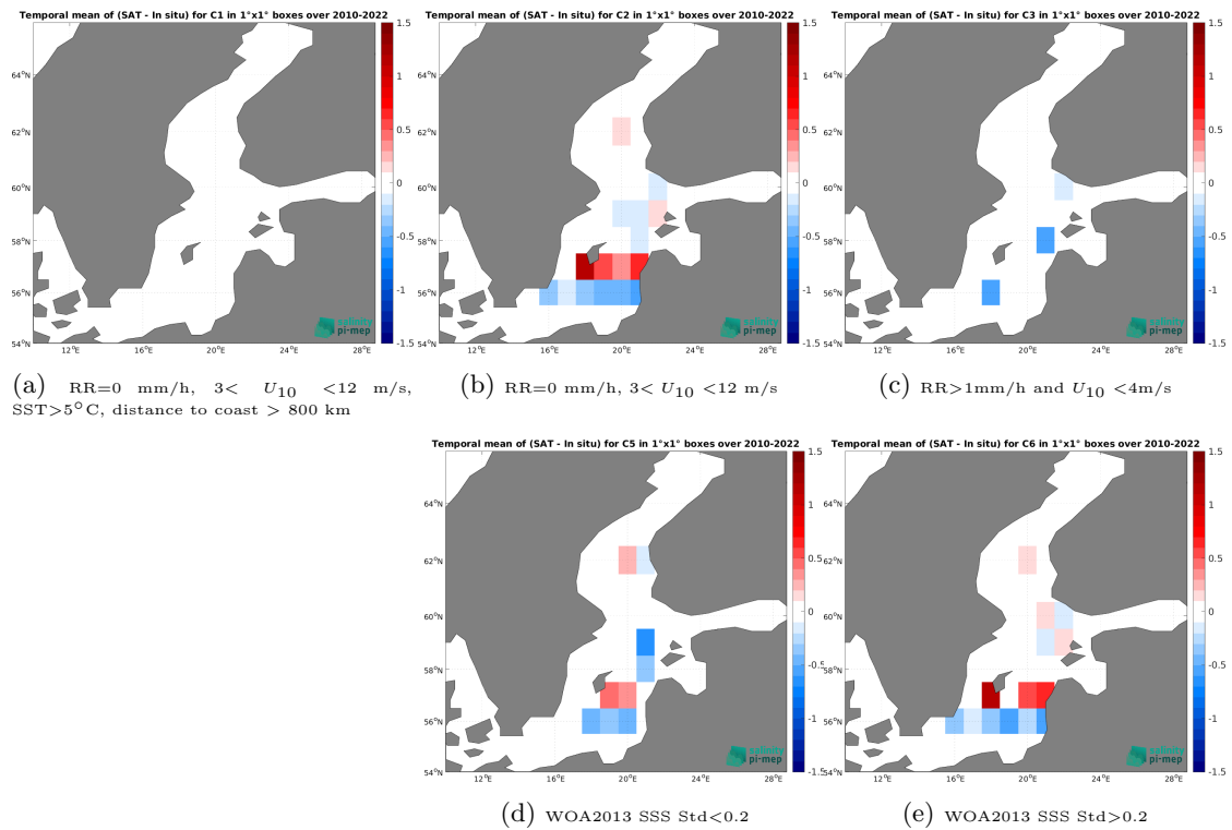
Figure 14: Temporal mean gridded over spatial boxes of size 1^\circ \times 1^\circ of \Delta SSS (CCI SSS L4 POLAR NH Merged-OI v4.41 - 30-day running (ESA) - ICES) for 5 different subdatasets corresponding to: RR=0 mm/h, 3 < U_{10} < 12 m/s, SST > 5^\circ\text{C} , distance to coast > 800 km (a), RR=0 mm/h, 3 < U_{10} < 12 m/s (b), RR > 1\text{mm/h} and U_{10} < 4\text{m/s} (c), WOA2013 SSS Std < 0.2 (d), WOA2013 SSS Std > 0.2 (e).
