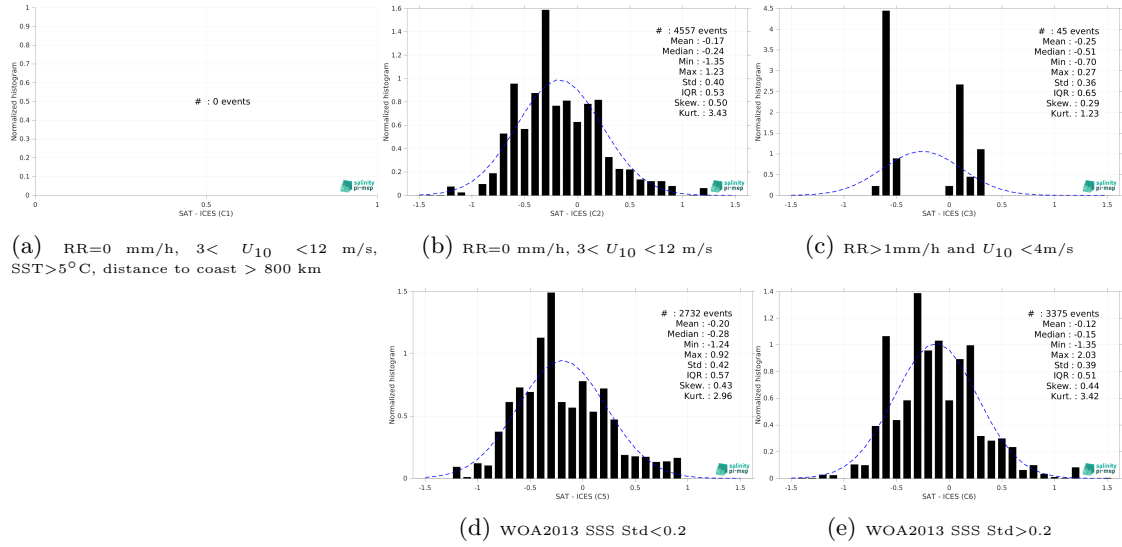
Figure 15: Normalized histogram of \Delta SSS (CCI SSS L4 POLAR NH Merged-OI v4.41 - 30-day running (ESA) - ICES) for 5 different subdatasets corresponding to: RR=0 mm/h, 3 < U_{10} < 12 m/s, SST > 5°C, distance to coast > 800 km (a), RR=0 mm/h, 3 < U_{10} < 12 m/s (b), RR > 1mm/h and U_{10} < 4 m/s (c), WOA2013 SSS Std < 0.2 (d), WOA2013 SSS Std > 0.2 (e).
