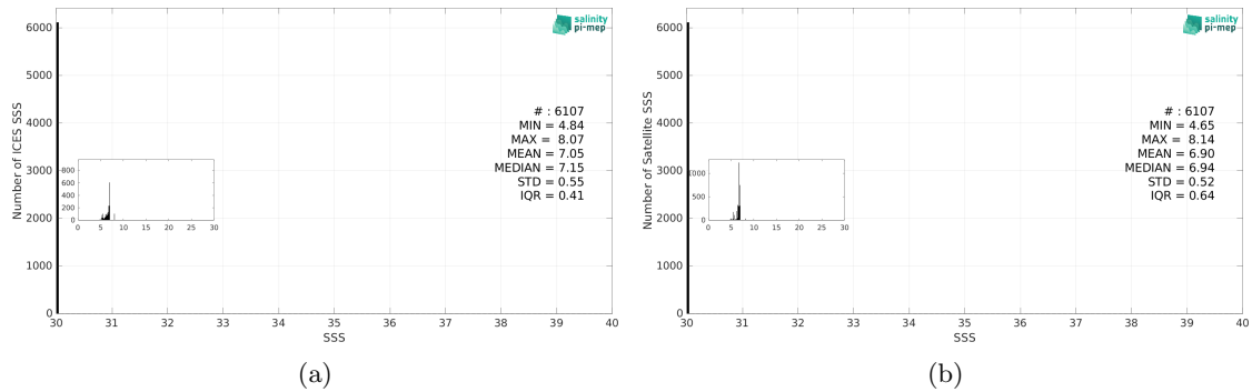
Figure 3: Histograms of SSS from ICES (a) and CCI SSS L4 POLAR NH Merged-OI v4.41 - 30-day running (ESA) (b) considering all match-up pairs per bins of 0.1 over the Baltic Sea Pi-MEP region and for the full satellite product period.
