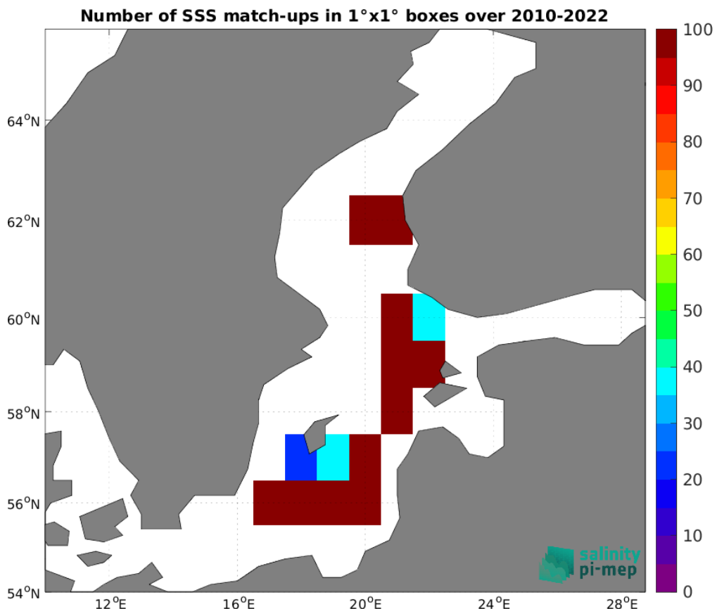
Figure 5: Number of SSS match-ups between ICES SSS and the CCI SSS L4 POLAR NH Merged-OI v4.41 - 30-day running (ESA) SSS product for the Baltic Sea Pi-MEP region over 1°x1° boxes and for the full satellite product period.
