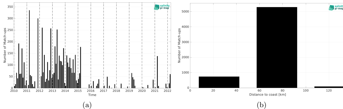
Figure 2: Number of match-ups between ICES and CCI SSS L4 POLAR NH Merged-OI v4.41 - 30-day running (ESA) SSS as a function of time (a) and as function of the distance to coast (b) over the Baltic Sea Pi-MEP region and for the full satellite product period.
