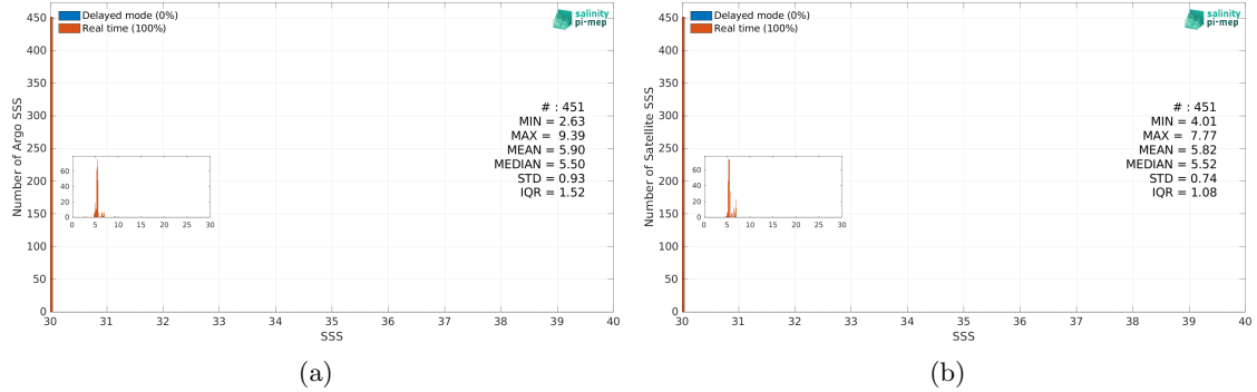
Figure 3: Histograms of SSS from Argo (a) and CCI SSS L4 POLAR NH Merged-OI v4.41 - 30-day running (ESA) (b) considering all match-up pairs per bins of 0.1 over the Baltic Sea Pi-MEP region and for the full satellite product period.
