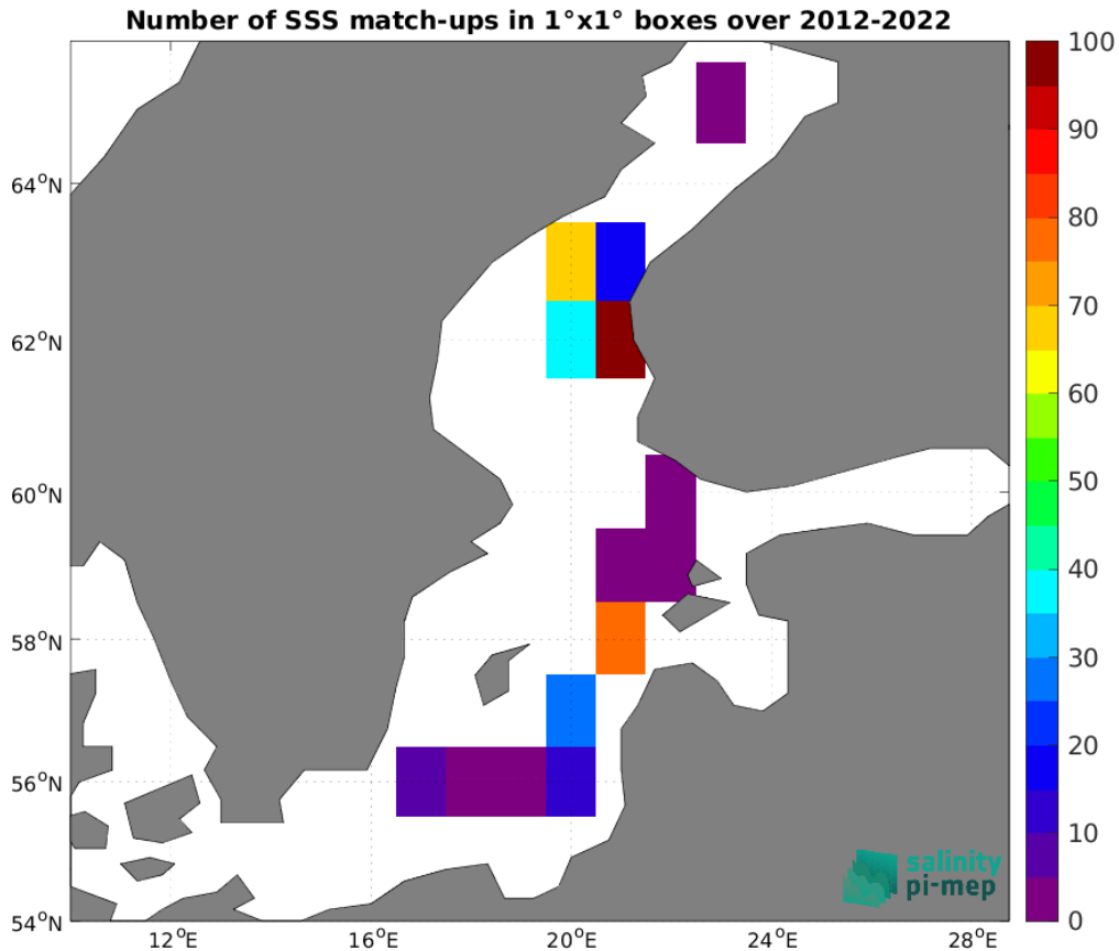
Figure 5: Number of SSS match-ups between Argo SSS and the CCI SSS L4 POLAR NH Merged-OI v4.41 - 30-day running (ESA) SSS product for the Baltic Sea Pi-MEP region over 1^\circ \times 1^\circ boxes and for the full satellite product period.
