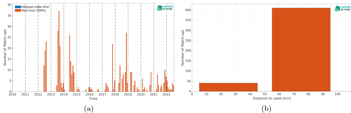
Figure 2: Number of match-ups between Argo and CCI SSS L4 POLAR NH Merged-OI v4.41 - 30-day running (ESA) SSS as a function of time (a) and as function of the distance to coast (b) over the Baltic Sea Pi-MEP region and for the full satellite product period.
