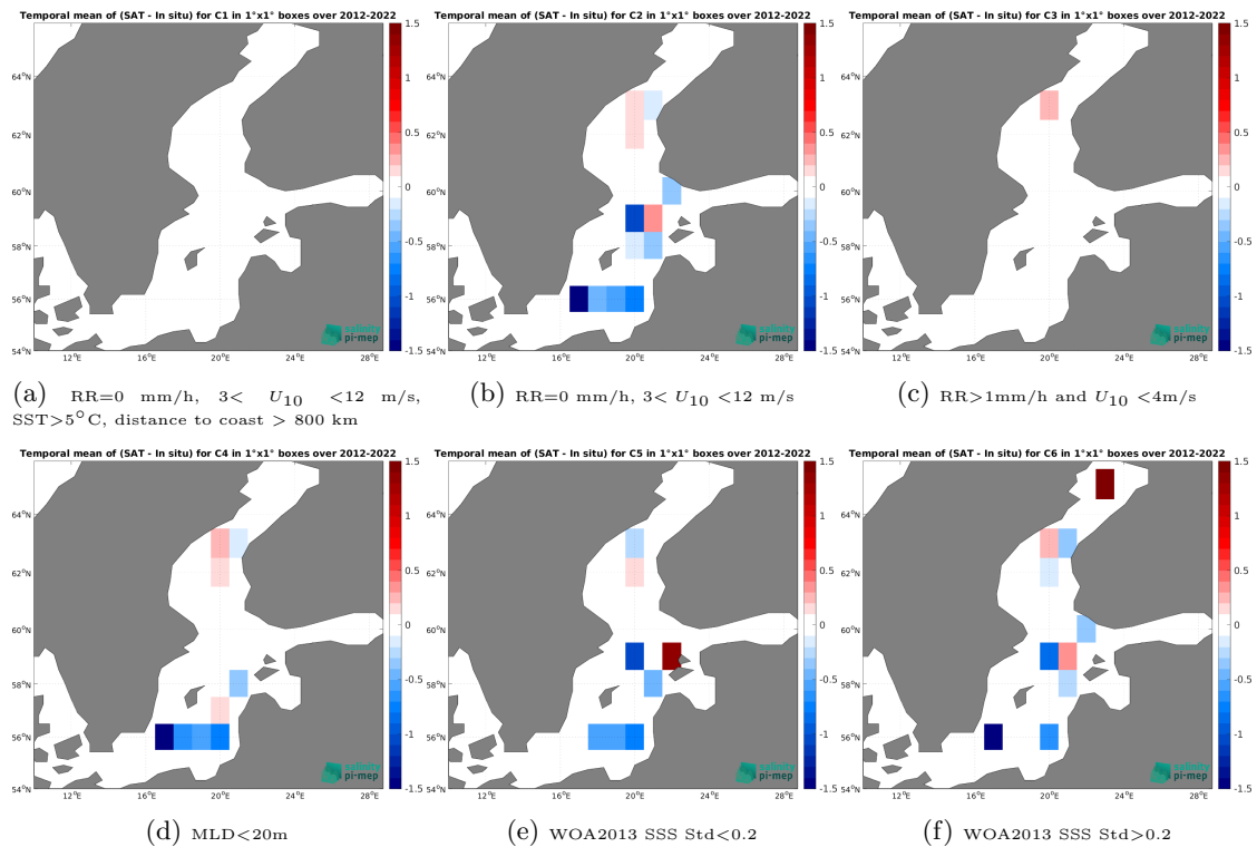
Figure 14: Temporal mean gridded over spatial boxes of size 1^\circ \times 1^\circ of \Delta SSS (CCI SSS L4 POLAR NH Merged-OI v4.41 - 30-day running (ESA) - Argo) for 6 different subdatasets corresponding to:RR=0 mm/h, 3 < U_{10} < 12 m/s, SST >5^\circ C, distance to coast > 800 km (a), RR=0 mm/h, 3 < U_{10} < 12 m/s (b), RR >1 mm/h and U_{10} < 4 m/s (c),MLD <20 m (d),WOA2013 SSS Std <0.2 (e),WOA2013 SSS Std >0.2 (f).
