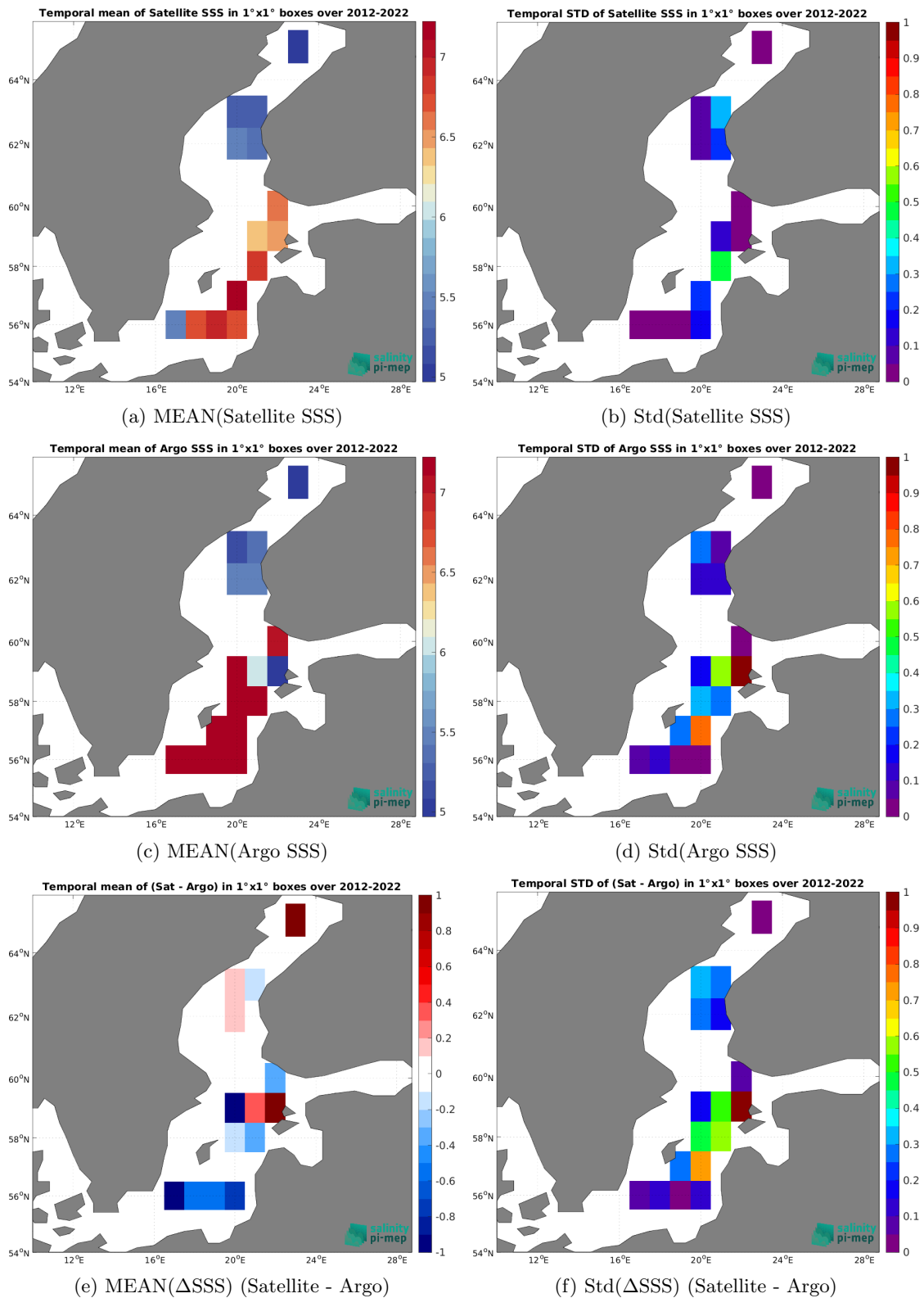
Figure 7: Temporal mean (left) and Std (right) of SSS from CCI SSS L4 POLAR NH Merged-OI v4.41 - 30-day running (ESA) (top), Argo (middle), and of \Delta SSS (Satellite - Argo). Only match-up pairs are used to generate these maps.
