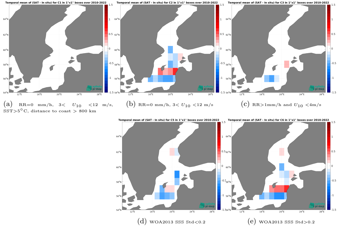
Figure 12: Temporal mean gridded over spatial boxes of size 1^{\circ}\times 1^{\circ} of \Delta\text{SSS} (CCI SSS L4 POLAR NH Merged-OI v4.4 - 7-day running (ESA) - ICES) for 5 different subdatasets corresponding to:RR=0 mm/h, 3 < U_{10} < 12 m/s, SST >5^{\circ}\text{C} , distance to coast > 800 km (a), RR=0 mm/h, 3 < U_{10} < 12 m/s (b), RR >1 mm/h and U_{10} < 4 m/s (c), WOA2013 SSS Std <0.2 (d), WOA2013 SSS Std >0.2 (e).
