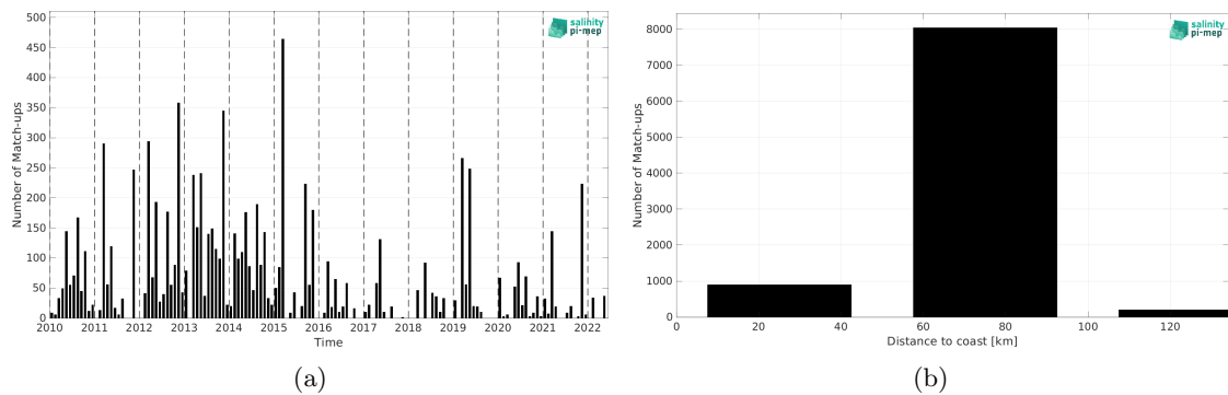
Figure 1: Number of match-ups between ICES and CCI SSS L4 POLAR NH Merged-OI v4.4 - 7-day running (ESA) SSS as a function of time (a) and as function of the distance to coast (b) over the Baltic Sea Pi-MEP region and for the full satellite product period.
