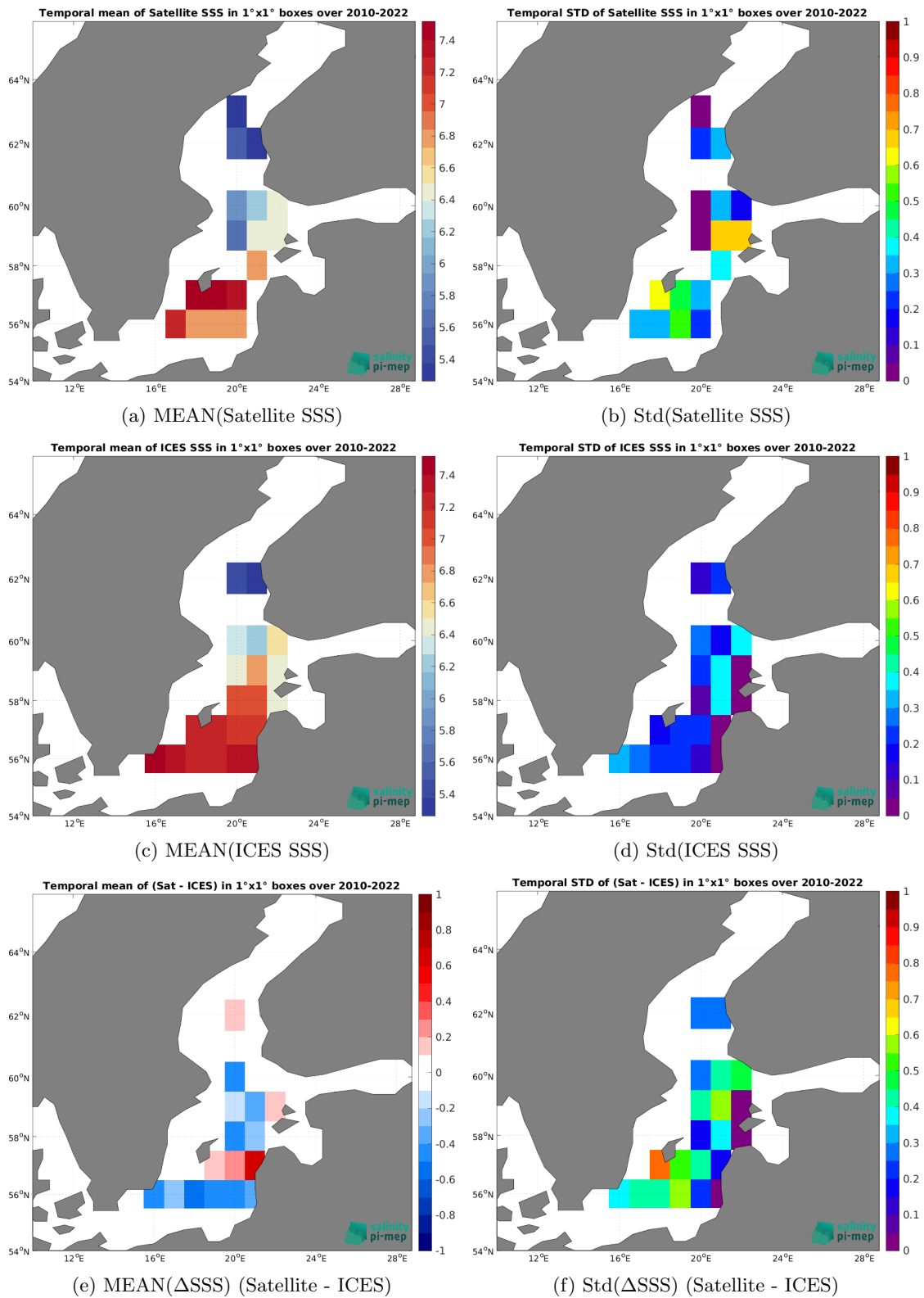
Figure 6: Temporal mean (left) and Std (right) of SSS from CCI SSS L4 POLAR NH Merged-OI v4.4 - 7-day running (ESA) (top), ICES (middle), and of \Delta SSS (Satellite - ICES). Only match-up pairs are used to generate these maps.
