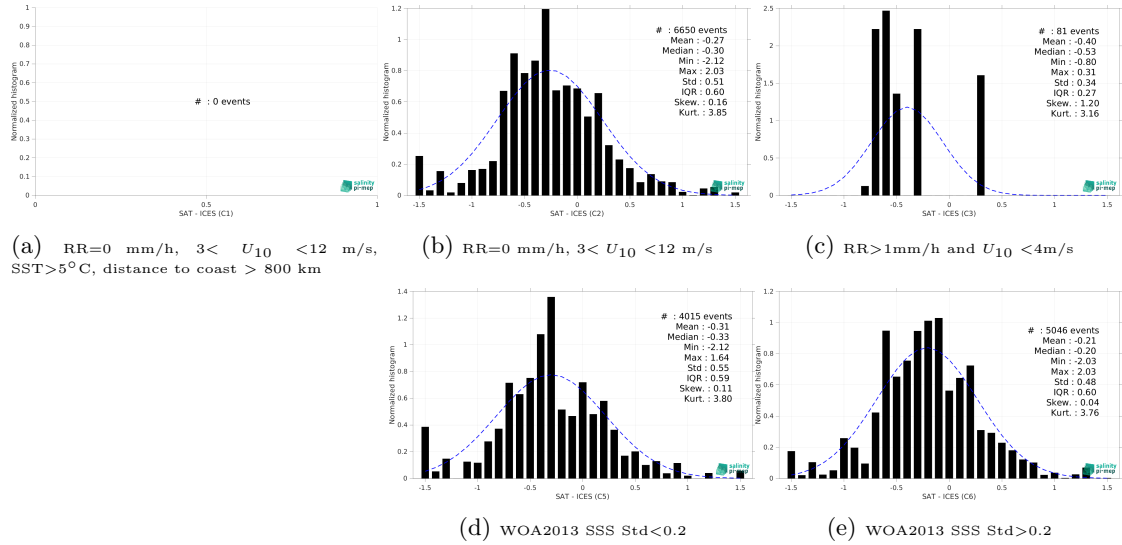
Figure 13: Normalized histogram of \Delta SSS (CCI SSS L4 POLAR NH Merged-OI v4.4 - 7-day running (ESA) - ICES) for 5 different subdatasets corresponding to: RR=0 mm/h, 3 < U_{10} < 12 m/s, SST > 5°C, distance to coast > 800 km (a), RR=0 mm/h, 3 < U_{10} < 12 m/s (b), RR > 1mm/h and U_{10} < 4 m/s (c), WOA2013 SSS Std < 0.2 (d), WOA2013 SSS Std > 0.2 (e).
