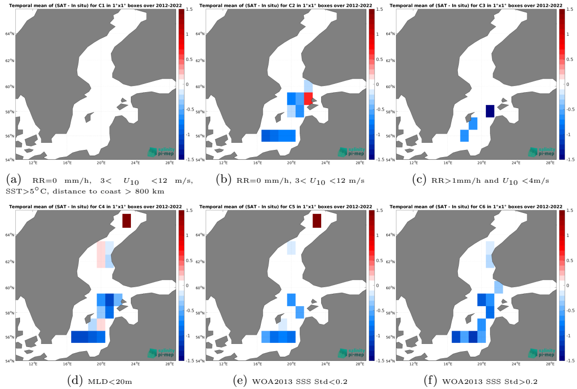
Figure 12: Temporal mean gridded over spatial boxes of size 1^{\circ}\times 1^{\circ} of \Delta\text{SSS} (CCI SSS L4 POLAR NH Merged-OI v4.4 - 7-day running (ESA) - Argo) for 6 different subdatasets corresponding to:RR=0 mm/h, 3 < U_{10} < 12 m/s, SST >5^{\circ}\text{C} , distance to coast > 800 km (a), RR=0 mm/h, 3 < U_{10} < 12 m/s (b), RR >1\text{mm/h} and U_{10} < 4\text{m/s} (c),MLD <20\text{m} (d),WOA2013 SSS Std <0.2 (e),WOA2013 SSS Std >0.2 (f).
