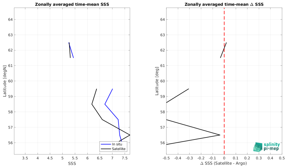
Figure 8: Left panel: Zonal mean SSS from CCI SSS L4 POLAR NH Merged-OI v4.4 - 7-day running (ESA) satellite product (black) and from Argo (blue). Right panel: Zonal mean of \Delta SSS (Satellite - Argo) for all the collected Pi-MEP match-up pairs estimated over the full satellite product period.
