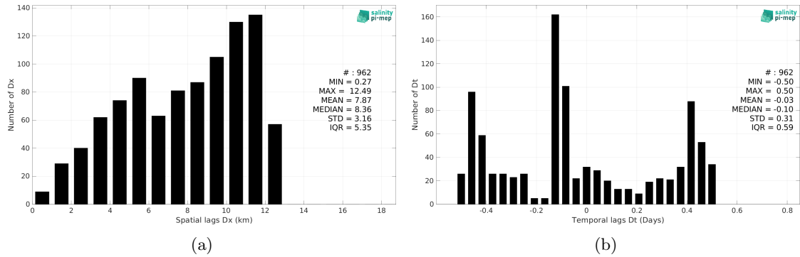
Figure 5: Histograms of the spatial (a) and temporal (b) lags between the location/time of the Argo measurement and the date of the corresponding CCI SSS L4 POLAR NH Merged-OI v4.4 - 7-day running (ESA) SSS pixel.
