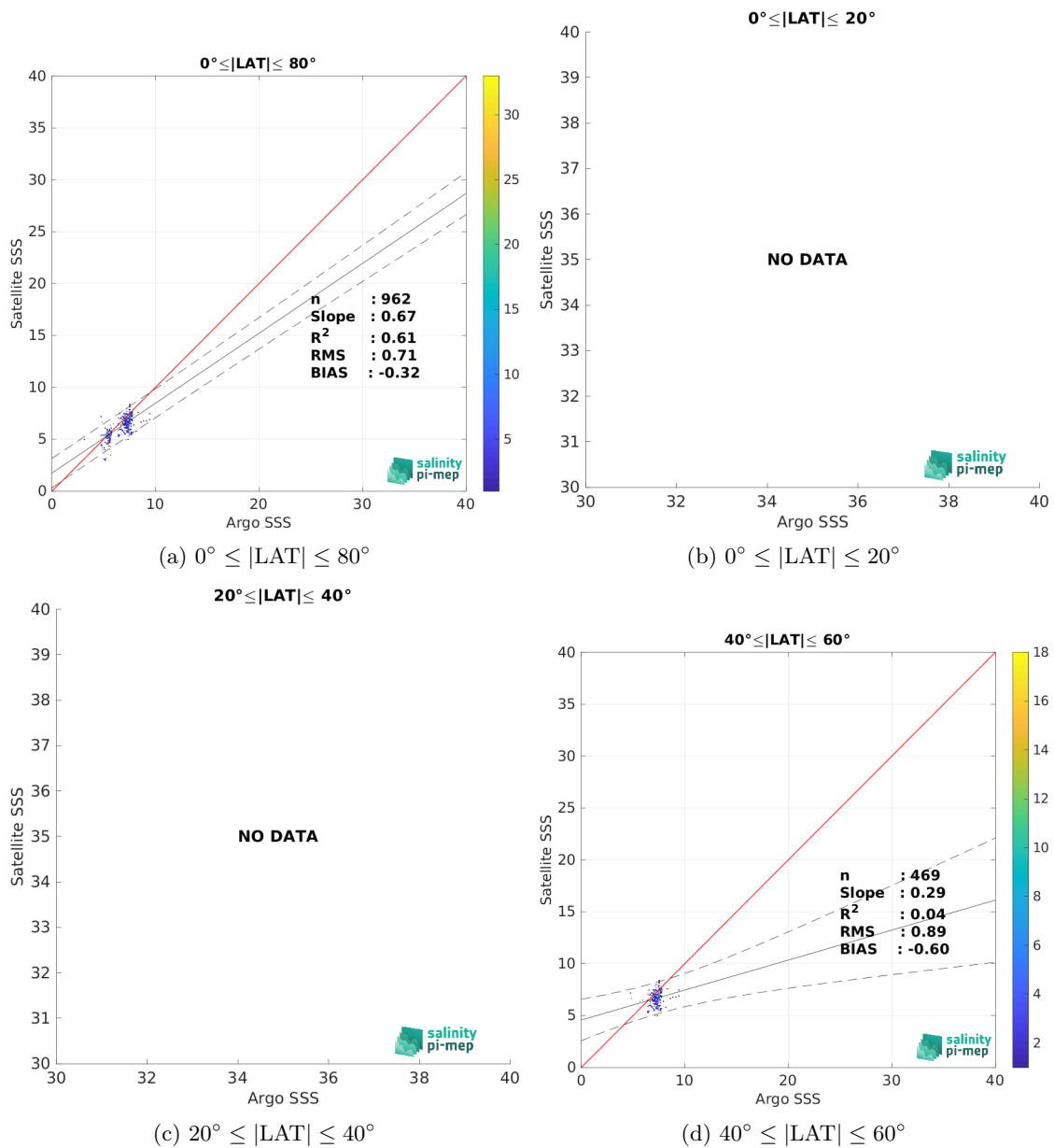
Figure 9: Contour maps of the concentration of CCI SSS L4 POLAR NH Merged-OI v4.4 - 7-day running (ESA) SSS (y-axis) versus Argo SSS (x-axis) at match-up pairs for different latitude bands. For each plot, the red line shows x=y . The black thin and dashed lines indicate a linear fit through the data cloud and the \pm 95\% confidence levels, respectively. The number match-up pairs n , the slope and R^2 coefficient of the linear fit, the root mean square (RMS) and the mean bias between satellite and in situ data are indicated for each latitude band in each plots.
