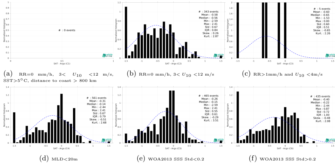
Figure 13: Normalized histogram of \Delta SSS (CCI SSS L4 POLAR NH Merged-OI v4.4 - 7-day running (ESA) - Argo) for 6 different subdatasets corresponding to: RR=0 mm/h, 3 < U_{10} < 12 m/s, SST>5°C, distance to coast > 800 km (a), RR=0 mm/h, 3 < U_{10} < 12 m/s (b), RR>1mm/h and U_{10} < 4 m/s (c), MLD<20m (d), WOA2013 SSS Std<0.2 (e), WOA2013 SSS Std>0.2 (f).
