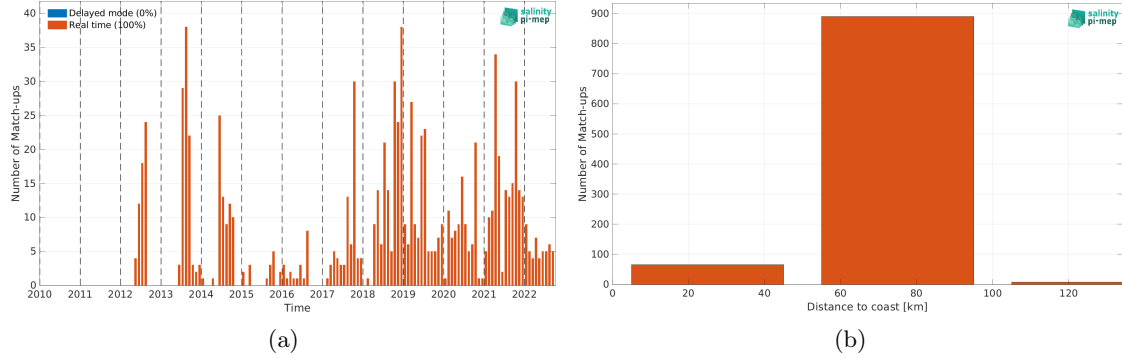
Figure 1: Number of match-ups between Argo and CCI SSS L4 POLAR NH Merged-OI v4.4 - 7-day running (ESA) SSS as a function of time (a) and as function of the distance to coast (b) over the Baltic Sea Pi-MEP region and for the full satellite product period.
