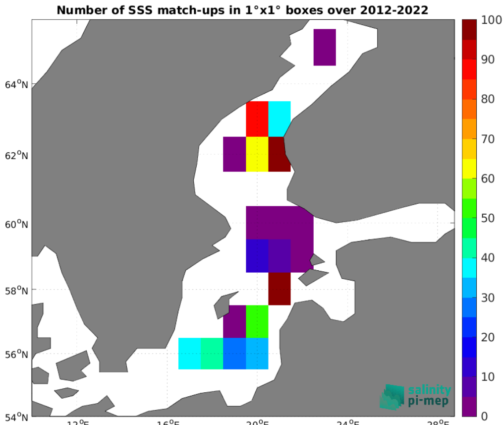
Figure 4: Number of SSS match-ups between Argo SSS and the CCI SSS L4 POLAR NH Merged-OI v4.4 - 7-day running (ESA) SSS product for the Baltic Sea Pi-MEP region over 1°×1° boxes and for the full satellite product period.
