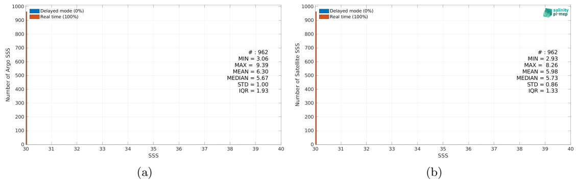
Figure 2: Histograms of SSS from Argo (a) and CCI SSS L4 POLAR NH Merged-OI v4.4 - 7-day running (ESA) (b) considering all match-up pairs per bins of 0.1 over the Baltic Sea Pi-MEP region and for the full satellite product period.
