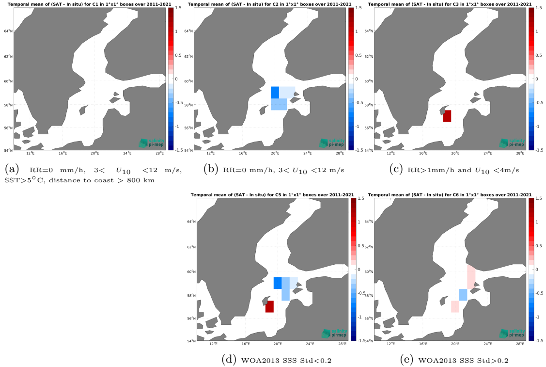
Figure 12: Temporal mean gridded over spatial boxes of size 1^{\circ}\times 1^{\circ} of \Delta\text{SSS} (CCI SSS L4 POLAR NH Merged-OI v4.4 - 30-day running (ESA) - TSG (LEGOS-DM)) for 5 different subdatasets corresponding to:RR=0 mm/h, 3 < U_{10} < 12 m/s, SST > 5^{\circ}\text{C} , distance to coast > 800 km (a), RR=0 mm/h, 3 < U_{10} < 12 m/s (b), RR > 1 mm/h and U_{10} < 4 m/s (c), WOA2013 SSS Std < 0.2 (d), WOA2013 SSS Std > 0.2 (e).
