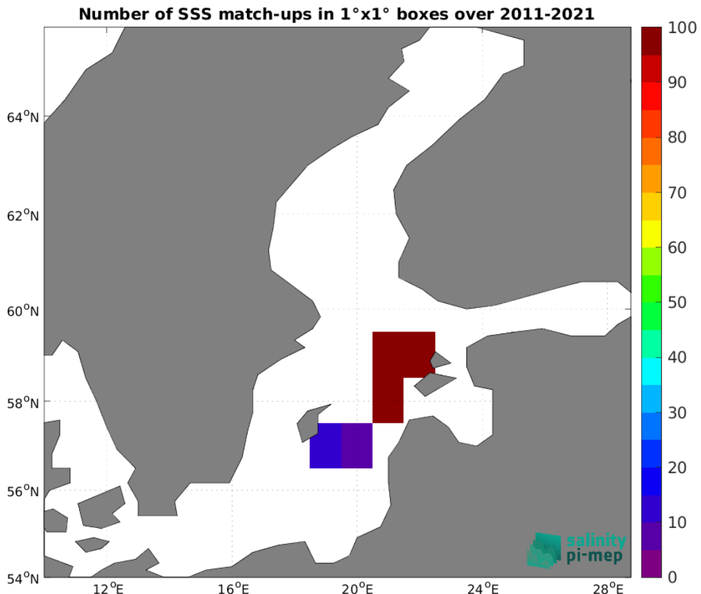
Figure 4: Number of SSS match-ups between TSG (LEGOS-DM) SSS and the CCI SSS L4 POLAR NH Merged-OI v4.4 - 30-day running (ESA) SSS product for the Baltic Sea Pi-MEP region over 1°x1° boxes and for the full satellite product period.
