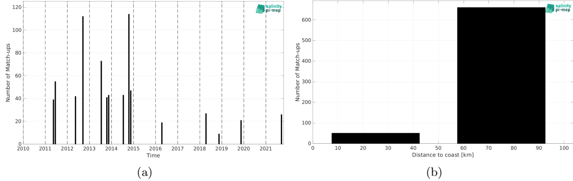
Figure 1: Number of match-ups between TSG (LEGOS-DM) and CCI SSS L4 POLAR NH Merged-OI v4.4 - 30-day running (ESA) SSS as a function of time (a) and as function of the distance to coast (b) over the Baltic Sea Pi-MEP region and for the full satellite product period.
