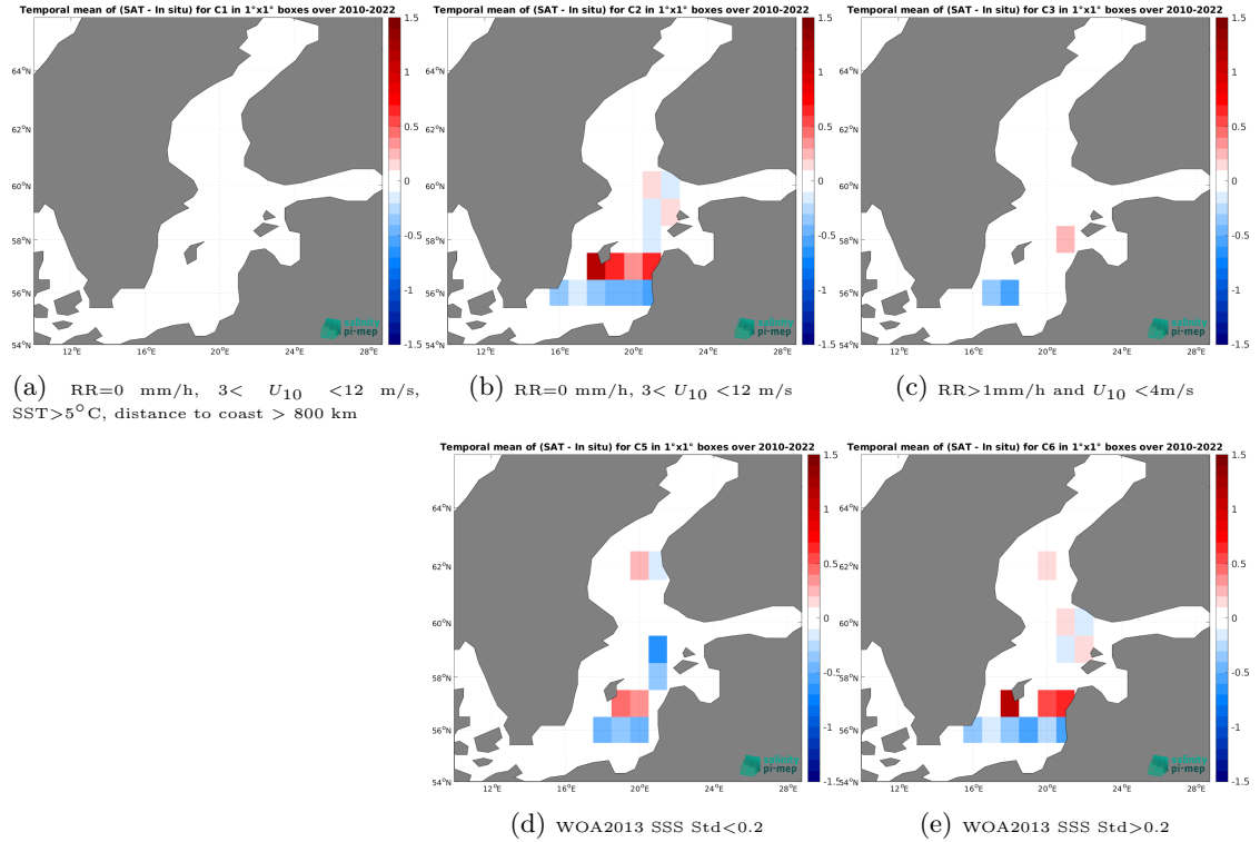
Figure 12: Temporal mean gridded over spatial boxes of size 1^{\circ}\times 1^{\circ} of \Delta\text{SSS} (CCI SSS L4 POLAR NH Merged-OI v4.4 - 30-day running (ESA) - ICES) for 5 different subdatasets corresponding to:RR=0 mm/h, 3 < U_{10} < 12 m/s, SST >5^{\circ}\text{C} , distance to coast > 800 km (a), RR=0 mm/h, 3 < U_{10} < 12 m/s (b), RR >1 mm/h and U_{10} < 4 m/s (c), WOA2013 SSS Std <0.2 (d), WOA2013 SSS Std >0.2 (e).
