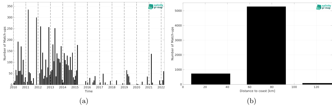
Figure 1: Number of match-ups between ICES and CCI SSS L4 POLAR NH Merged-OI v4.4 - 30-day running (ESA) SSS as a function of time (a) and as function of the distance to coast (b) over the Baltic Sea Pi-MEP region and for the full satellite product period.
