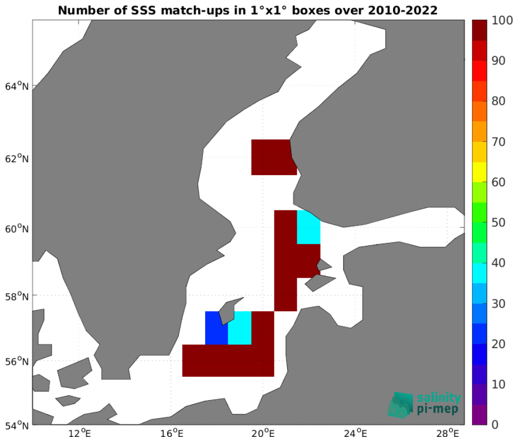
Figure 4: Number of SSS match-ups between ICES SSS and the CCI SSS L4 POLAR NH Merged-OI v4.4 - 30-day running (ESA) SSS product for the Baltic Sea Pi-MEP region over 1°x1° boxes and for the full satellite product period.
