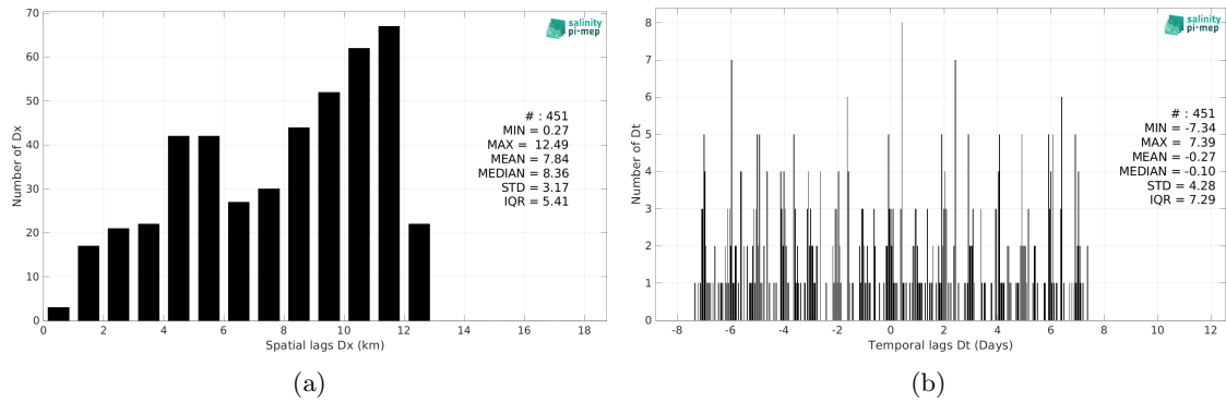
Figure 5: Histograms of the spatial (a) and temporal (b) lags between the location/time of the Argo measurement and the date of the corresponding CCI SSS L4 POLAR NH Merged-OI v4.4 - 30-day running (ESA) SSS pixel.
