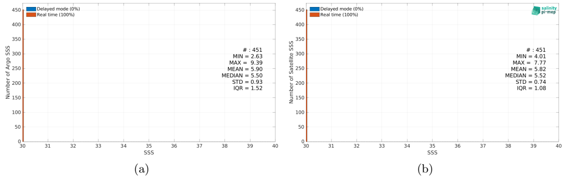
Figure 2: Histograms of SSS from Argo (a) and CCI SSS L4 POLAR NH Merged-OI v4.4 - 30-day running (ESA) (b) considering all match-up pairs per bins of 0.1 over the Baltic Sea Pi-MEP region and for the full satellite product period.
