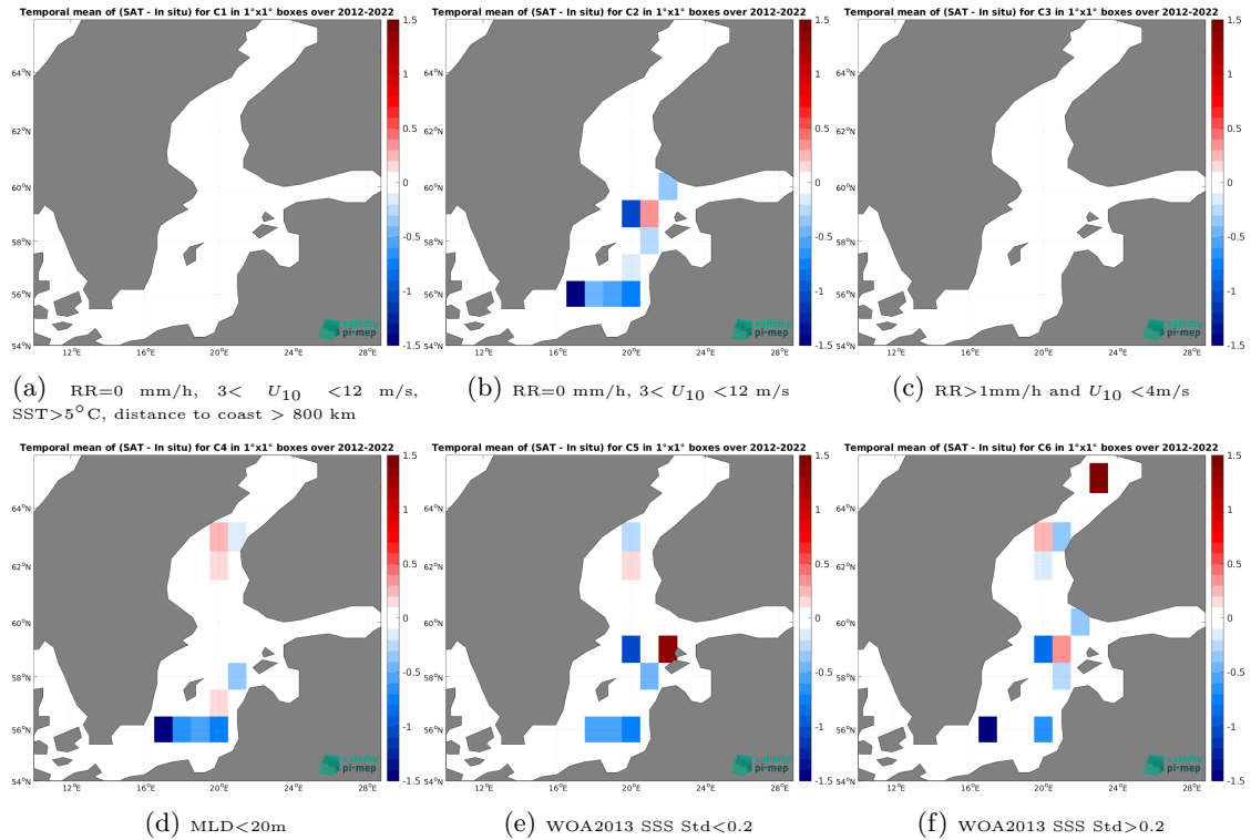
Figure 12: Temporal mean gridded over spatial boxes of size 1^{\circ}\times 1^{\circ} of \Delta\text{SSS} (CCI SSS L4 POLAR NH Merged-OI v4.4 - 30-day running (ESA) - Argo) for 6 different subdatasets corresponding to:RR=0 mm/h, 3 < U_{10} < 12 m/s, SST >5^{\circ}\text{C} , distance to coast > 800 km (a), RR=0 mm/h, 3 < U_{10} < 12 m/s (b), RR >1\text{mm/h} and U_{10} < 4\text{m/s} (c),MLD <20\text{m} (d),WOA2013 SSS Std <0.2 (e),WOA2013 SSS Std >0.2 (f).
