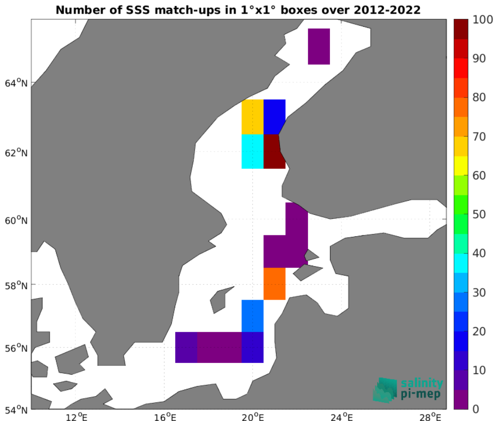
Figure 4: Number of SSS match-ups between Argo SSS and the CCI SSS L4 POLAR NH Merged-OI v4.4 - 30-day running (ESA) SSS product for the Baltic Sea Pi-MEP region over 1°x1° boxes and for the full satellite product period.
