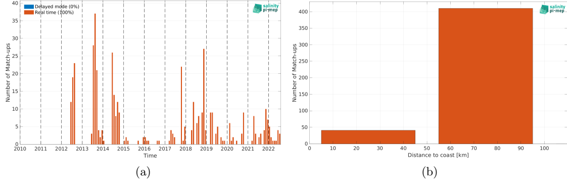
Figure 1: Number of match-ups between Argo and CCI SSS L4 POLAR NH Merged-OI v4.4 - 30-day running (ESA) SSS as a function of time (a) and as function of the distance to coast (b) over the Baltic Sea Pi-MEP region and for the full satellite product period.
