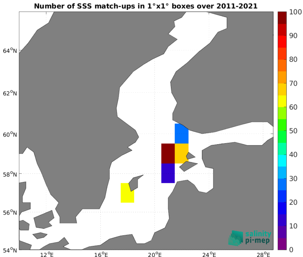
Figure 5: Number of SSS match-ups between TSG (LEGOS-DM) SSS and the CCI SSS L4 Merged-OI v5.5 - 7-day running (ESA) SSS product for the Baltic Sea Pi-MEP region over 1°x1° boxes and for the full satellite product period.
