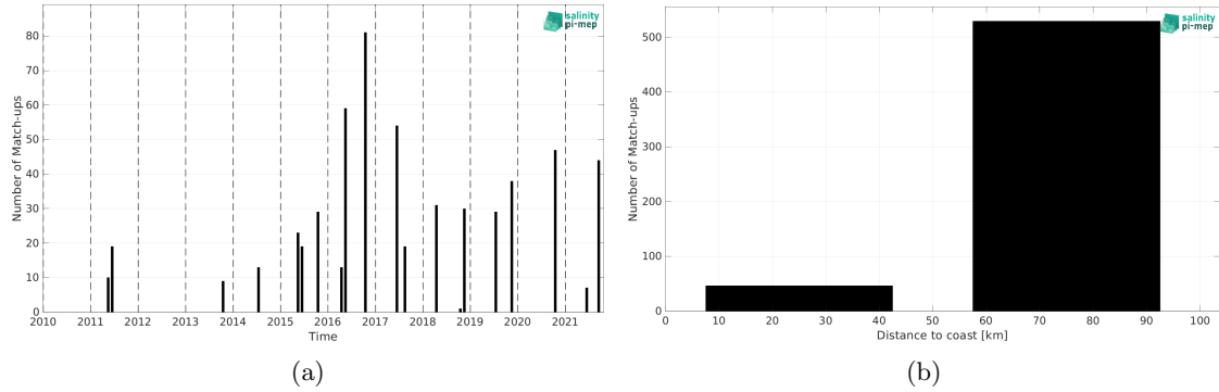
Figure 2: Number of match-ups between TSG (LEGOS-DM) and CCI SSS L4 Merged-OI v5.5 - 7-day running (ESA) SSS as a function of time (a) and as function of the distance to coast (b) over the Baltic Sea Pi-MEP region and for the full satellite product period.
