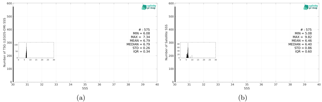
Figure 3: Histograms of SSS from TSG (LEGOS-DM) (a) and CCI SSS L4 Merged-OI v5.5 - 7-day running (ESA) (b) considering all match-up pairs per bins of 0.1 over the Baltic Sea Pi-MEP region and for the full satellite product period.
