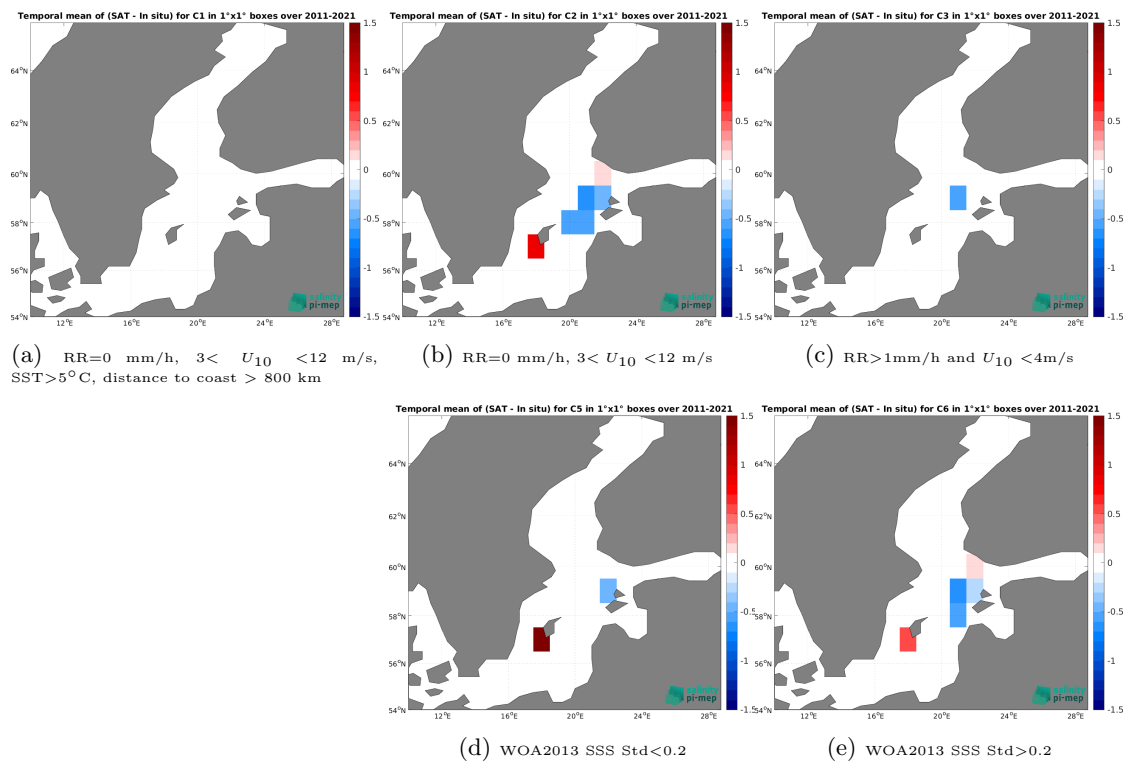
Figure 14: Temporal mean gridded over spatial boxes of size 1^\circ \times 1^\circ of \Delta SSS (CCI SSS L4 Merged-OI v5.5 - 7-day running (ESA) - TSG (LEGOS-DM)) for 5 different subdatasets corresponding to: RR=0 mm/h, 3 < U_{10} < 12 m/s, SST >5^\circ\text{C} , distance to coast > 800 km (a), RR=0 mm/h, 3 < U_{10} < 12 m/s (b), RR >1 mm/h and U_{10} < 4 m/s (c), WOA2013 SSS Std <0.2 (d), WOA2013 SSS Std >0.2 (e).
