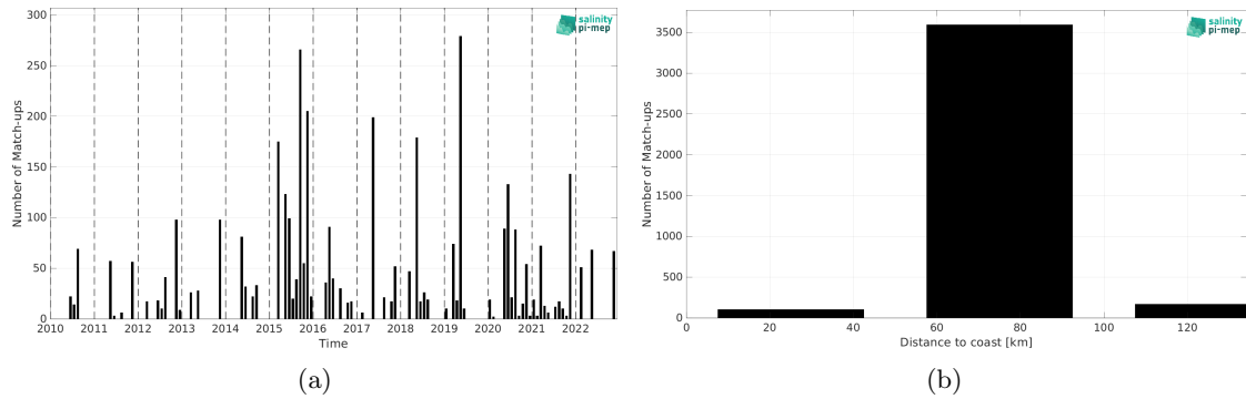
Figure 2: Number of match-ups between ICES and CCI SSS L4 Merged-OI v5.5 - 7-day running (ESA) SSS as a function of time (a) and as function of the distance to coast (b) over the Baltic Sea Pi-MEP region and for the full satellite product period.
