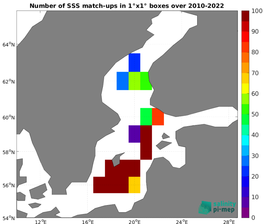
Figure 5: Number of SSS match-ups between ICES SSS and the CCI SSS L4 Merged-OI v5.5 - 7-day running (ESA) SSS product for the Baltic Sea Pi-MEP region over 1°x1° boxes and for the full satellite product period.
