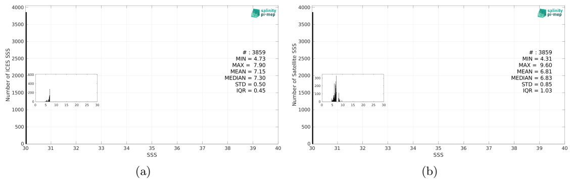
Figure 3: Histograms of SSS from ICES (a) and CCI SSS L4 Merged-OI v5.5 - 7-day running (ESA) (b) considering all match-up pairs per bins of 0.1 over the Baltic Sea Pi-MEP region and for the full satellite product period.
