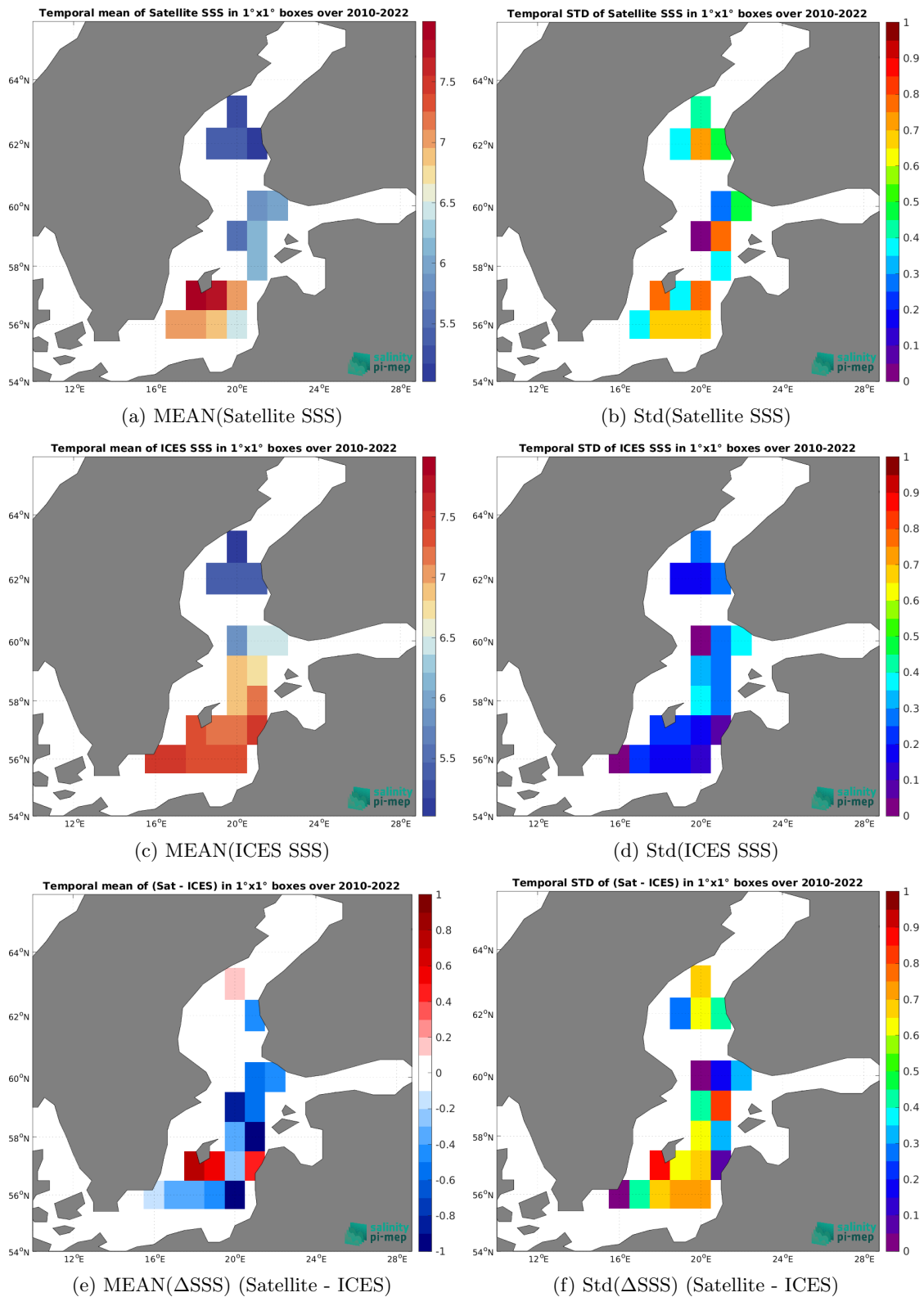
Figure 7: Temporal mean (left) and Std (right) of SSS from CCI SSS L4 Merged-OI v5.5 - 7-day running (ESA) (top), ICES (middle), and of \Delta SSS (Satellite - ICES). Only match-up pairs are used to generate these maps.
