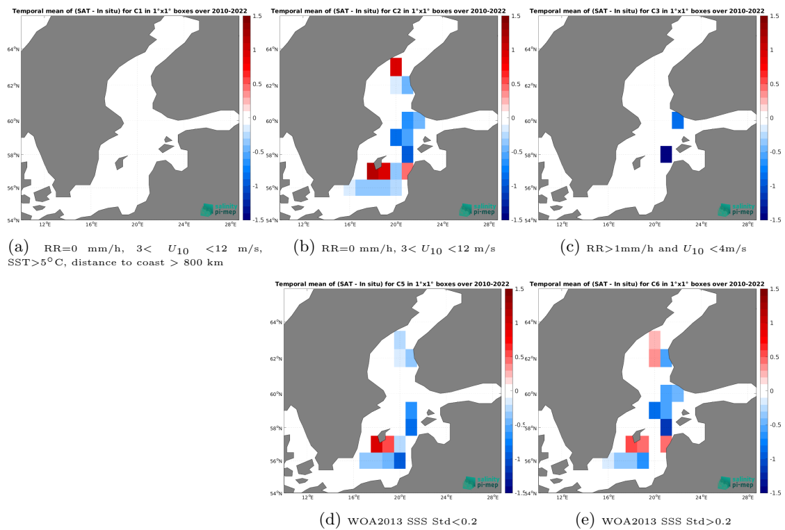
Figure 14: Temporal mean gridded over spatial boxes of size 1^\circ \times 1^\circ of \Delta SSS (CCI SSS L4 Merged-OI v5.5 - 7-day running (ESA) - ICES) for 5 different subdatasets corresponding to:RR=0 mm/h, 3 < U_{10} < 12 m/s, SST >5^\circ\text{C} , distance to coast > 800 km (a), RR=0 mm/h, 3 < U_{10} < 12 m/s (b), RR >1 mm/h and U_{10} < 4 m/s (c), WOA2013 SSS Std <0.2 (d), WOA2013 SSS Std >0.2 (e).
