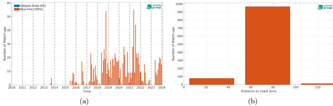
Figure 2: Number of match-ups between Argo and CCI SSS L4 Merged-OI v5.5 - 7-day running (ESA) SSS as a function of time (a) and as function of the distance to coast (b) over the Baltic Sea Pi-MEP region and for the full satellite product period.
