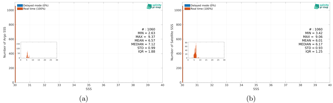
Figure 3: Histograms of SSS from Argo (a) and CCI SSS L4 Merged-OI v5.5 - 7-day running (ESA) (b) considering all match-up pairs per bins of 0.1 over the Baltic Sea Pi-MEP region and for the full satellite product period.
