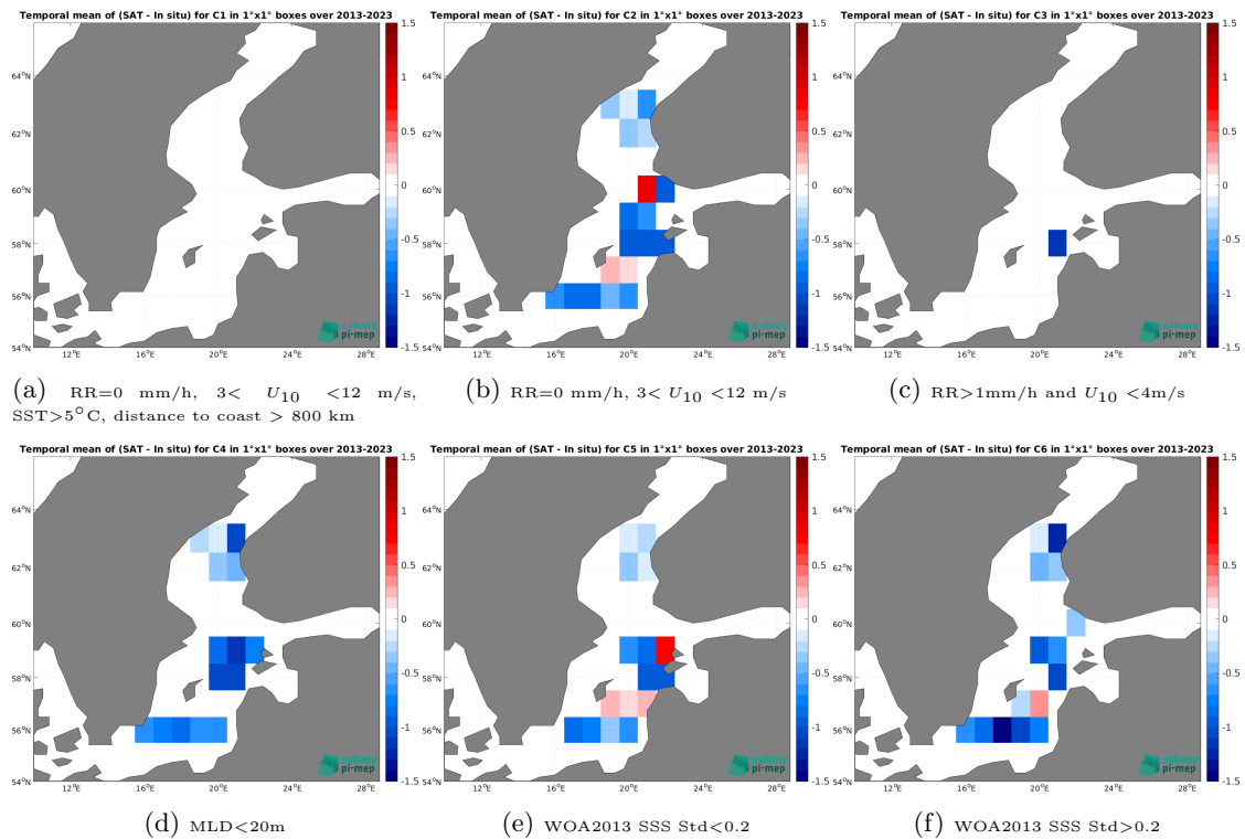
Figure 14: Temporal mean gridded over spatial boxes of size 1^\circ \times 1^\circ of \Delta SSS (CCI SSS L4 Merged-OI v5.5 - 7-day running (ESA) - Argo) for 6 different subdatasets corresponding to:RR=0 mm/h, 3 < U_{10} < 12 m/s, SST > 5^\circ\text{C} , distance to coast > 800 km (a), RR=0 mm/h, 3 < U_{10} < 12 m/s (b), RR > 1 mm/h and U_{10} < 4 m/s (c),MLD < 20 m (d),WOA2013 SSS Std < 0.2 (e),WOA2013 SSS Std > 0.2 (f).
