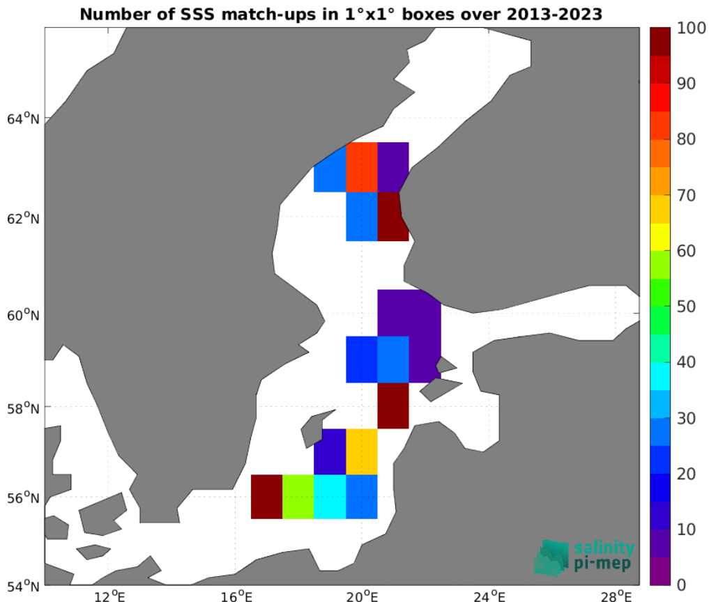
Figure 5: Number of SSS match-ups between Argo SSS and the CCI SSS L4 Merged-OI v5.5 - 7-day running (ESA) SSS product for the Baltic Sea Pi-MEP region over 1°x1° boxes and for the full satellite product period.
