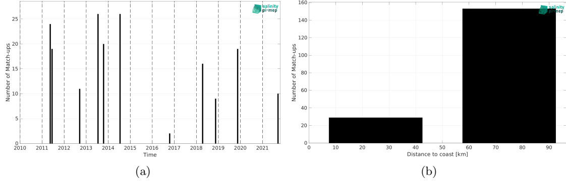
Figure 2: Number of match-ups between TSG (LEGOS-DM) and CCI SSS L4 Merged-OI v5.5 - 30-day running (ESA) SSS as a function of time (a) and as function of the distance to coast (b) over the Baltic Sea Pi-MEP region and for the full satellite product period.
