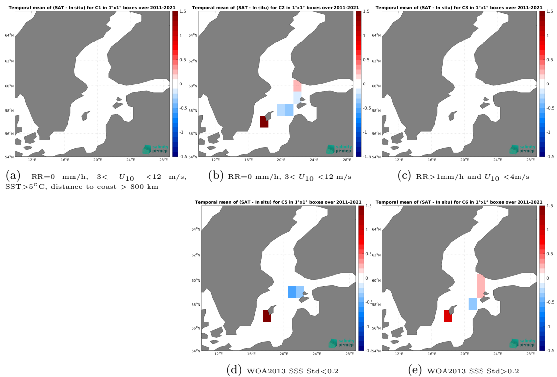
Figure 14: Temporal mean gridded over spatial boxes of size 1^\circ \times 1^\circ of \Delta SSS (CCI SSS L4 Merged-OI v5.5 - 30-day running (ESA) - TSG (LEGOS-DM)) for 5 different subdatasets corresponding to:RR=0 mm/h, 3 < U_{10} < 12 m/s, SST >5^\circ C, distance to coast > 800 km (a), RR=0 mm/h, 3 < U_{10} < 12 m/s (b), RR >1 mm/h and U_{10} < 4 m/s (c), WOA2013 SSS Std <0.2 (d), WOA2013 SSS Std >0.2 (e).
