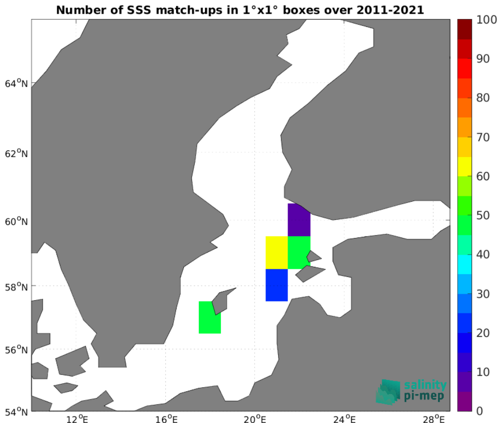
Figure 5: Number of SSS match-ups between TSG (LEGOS-DM) SSS and the CCI SSS L4 Merged-OI v5.5 - 30-day running (ESA) SSS product for the Baltic Sea Pi-MEP region over 1°x1° boxes and for the full satellite product period.
