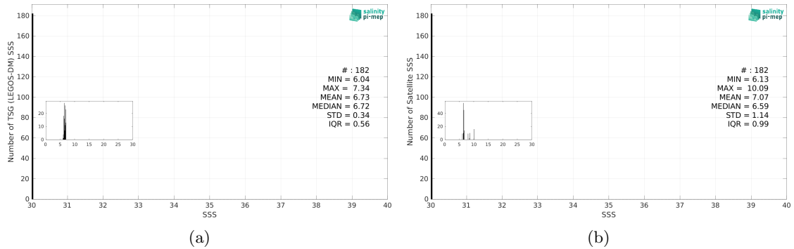
Figure 3: Histograms of SSS from TSG (LEGOS-DM) (a) and CCI SSS L4 Merged-OI v5.5 - 30-day running (ESA) (b) considering all match-up pairs per bins of 0.1 over the Baltic Sea Pi-MEP region and for the full satellite product period.
