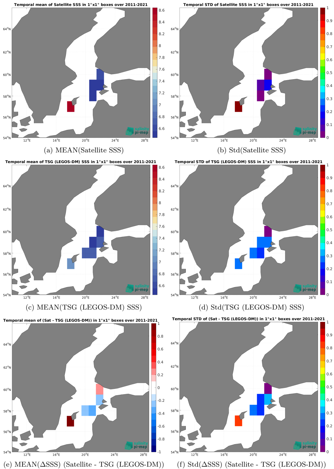
Figure 7: Temporal mean (left) and Std (right) of SSS from CCI SSS L4 Merged-OI v5.5 - 30-day running (ESA) (top), TSG (LEGOS-DM) (middle), and of \Delta SSS (Satellite - TSG (LEGOS-DM)). Only match-up pairs are used to generate these maps.
