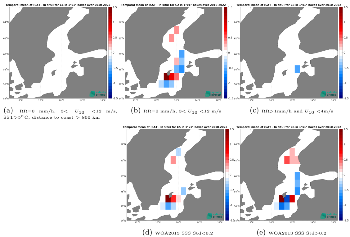
Figure 14: Temporal mean gridded over spatial boxes of size 1^\circ \times 1^\circ of \Delta SSS (CCI SSS L4 Merged-OI v5.5 - 30-day running (ESA) - ICES) for 5 different subdatasets corresponding to:RR=0 mm/h, 3 < U_{10} < 12 m/s, SST >5^\circ C, distance to coast > 800 km (a), RR=0 mm/h, 3 < U_{10} < 12 m/s (b), RR >1 mm/h and U_{10} < 4 m/s (c), WOA2013 SSS Std <0.2 (d), WOA2013 SSS Std >0.2 (e).
