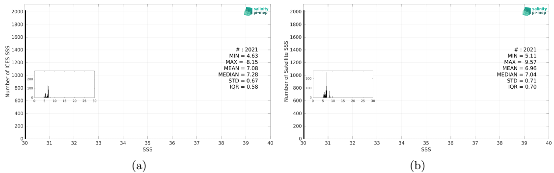
Figure 3: Histograms of SSS from ICES (a) and CCI SSS L4 Merged-OI v5.5 - 30-day running (ESA) (b) considering all match-up pairs per bins of 0.1 over the Baltic Sea Pi-MEP region and for the full satellite product period.
