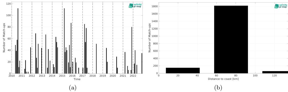
Figure 2: Number of match-ups between ICES and CCI SSS L4 Merged-OI v5.5 - 30-day running (ESA) SSS as a function of time (a) and as function of the distance to coast (b) over the Baltic Sea Pi-MEP region and for the full satellite product period.
