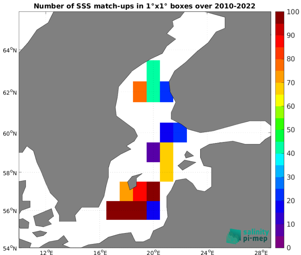
Figure 5: Number of SSS match-ups between ICES SSS and the CCI SSS L4 Merged-OI v5.5 - 30-day running (ESA) SSS product for the Baltic Sea Pi-MEP region over 1°×1° boxes and for the full satellite product period.
