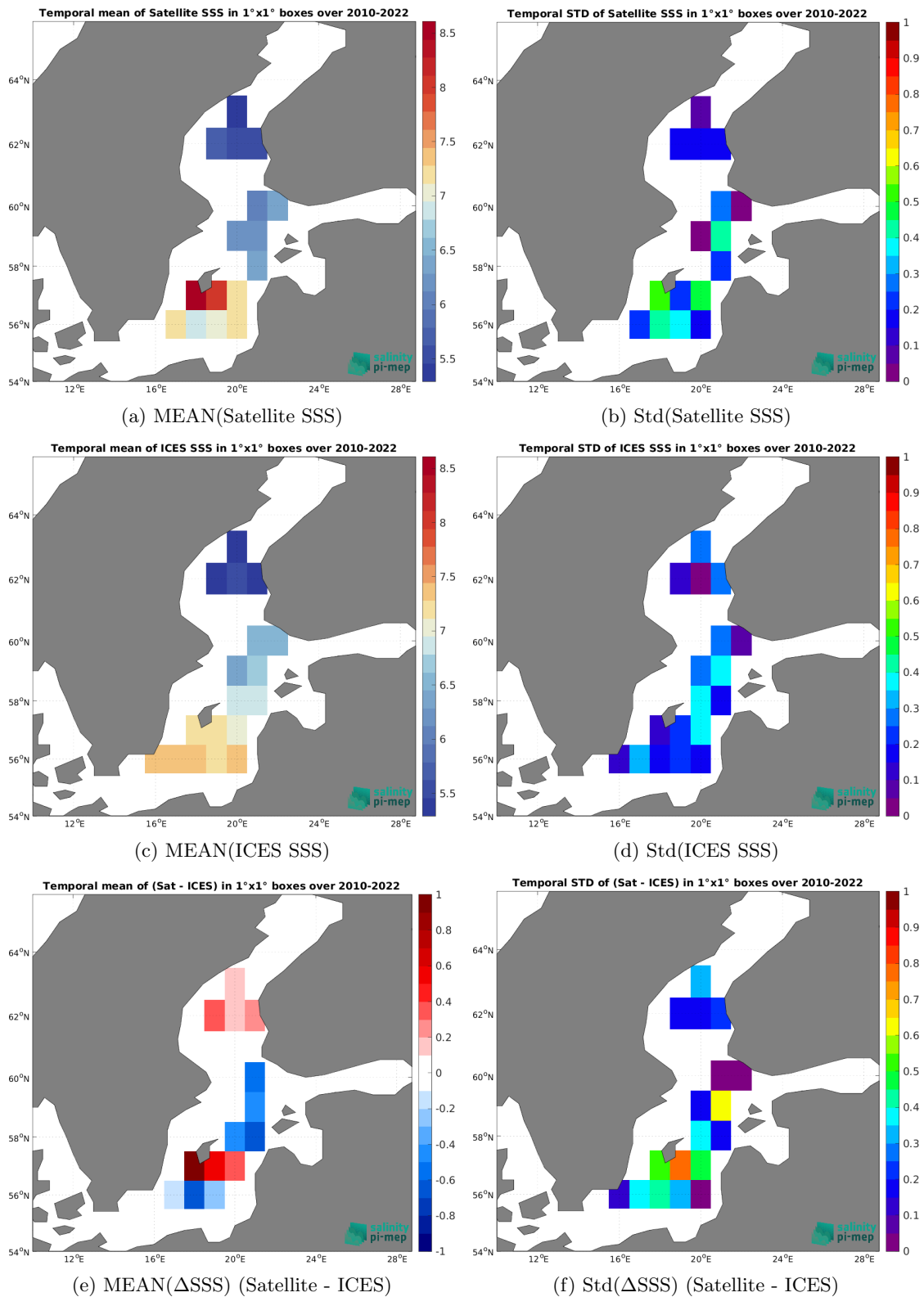
Figure 7: Temporal mean (left) and Std (right) of SSS from CCI SSS L4 Merged-OI v5.5 - 30-day running (ESA) (top), ICES (middle), and of \Delta SSS (Satellite - ICES). Only match-up pairs are used to generate these maps.
