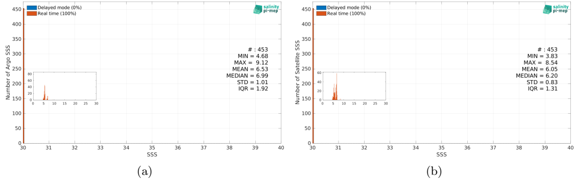
Figure 3: Histograms of SSS from Argo (a) and CCI SSS L4 Merged-OI v5.5 - 30-day running (ESA) (b) considering all match-up pairs per bins of 0.1 over the Baltic Sea Pi-MEP region and for the full satellite product period.
