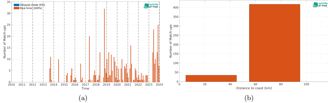
Figure 2: Number of match-ups between Argo and CCI SSS L4 Merged-OI v5.5 - 30-day running (ESA) SSS as a function of time (a) and as function of the distance to coast (b) over the Baltic Sea Pi-MEP region and for the full satellite product period.
