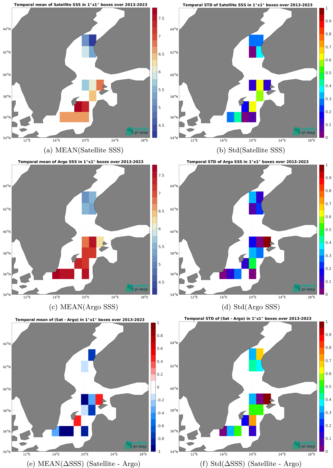
Figure 7: Temporal mean (left) and Std (right) of SSS from CCI SSS L4 Merged-OI v5.5 - 30-day running (ESA) (top), Argo (middle), and of \Delta SSS (Satellite - Argo). Only match-up pairs are used to generate these maps.
