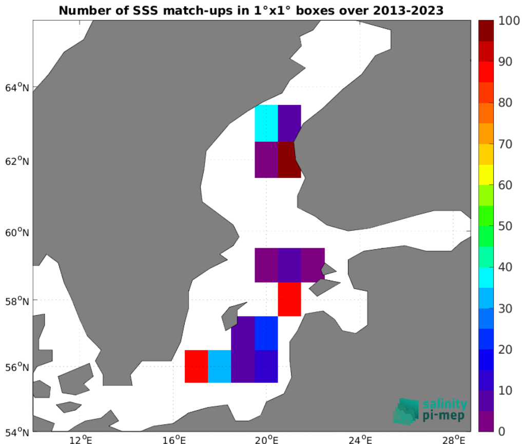
Figure 5: Number of SSS match-ups between Argo SSS and the CCI SSS L4 Merged-OI v5.5 - 30-day running (ESA) SSS product for the Baltic Sea Pi-MEP region over 1°×1° boxes and for the full satellite product period.
