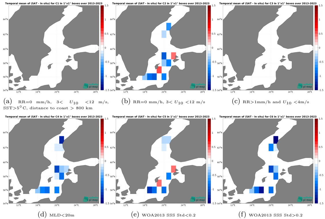
Figure 14: Temporal mean gridded over spatial boxes of size 1^\circ \times 1^\circ of \Delta SSS (CCI SSS L4 Merged-OI v5.5 - 30-day running (ESA) - Argo) for 6 different subdatasets corresponding to:RR=0 mm/h, 3 < U_{10} < 12 m/s, SST > 5^\circ\text{C} , distance to coast > 800 km (a), RR=0 mm/h, 3 < U_{10} < 12 m/s (b), RR > 1 mm/h and U_{10} < 4 m/s (c),MLD < 20 m (d),WOA2013 SSS Std < 0.2 (e),WOA2013 SSS Std > 0.2 (f).
