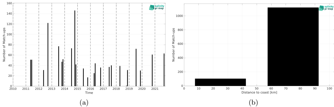
Figure 2: Number of match-ups between TSG (LEGOS-DM) and CCI SSS L4 Merged-OI v4.41 - 7-day running (ESA) SSS as a function of time (a) and as function of the distance to coast (b) over the Baltic Sea Pi-MEP region and for the full satellite product period.
