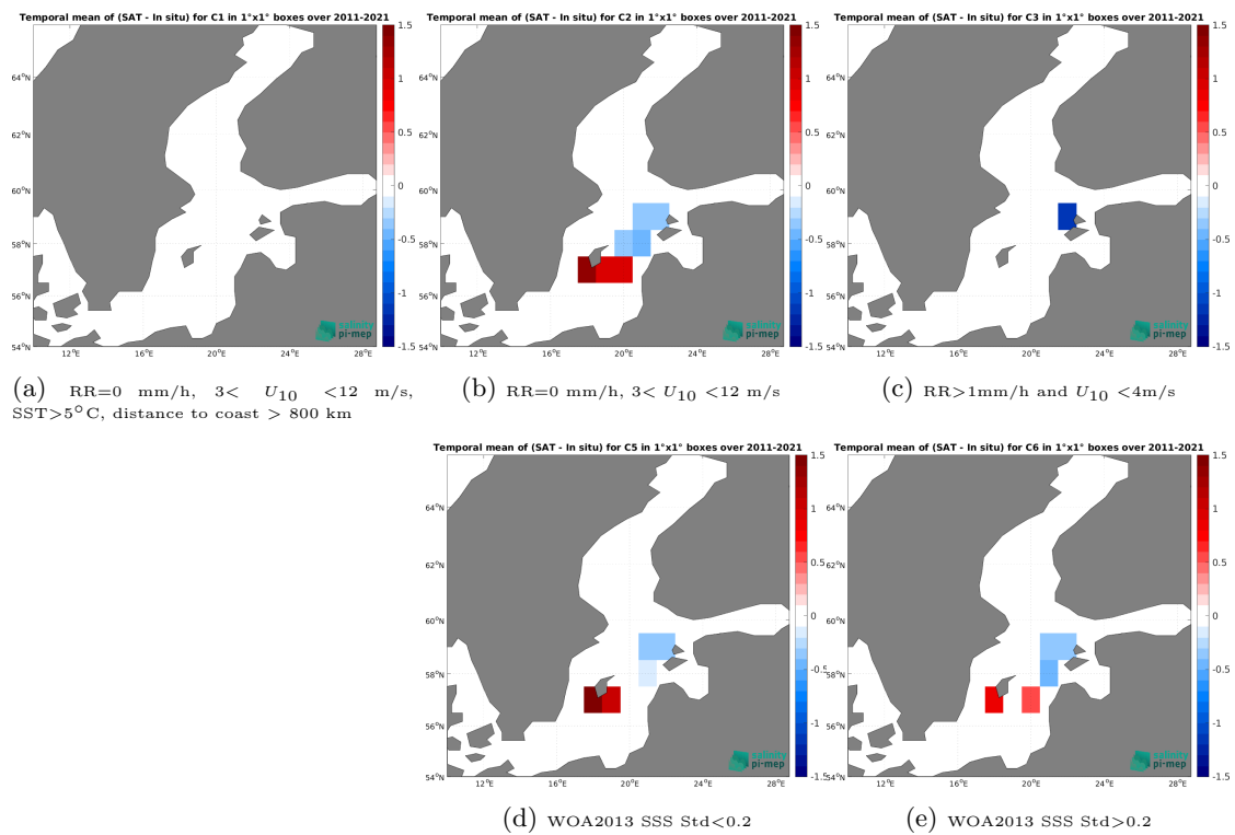
Figure 14: Temporal mean gridded over spatial boxes of size 1^\circ \times 1^\circ of \Delta SSS (CCI SSS L4 Merged-OI v4.41 - 7-day running (ESA) - TSG (LEGOS-DM)) for 5 different subdatasets corresponding to:RR=0 mm/h, 3 < U_{10} < 12 m/s, SST >5^\circ\text{C} , distance to coast > 800 km (a), RR=0 mm/h, 3 < U_{10} < 12 m/s (b), RR >1 mm/h and U_{10} < 4 m/s (c), WOA2013 SSS Std <0.2 (d), WOA2013 SSS Std >0.2 (e).
