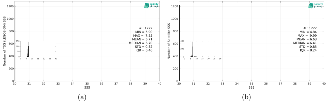
Figure 3: Histograms of SSS from TSG (LEGOS-DM) (a) and CCI SSS L4 Merged-OI v4.41 - 7-day running (ESA) (b) considering all match-up pairs per bins of 0.1 over the Baltic Sea Pi-MEP region and for the full satellite product period.
