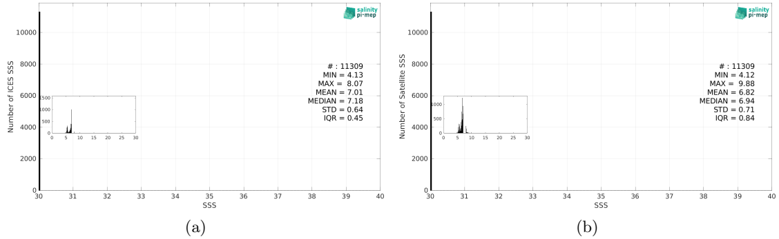
Figure 3: Histograms of SSS from ICES (a) and CCI SSS L4 Merged-OI v4.41 - 7-day running (ESA) (b) considering all match-up pairs per bins of 0.1 over the Baltic Sea Pi-MEP region and for the full satellite product period.
