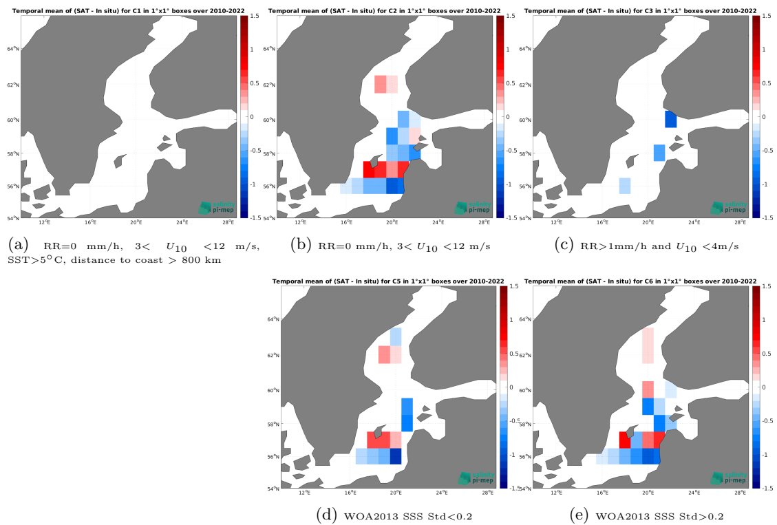
Figure 14: Temporal mean gridded over spatial boxes of size 1^\circ \times 1^\circ of \Delta SSS (CCI SSS L4 Merged-OI v4.41 - 7-day running (ESA) - ICES) for 5 different subdatasets corresponding to:RR=0 mm/h, 3 < U_{10} < 12 m/s, SST >5^\circ\text{C} , distance to coast > 800 km (a), RR=0 mm/h, 3 < U_{10} < 12 m/s (b), RR >1 mm/h and U_{10} < 4 m/s (c), WOA2013 SSS Std <0.2 (d), WOA2013 SSS Std >0.2 (e).
