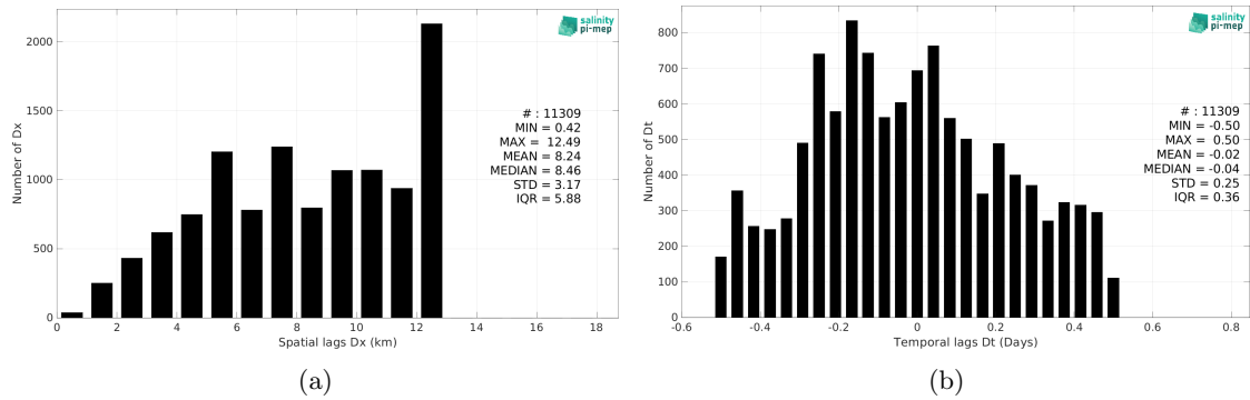
Figure 6: Histograms of the spatial (a) and temporal (b) lags between the location/time of the ICES measurement and the date of the corresponding CCI SSS L4 Merged-OI v4.41 - 7-day running (ESA) SSS pixel.
