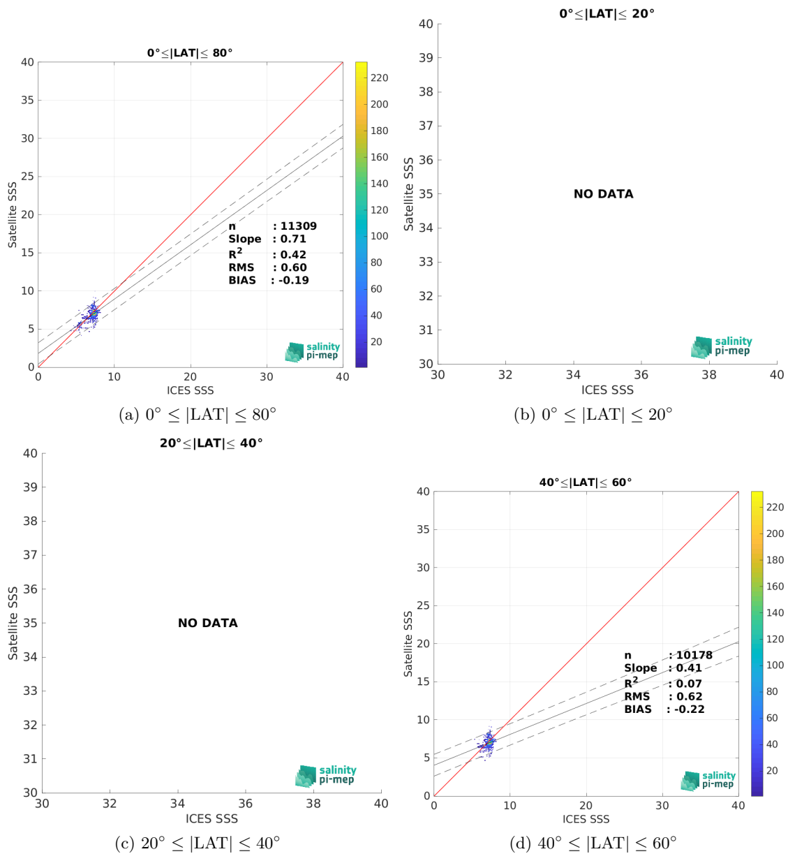
Figure 10: Contour maps of the concentration of CCI SSS L4 Merged-OI v4.41 - 7-day running (ESA) SSS (y-axis) versus ICES SSS (x-axis) at match-up pairs for different latitude bands. For each plot, the red line shows x=y . The black thin and dashed lines indicate a linear fit through the data cloud and the \pm 95\% confidence levels, respectively. The number match-up pairs n , the slope and R^2 coefficient of the linear fit, the root mean square (RMS) and the mean bias between satellite and in situ data are indicated for each latitude band in each plots.
