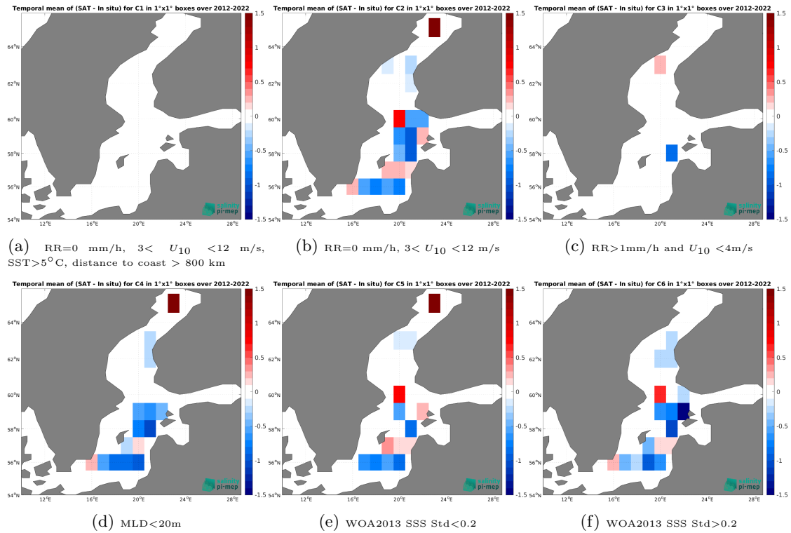
Figure 14: Temporal mean gridded over spatial boxes of size 1^\circ \times 1^\circ of \Delta SSS (CCI SSS L4 Merged-OI v4.41 - 7-day running (ESA) - Argo) for 6 different subdatasets corresponding to:RR=0 mm/h, 3 < U_{10} < 12 m/s, SST >5^\circ C, distance to coast > 800 km (a), RR=0 mm/h, 3 < U_{10} < 12 m/s (b), RR >1 mm/h and U_{10} < 4 m/s (c),MLD <20 m (d),WOA2013 SSS Std <0.2 (e),WOA2013 SSS Std >0.2 (f).
