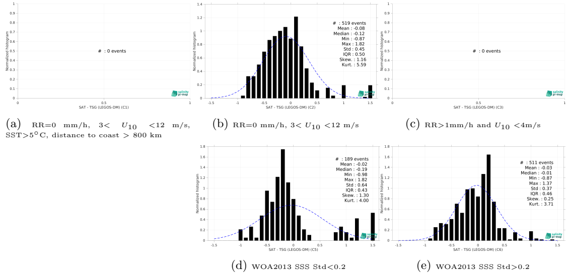
Figure 15: Normalized histogram of \Delta SSS (CCI SSS L4 Merged-OI v4.41 - 30-day running (ESA) - TSG (LEGOS-DM)) for 5 different subdatasets corresponding to: RR=0 mm/h, 3 < U_{10} < 12 m/s, SST > 5°C, distance to coast > 800 km (a), RR=0 mm/h, 3 < U_{10} < 12 m/s (b), RR > 1mm/h and U_{10} < 4 m/s (c), WOA2013 SSS Std < 0.2 (d), WOA2013 SSS Std > 0.2 (e).
