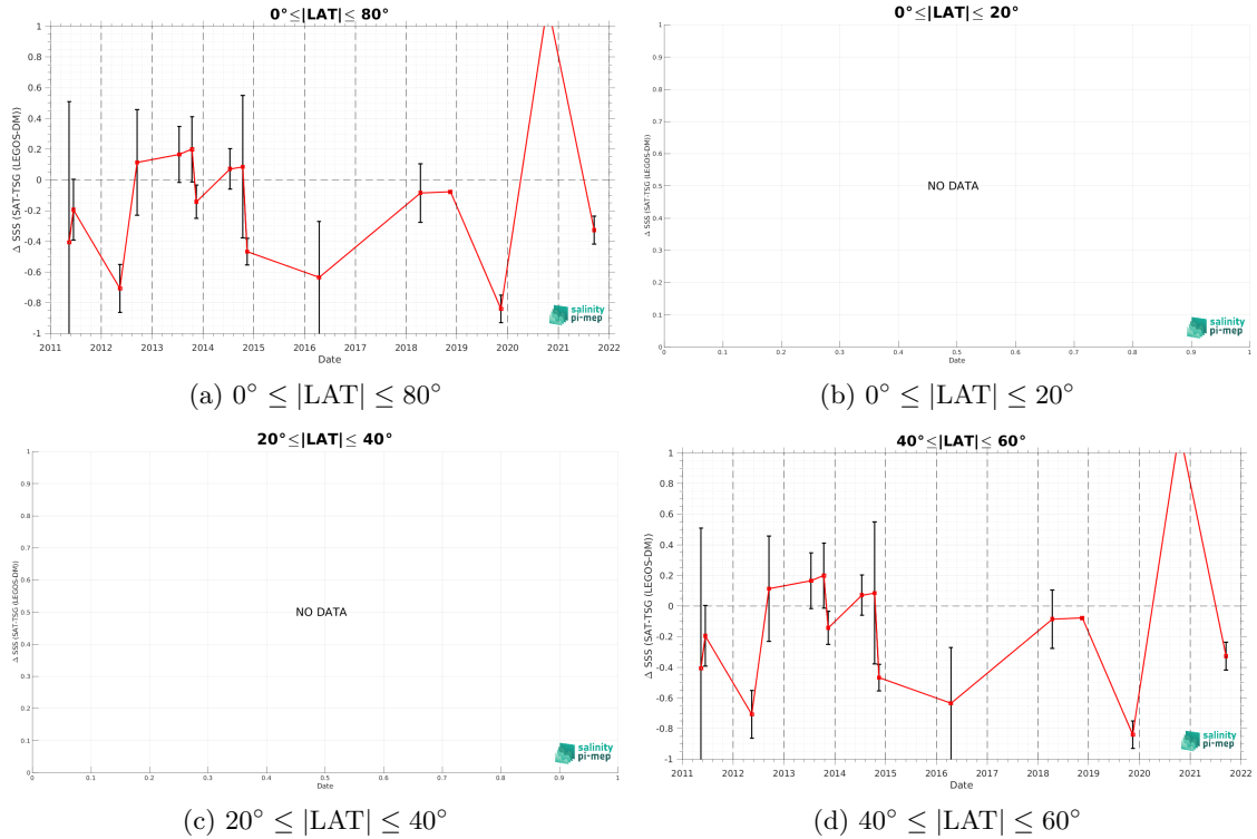
Figure 11: Monthly median (red curves) of \Delta SSS (Satellite - in situ ) between CCI SSS L4 Merged-OI v4.41 - 30-day running (ESA) and TSG (LEGOS-DM) SSS as function of time for all the collected Pi-MEP match-up pairs estimated over the Baltic Sea Pi-MEP region and for the full satellite product period are shown for different latitude bands: (a) 80^{\circ}\text{S}-80^{\circ}\text{N} , (b) 20^{\circ}\text{S}-20^{\circ}\text{N} , (c) 40^{\circ}\text{S}-20^{\circ}\text{S} and 20^{\circ}\text{N}-40^{\circ}\text{N} and (d) 60^{\circ}\text{S}-40^{\circ}\text{S} and 40^{\circ}\text{N}-60^{\circ}\text{N} .
