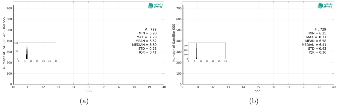
Figure 3: Histograms of SSS from TSG (LEGOS-DM) (a) and CCI SSS L4 Merged-OI v4.41 - 30-day running (ESA) (b) considering all match-up pairs per bins of 0.1 over the Baltic Sea Pi-MEP region and for the full satellite product period.
