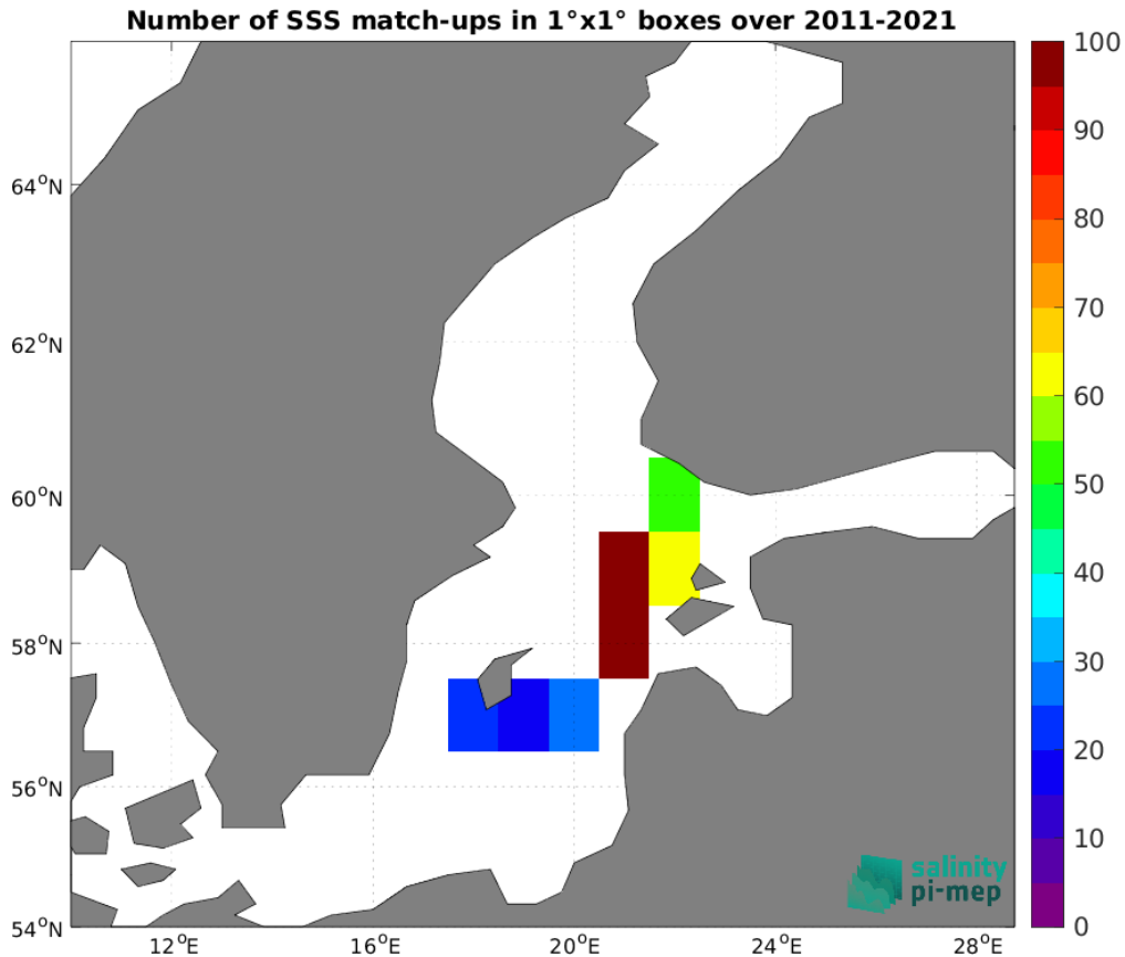
Figure 5: Number of SSS match-ups between TSG (LEGOS-DM) SSS and the CCI SSS L4 Merged-OI v4.41 - 30-day running (ESA) SSS product for the Baltic Sea Pi-MEP region over 1^\circ \times 1^\circ boxes and for the full satellite product period.
