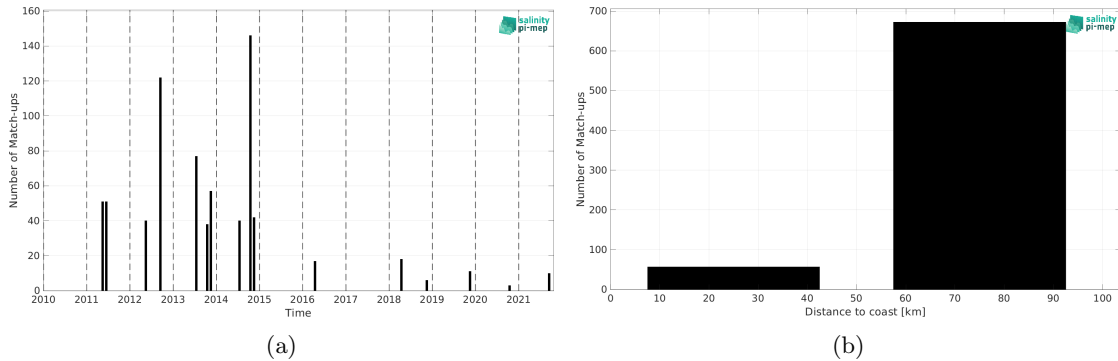
Figure 2: Number of match-ups between TSG (LEGOS-DM) and CCI SSS L4 Merged-OI v4.41 - 30-day running (ESA) SSS as a function of time (a) and as function of the distance to coast (b) over the Baltic Sea Pi-MEP region and for the full satellite product period.
