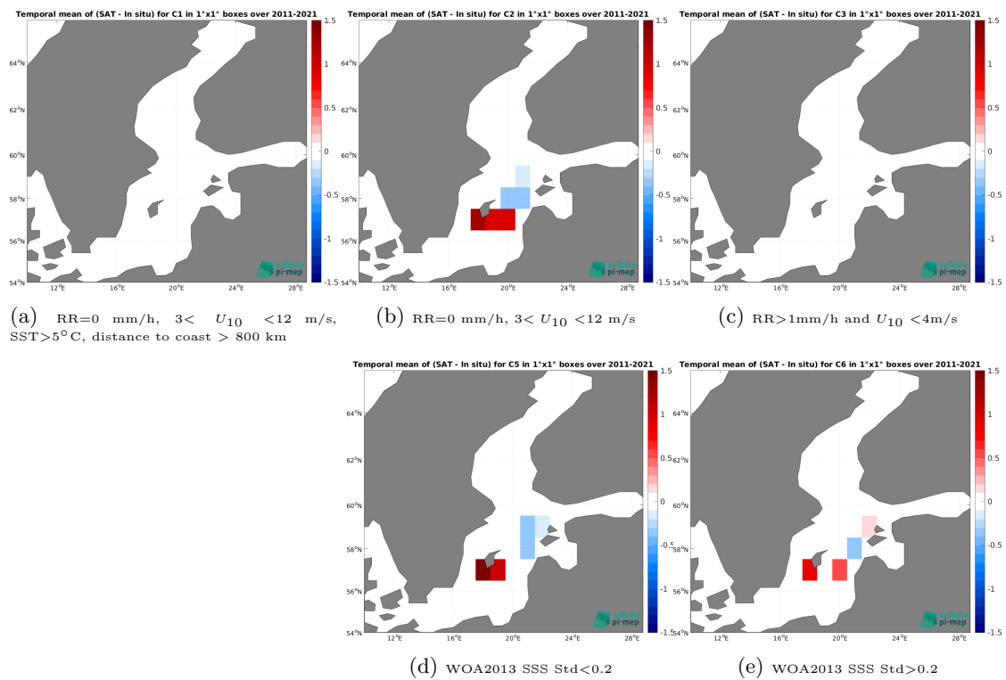
Figure 14: Temporal mean gridded over spatial boxes of size 1^\circ \times 1^\circ of \Delta SSS (CCI SSS L4 Merged-OI v4.41 - 30-day running (ESA) - TSG (LEGOS-DM)) for 5 different subdatasets corresponding to:RR=0 mm/h, 3 < U_{10} < 12 m/s, SST >5^\circ\text{C} , distance to coast > 800 km (a), RR=0 mm/h, 3 < U_{10} < 12 m/s (b), RR >1 mm/h and U_{10} < 4 m/s (c), WOA2013 SSS Std <0.2 (d), WOA2013 SSS Std >0.2 (e).
