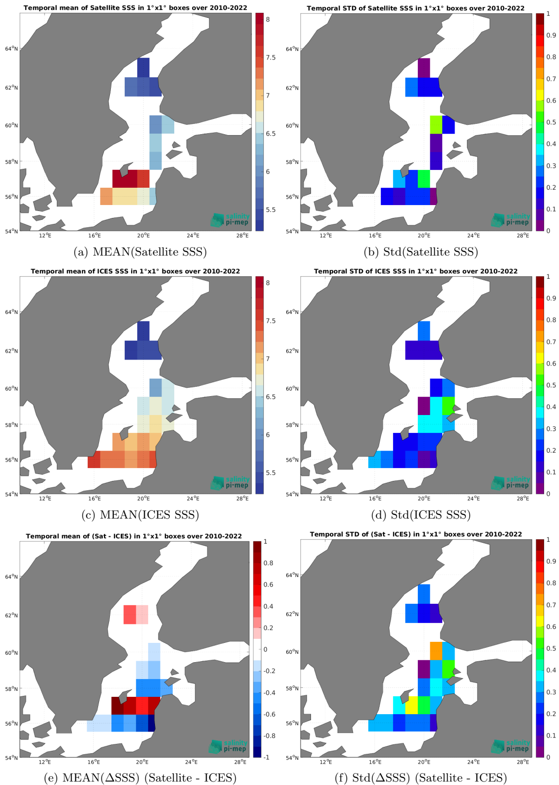
Figure 7: Temporal mean (left) and Std (right) of SSS from CCI SSS L4 Merged-OI v4.41 - 30-day running (ESA) (top), ICES (middle), and of \Delta SSS (Satellite - ICES). Only match-up pairs are used to generate these maps.
