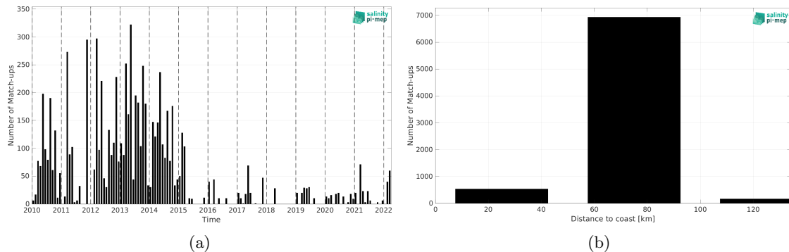
Figure 2: Number of match-ups between ICES and CCI SSS L4 Merged-OI v4.41 - 30-day running (ESA) SSS as a function of time (a) and as function of the distance to coast (b) over the Baltic Sea Pi-MEP region and for the full satellite product period.
