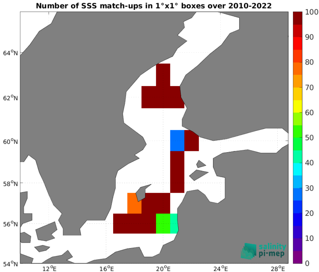
Figure 5: Number of SSS match-ups between ICES SSS and the CCI SSS L4 Merged-OI v4.41 - 30-day running (ESA) SSS product for the Baltic Sea Pi-MEP region over 1^\circ \times 1^\circ boxes and for the full satellite product period.
