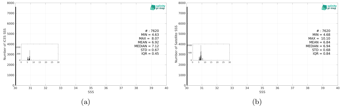
Figure 3: Histograms of SSS from ICES (a) and CCI SSS L4 Merged-OI v4.41 - 30-day running (ESA) (b) considering all match-up pairs per bins of 0.1 over the Baltic Sea Pi-MEP region and for the full satellite product period.
