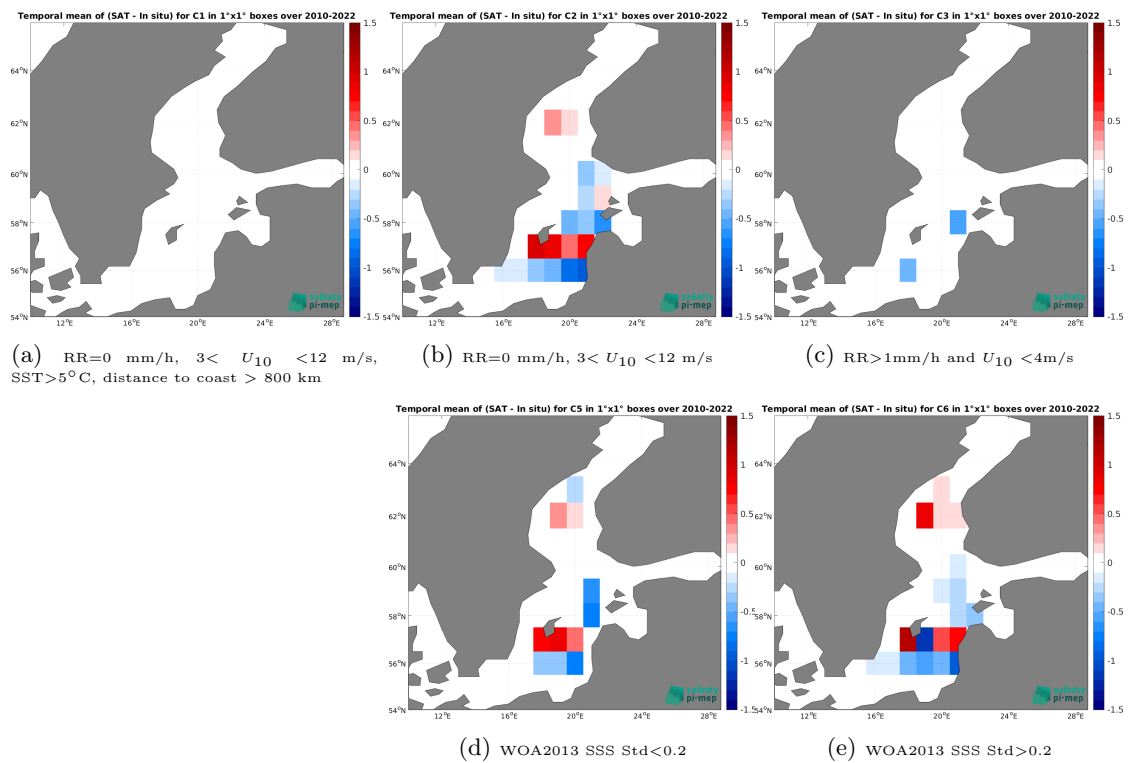
Figure 14: Temporal mean gridded over spatial boxes of size 1^\circ \times 1^\circ of \Delta SSS (CCI SSS L4 Merged-OI v4.41 - 30-day running (ESA) - ICES) for 5 different subdatasets corresponding to: RR=0 mm/h, 3 < U_{10} < 12 m/s, SST > 5^\circ\text{C} , distance to coast > 800 km (a), RR=0 mm/h, 3 < U_{10} < 12 m/s (b), RR > 1 mm/h and U_{10} < 4 m/s (c), WOA2013 SSS Std < 0.2 (d), WOA2013 SSS Std > 0.2 (e).
