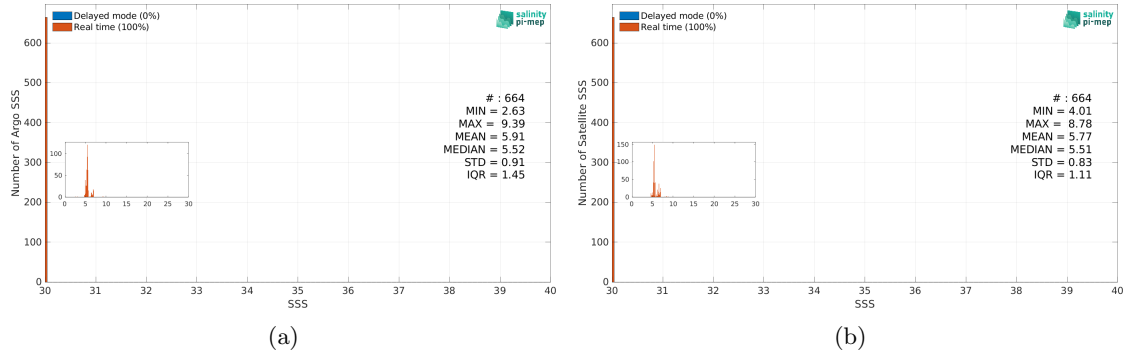
Figure 3: Histograms of SSS from Argo (a) and CCI SSS L4 Merged-OI v4.41 - 30-day running (ESA) (b) considering all match-up pairs per bins of 0.1 over the Baltic Sea Pi-MEP region and for the full satellite product period.
