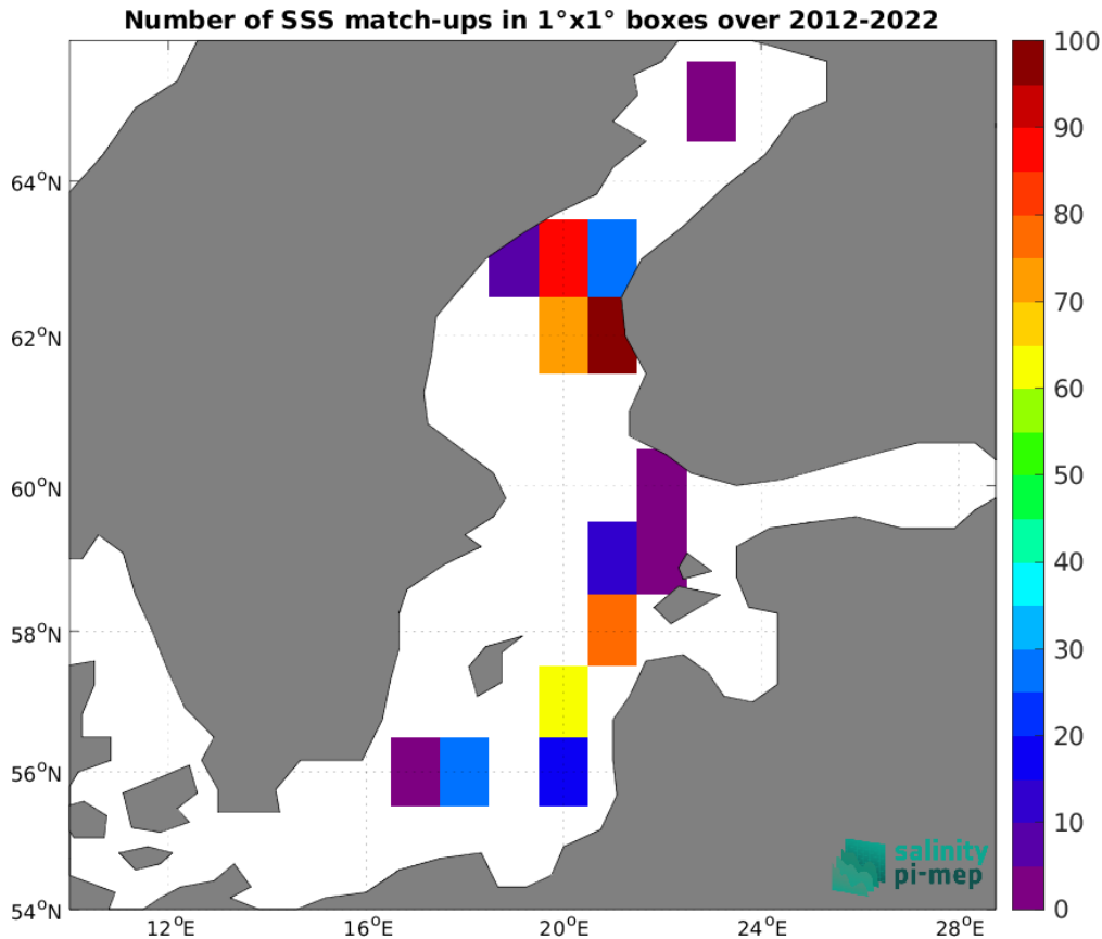
Figure 5: Number of SSS match-ups between Argo SSS and the CCI SSS L4 Merged-OI v4.41 - 30-day running (ESA) SSS product for the Baltic Sea Pi-MEP region over 1^\circ \times 1^\circ boxes and for the full satellite product period.
