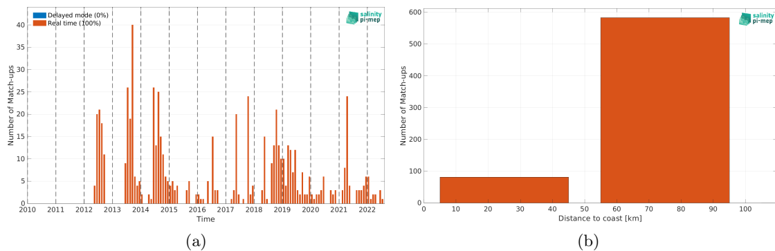
Figure 2: Number of match-ups between Argo and CCI SSS L4 Merged-OI v4.41 - 30-day running (ESA) SSS as a function of time (a) and as function of the distance to coast (b) over the Baltic Sea Pi-MEP region and for the full satellite product period.
