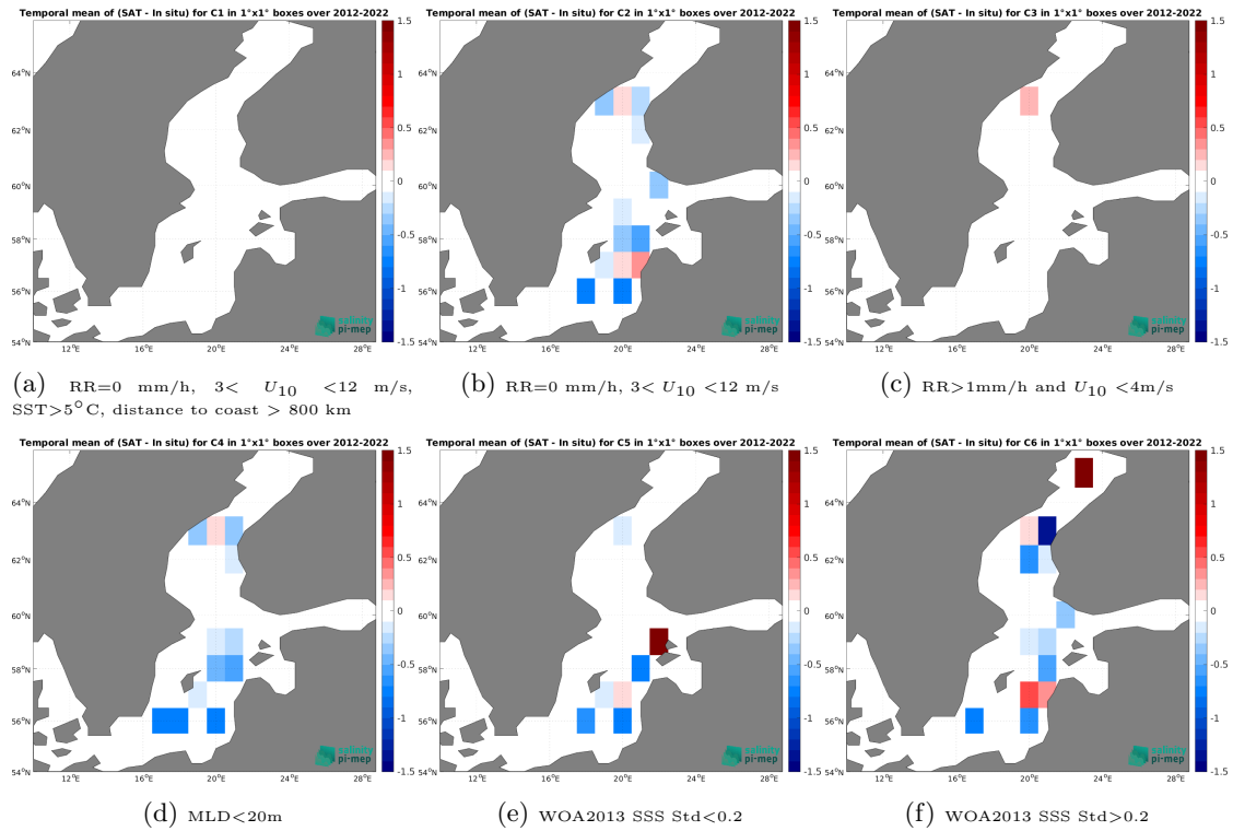
Figure 14: Temporal mean gridded over spatial boxes of size 1^\circ \times 1^\circ of \Delta\text{SSS} (CCI SSS L4 Merged-OI v4.41 - 30-day running (ESA) - Argo) for 6 different subdatasets corresponding to:RR=0 mm/h, 3 < U_{10} < 12 m/s, SST>5°C, distance to coast > 800 km (a), RR=0 mm/h, 3 < U_{10} < 12 m/s (b), RR>1mm/h and U_{10} < 4 m/s (c),MLD<20m (d),WOA2013 SSS Std<0.2 (e),WOA2013 SSS Std>0.2 (f).
