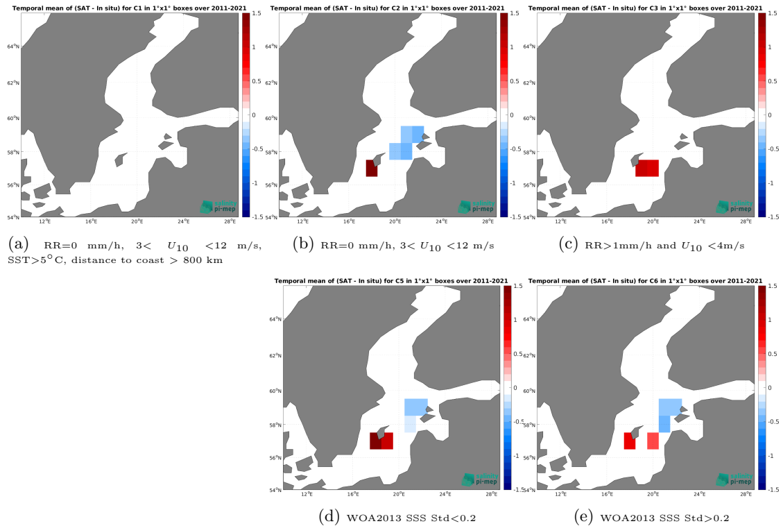
Figure 12: Temporal mean gridded over spatial boxes of size 1^{\circ}\times 1^{\circ} of \Delta\text{SSS} (CCI SSS L4 Merged-OI v4.4 - 7-day running (ESA) - TSG (LEGOS-DM)) for 5 different subdatasets corresponding to: RR=0 mm/h, 3 < U_{10} < 12 m/s, SST > 5^{\circ}\text{C} , distance to coast > 800 km (a), RR=0 mm/h, 3 < U_{10} < 12 m/s (b), RR > 1 mm/h and U_{10} < 4 m/s (c), WOA2013 SSS Std < 0.2 (d), WOA2013 SSS Std > 0.2 (e).
