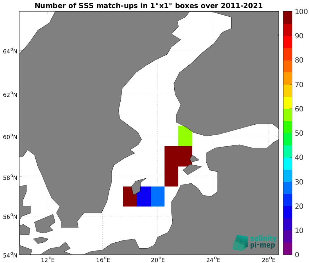
Figure 4: Number of SSS match-ups between TSG (LEGOS-DM) SSS and the CCI SSS L4 Merged-OI v4.4 - 7-day running (ESA) SSS product for the Baltic Sea Pi-MEP region over 1^\circ \times 1^\circ boxes and for the full satellite product period.
