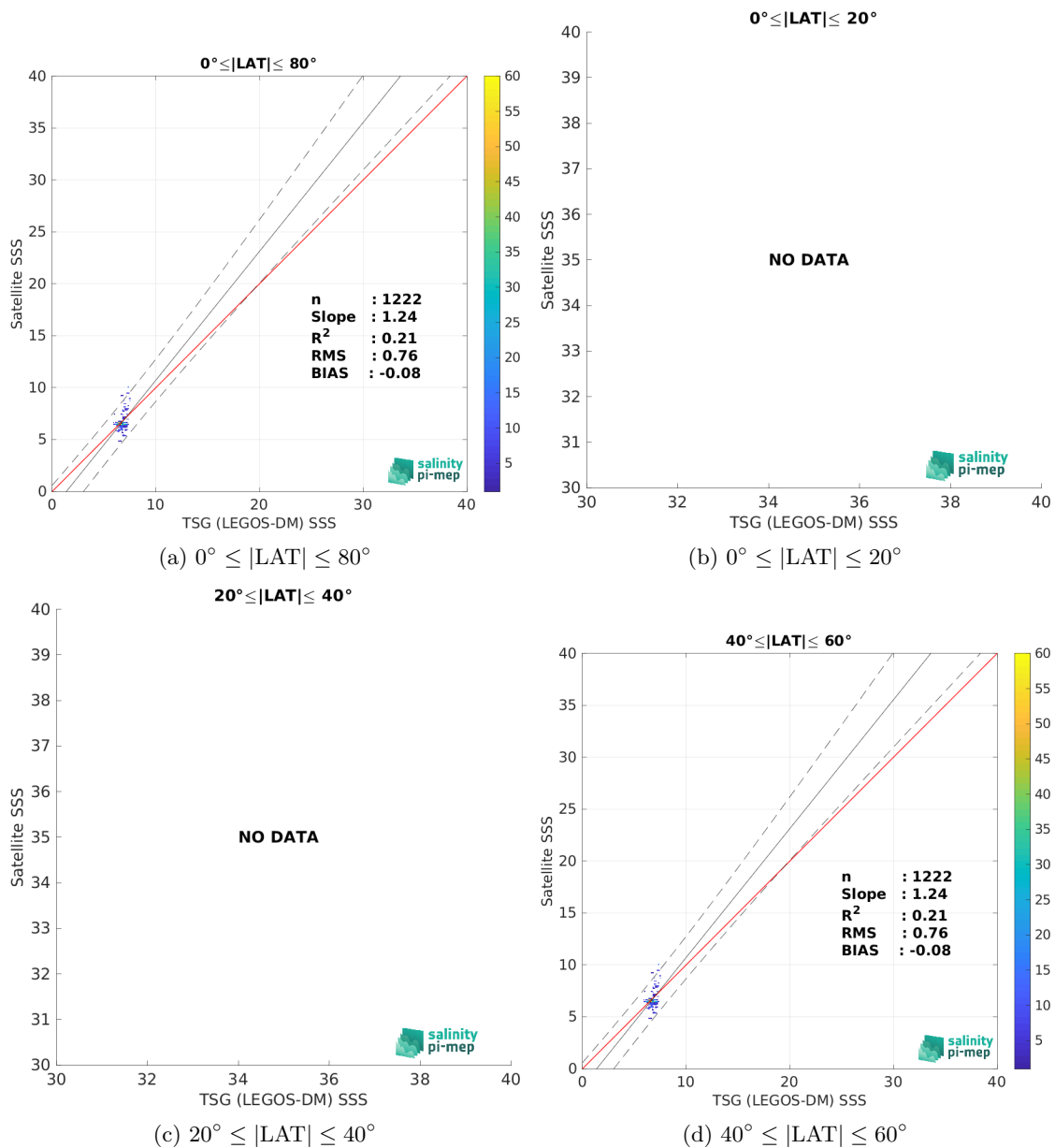
Figure 9: Contour maps of the concentration of CCI SSS L4 Merged-OI v4.4 - 7-day running (ESA) SSS (y-axis) versus TSG (LEGOS-DM) SSS (x-axis) at match-up pairs for different latitude bands. For each plot, the red line shows x=y . The black thin and dashed lines indicate a linear fit through the data cloud and the \pm 95\% confidence levels, respectively. The number match-up pairs n , the slope and R^2 coefficient of the linear fit, the root mean square (RMS) and the mean bias between satellite and in situ data are indicated for each latitude band in each plots.
