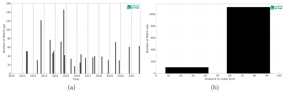
Figure 1: Number of match-ups between TSG (LEGOS-DM) and CCI SSS L4 Merged-OI v4.4 - 7-day running (ESA) SSS as a function of time (a) and as function of the distance to coast (b) over the Baltic Sea Pi-MEP region and for the full satellite product period.
