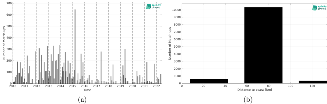
Figure 1: Number of match-ups between ICES and CCI SSS L4 Merged-OI v4.4 - 7-day running (ESA) SSS as a function of time (a) and as function of the distance to coast (b) over the Baltic Sea Pi-MEP region and for the full satellite product period.
