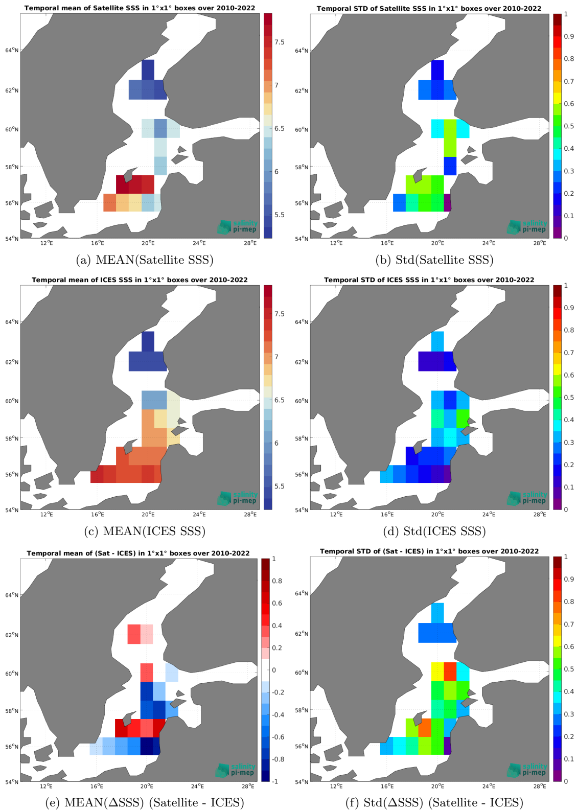
Figure 6: Temporal mean (left) and Std (right) of SSS from CCI SSS L4 Merged-OI v4.4 - 7-day running (ESA) (top), ICES (middle), and of \Delta SSS (Satellite - ICES). Only match-up pairs are used to generate these maps.
