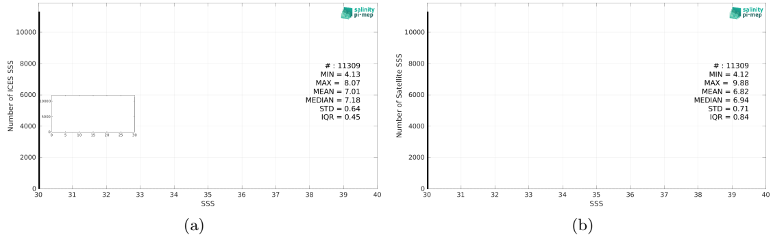
Figure 2: Histograms of SSS from ICES (a) and CCI SSS L4 Merged-OI v4.4 - 7-day running (ESA) (b) considering all match-up pairs per bins of 0.1 over the Baltic Sea Pi-MEP region and for the full satellite product period.
