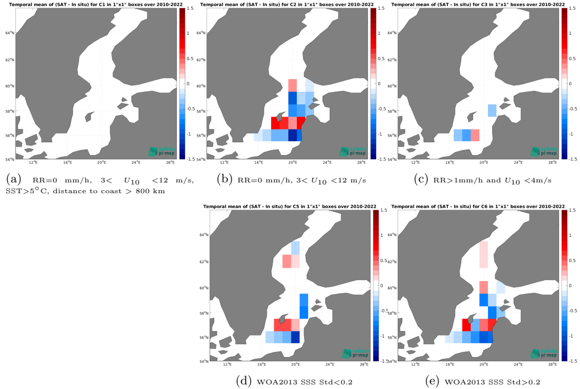
Figure 12: Temporal mean gridded over spatial boxes of size 1^{\circ}\times 1^{\circ} of \Delta\text{SSS} (CCI SSS L4 Merged-OI v4.4 - 7-day running (ESA) - ICES) for 5 different subdatasets corresponding to:RR=0 mm/h, 3 < U_{10} < 12 m/s, SST >5^{\circ}\text{C} , distance to coast > 800 km (a), RR=0 mm/h, 3 < U_{10} < 12 m/s (b), RR >1 mm/h and U_{10} < 4 m/s (c), WOA2013 SSS Std <0.2 (d), WOA2013 SSS Std >0.2 (e).
