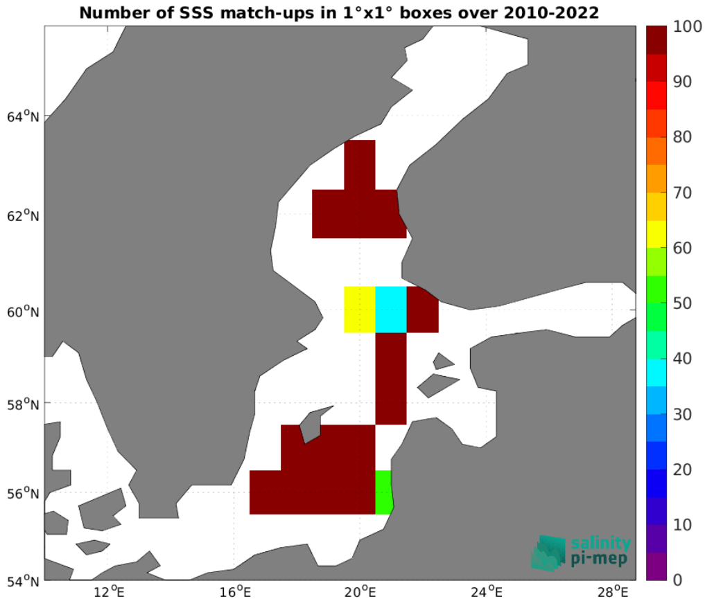
Figure 4: Number of SSS match-ups between ICES SSS and the CCI SSS L4 Merged-OI v4.4 - 7-day running (ESA) SSS product for the Baltic Sea Pi-MEP region over 1^\circ \times 1^\circ boxes and for the full satellite product period.
