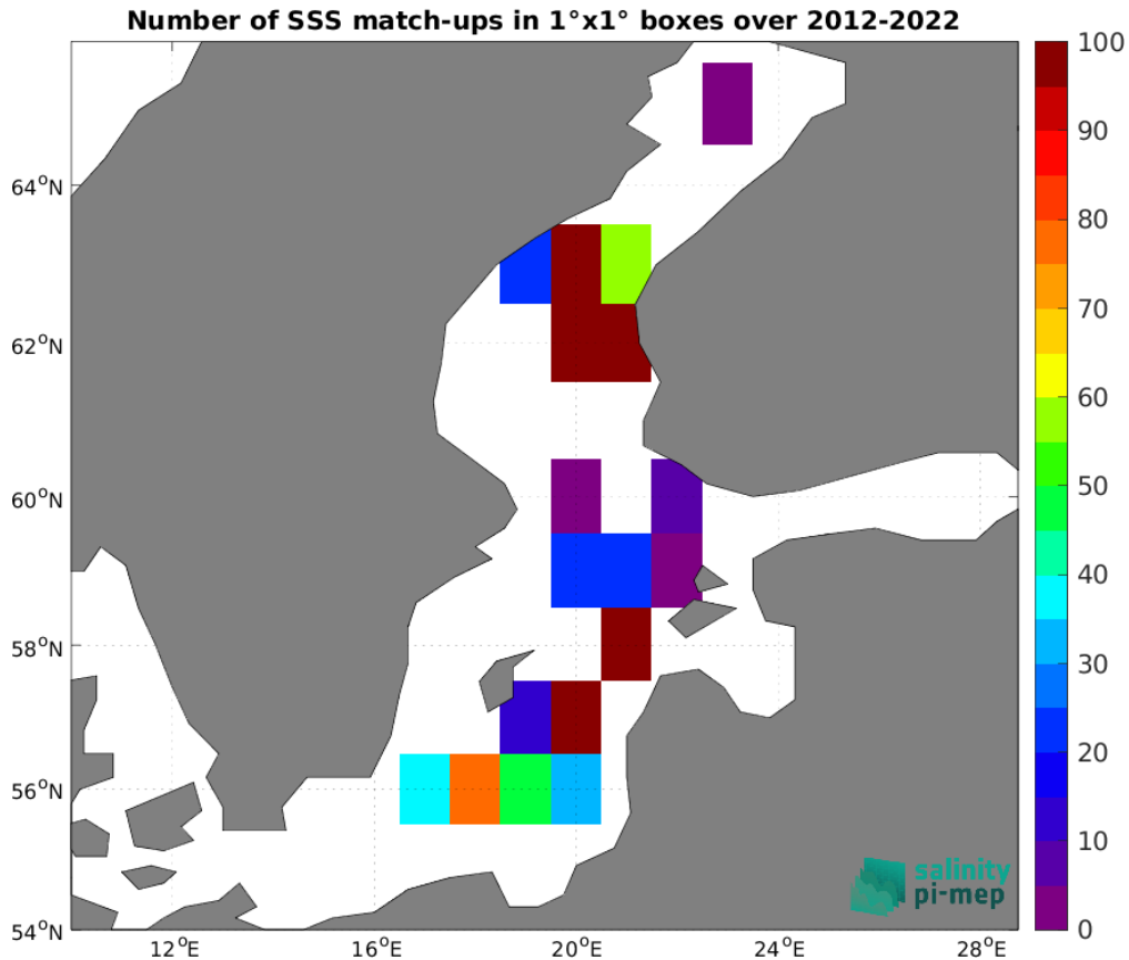
Figure 4: Number of SSS match-ups between Argo SSS and the CCI SSS L4 Merged-OI v4.4 - 7-day running (ESA) SSS product for the Baltic Sea Pi-MEP region over 1^\circ \times 1^\circ boxes and for the full satellite product period.
