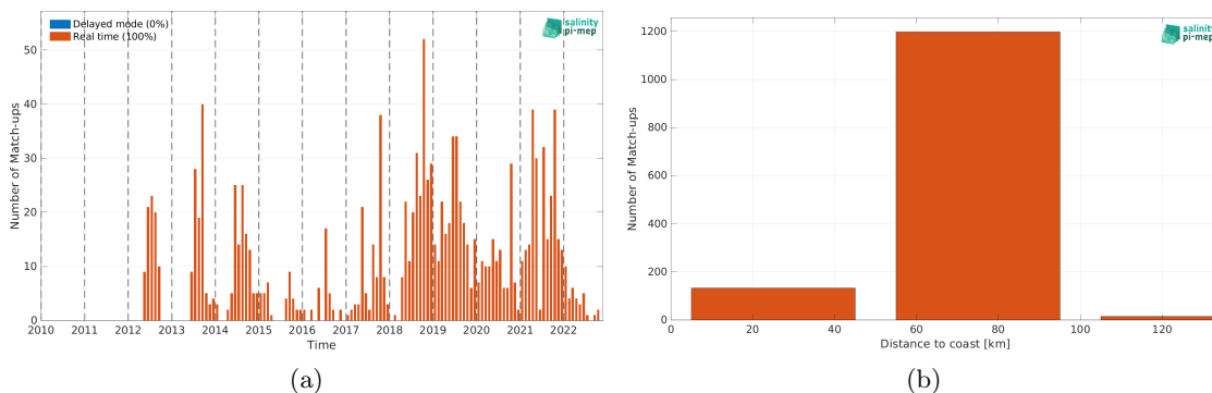
Figure 1: Number of match-ups between Argo and CCI SSS L4 Merged-OI v4.4 - 7-day running (ESA) SSS as a function of time (a) and as function of the distance to coast (b) over the Baltic Sea Pi-MEP region and for the full satellite product period.
