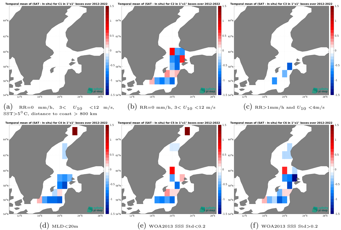
Figure 12: Temporal mean gridded over spatial boxes of size 1^{\circ}\times 1^{\circ} of \Delta\text{SSS} (CCI SSS L4 Merged-OI v4.4 - 7-day running (ESA) - Argo) for 6 different subdatasets corresponding to:RR=0 mm/h, 3 < U_{10} < 12 m/s, SST >5^{\circ}\text{C} , distance to coast > 800 km (a), RR=0 mm/h, 3 < U_{10} < 12 m/s (b), RR >1\text{mm/h} and U_{10} < 4\text{m/s} (c),MLD <20\text{m} (d),WOA2013 SSS Std <0.2 (e),WOA2013 SSS Std >0.2 (f).
