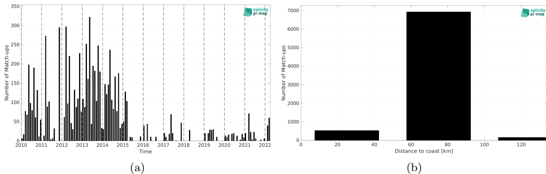
Figure 1: Number of match-ups between ICES and CCI SSS L4 Merged-OI v4.4 - 30-day running (ESA) SSS as a function of time (a) and as function of the distance to coast (b) over the Baltic Sea Pi-MEP region and for the full satellite product period.
