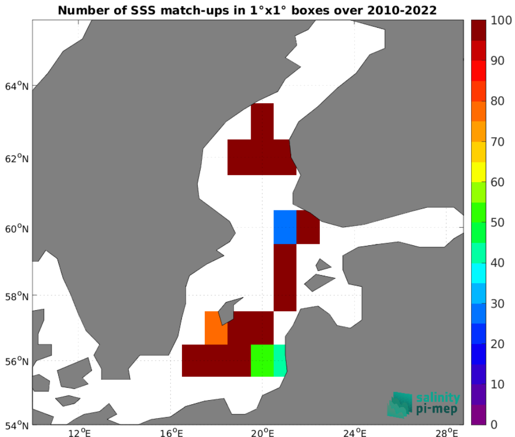
Figure 4: Number of SSS match-ups between ICES SSS and the CCI SSS L4 Merged-OI v4.4 - 30-day running (ESA) SSS product for the Baltic Sea Pi-MEP region over 1°×1° boxes and for the full satellite product period.
