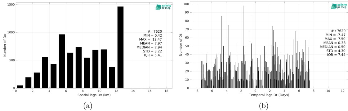
Figure 5: Histograms of the spatial (a) and temporal (b) lags between the location/time of the ICES measurement and the date of the corresponding CCI SSS L4 Merged-OI v4.4 - 30-day running (ESA) SSS pixel.
