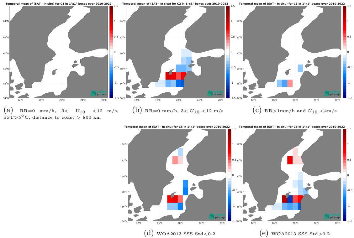
Figure 12: Temporal mean gridded over spatial boxes of size 1^{\circ}\times 1^{\circ} of \Delta\text{SSS} (CCI SSS L4 Merged-OI v4.4 - 30-day running (ESA) - ICES) for 5 different subdatasets corresponding to:RR=0 mm/h, 3 < U_{10} < 12 m/s, SST > 5^{\circ}\text{C} , distance to coast > 800 km (a), RR=0 mm/h, 3 < U_{10} < 12 m/s (b), RR > 1 mm/h and U_{10} < 4 m/s (c), WOA2013 SSS Std < 0.2 (d), WOA2013 SSS Std > 0.2 (e).
