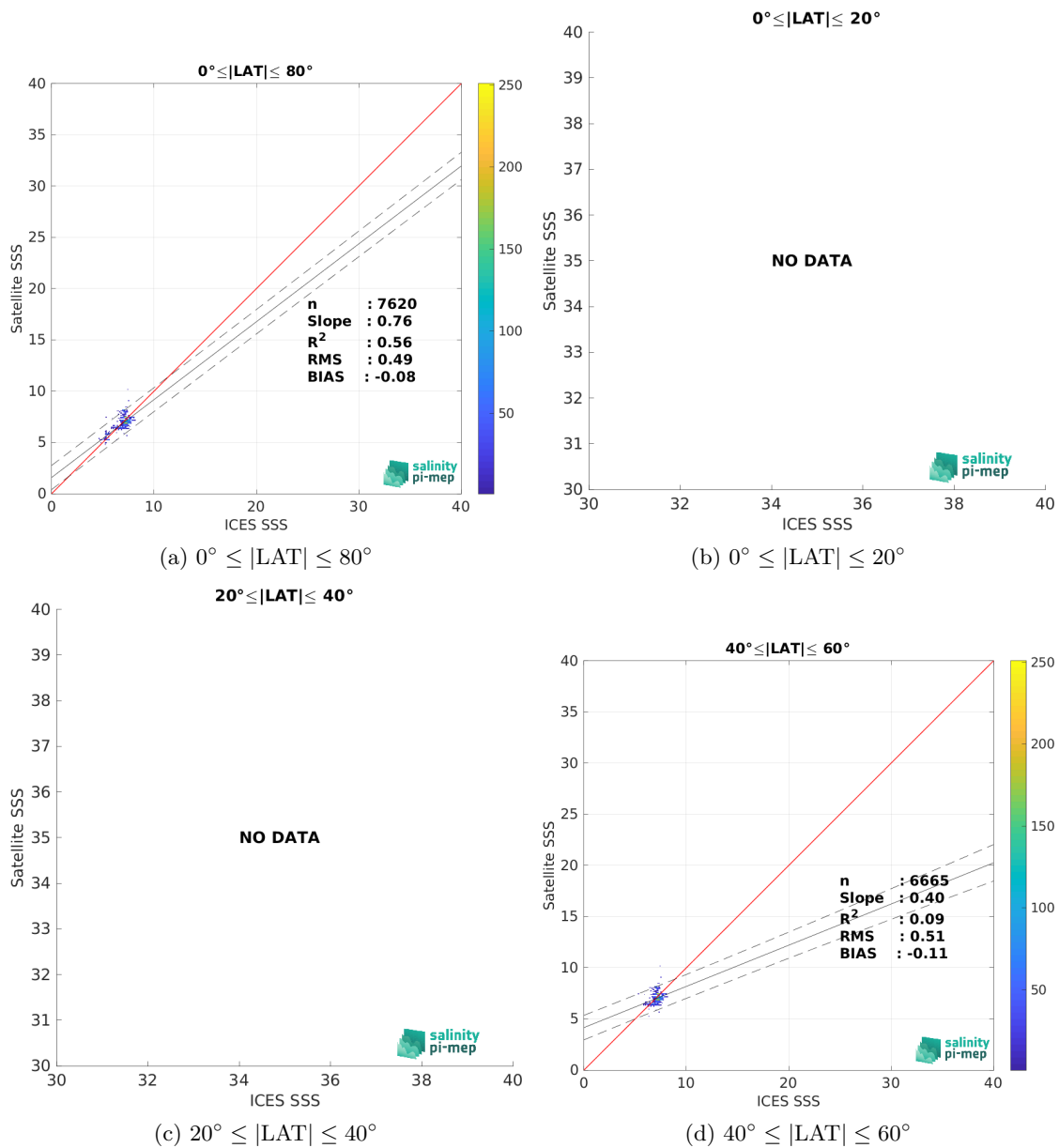
Figure 9: Contour maps of the concentration of CCI SSS L4 Merged-OI v4.4 - 30-day running (ESA) SSS (y-axis) versus ICES SSS (x-axis) at match-up pairs for different latitude bands. For each plot, the red line shows x=y . The black thin and dashed lines indicate a linear fit through the data cloud and the \pm 95\% confidence levels, respectively. The number match-up pairs n , the slope and R^2 coefficient of the linear fit, the root mean square (RMS) and the mean bias between satellite and in situ data are indicated for each latitude band in each plots.
