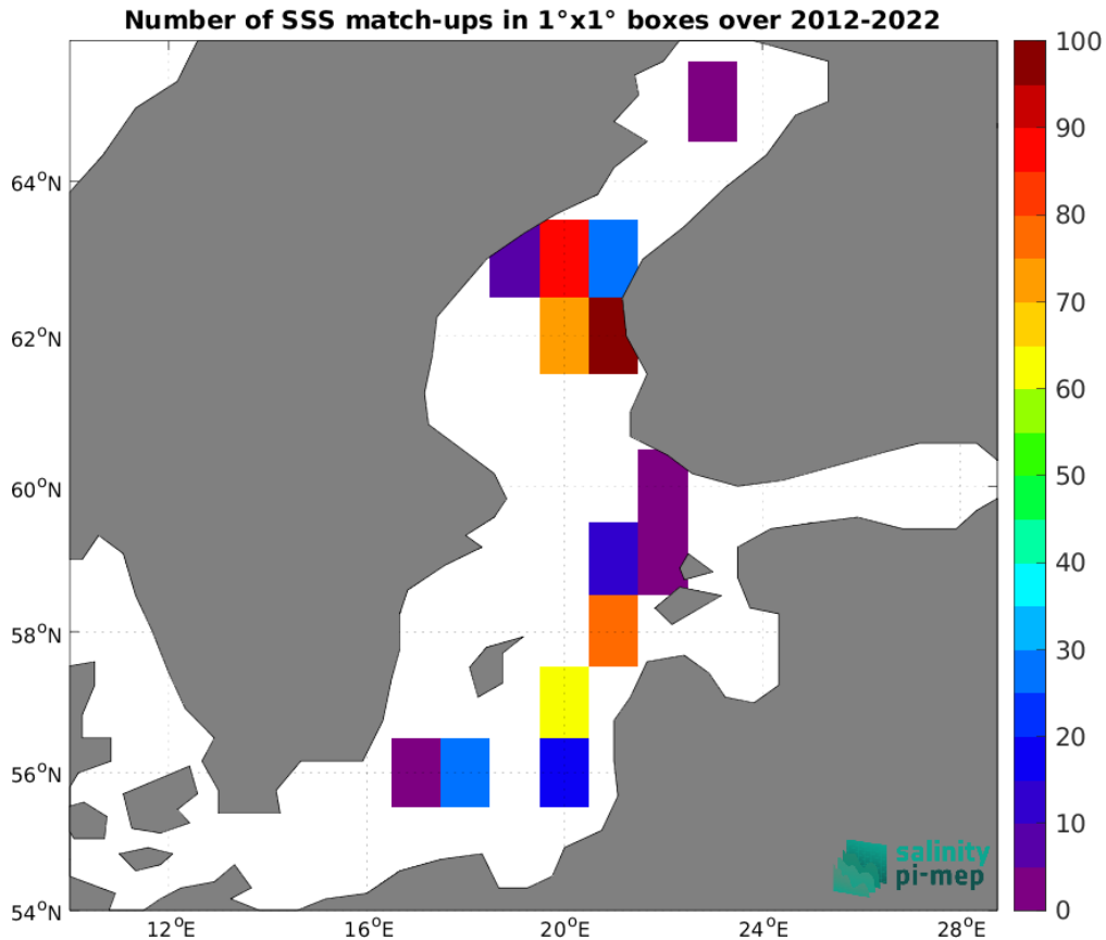
Figure 4: Number of SSS match-ups between Argo SSS and the CCI SSS L4 Merged-OI v4.4 - 30-day running (ESA) SSS product for the Baltic Sea Pi-MEP region over 1^\circ \times 1^\circ boxes and for the full satellite product period.
