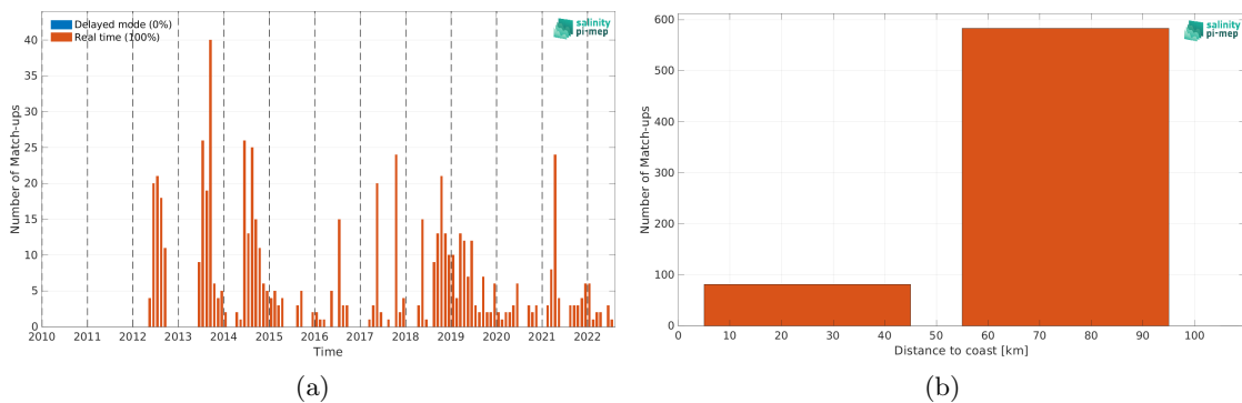
Figure 1: Number of match-ups between Argo and CCI SSS L4 Merged-OI v4.4 - 30-day running (ESA) SSS as a function of time (a) and as function of the distance to coast (b) over the Baltic Sea Pi-MEP region and for the full satellite product period.
