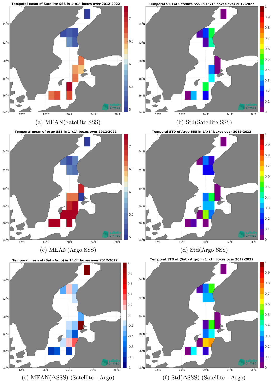
Figure 6: Temporal mean (left) and Std (right) of SSS from CCI SSS L4 Merged-OI v4.4 - 30-day running (ESA) (top), Argo (middle), and of \Delta SSS (Satellite - Argo). Only match-up pairs are used to generate these maps.
