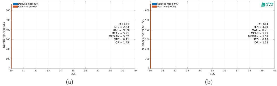
Figure 2: Histograms of SSS from Argo (a) and CCI SSS L4 Merged-OI v4.4 - 30-day running (ESA) (b) considering all match-up pairs per bins of 0.1 over the Baltic Sea Pi-MEP region and for the full satellite product period.
