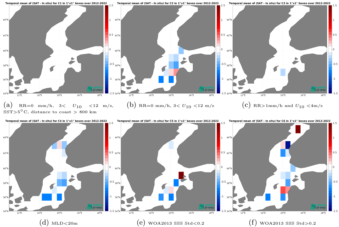
Figure 12: Temporal mean gridded over spatial boxes of size 1^{\circ}\times 1^{\circ} of \Delta\text{SSS} (CCI SSS L4 Merged-OI v4.4 - 30-day running (ESA) - Argo) for 6 different subdatasets corresponding to:RR=0 mm/h, 3 < U_{10} < 12 m/s, SST >5^{\circ}\text{C} , distance to coast > 800 km (a), RR=0 mm/h, 3 < U_{10} < 12 m/s (b), RR >1\text{mm/h} and U_{10} < 4\text{m/s} (c),MLD <20\text{m} (d),WOA2013 SSS Std <0.2 (e),WOA2013 SSS Std >0.2 (f).
