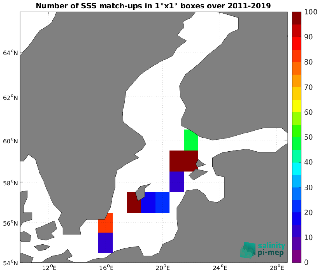
Figure 4: Number of SSS match-ups between TSG (LEGOS-DM) SSS and the CCI SSS L4 Merged-OI v3.2 - 7-day running (ESA) SSS product for the Baltic Sea Pi-MEP region over 1^\circ \times 1^\circ boxes and for the full satellite product period.
