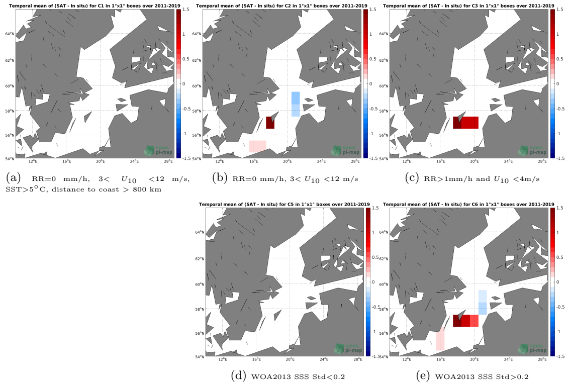
Figure 12: Temporal mean gridded over spatial boxes of size 1^{\circ}\times 1^{\circ} of \Delta\text{SSS} (CCI SSS L4 Merged-OI v3.2 - 7-day running (ESA) - TSG (LEGOS-DM)) for 5 different subdatasets corresponding to:RR=0 mm/h, 3 < U_{10} < 12 m/s, SST >5^{\circ}\text{C} , distance to coast > 800 km (a), RR=0 mm/h, 3 < U_{10} < 12 m/s (b), RR >1 mm/h and U_{10} < 4 m/s (c), WOA2013 SSS Std <0.2 (d), WOA2013 SSS Std >0.2 (e).
