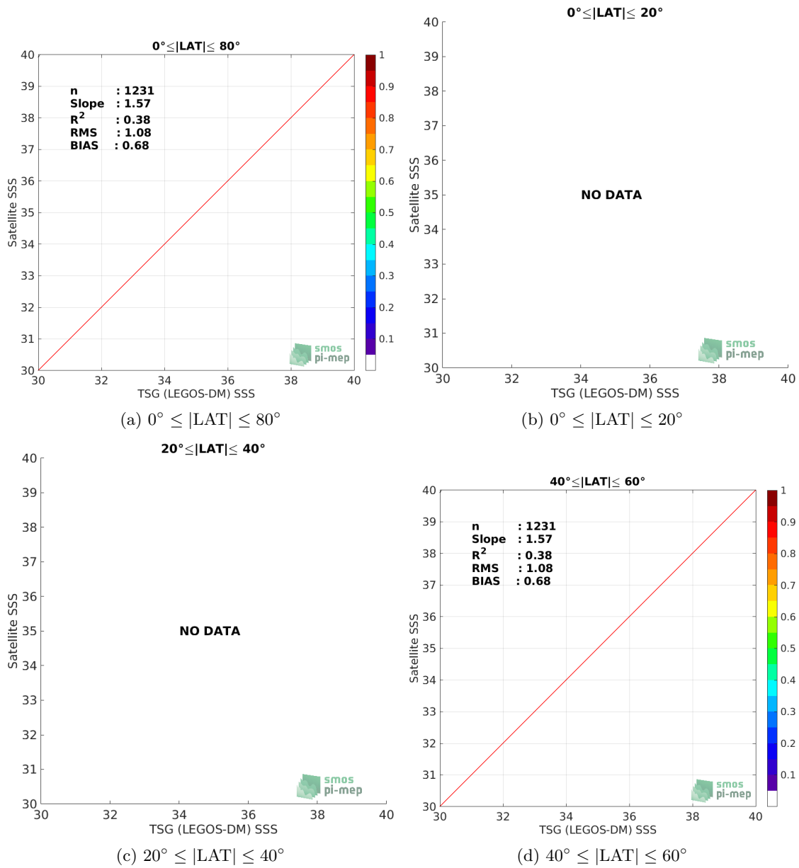
Figure 9: Contour maps of the concentration of CCI SSS L4 Merged-OI v3.2 - 7-day running (ESA) SSS (y-axis) versus TSG (LEGOS-DM) SSS (x-axis) at match-up pairs for different latitude bands. For each plot, the red line shows x=y . The black thin and dashed lines indicate a linear fit through the data cloud and the \pm 95\% confidence levels, respectively. The number match-up pairs n , the slope and R^2 coefficient of the linear fit, the root mean square (RMS) and the mean bias between satellite and in situ data are indicated for each latitude band in each plots.
