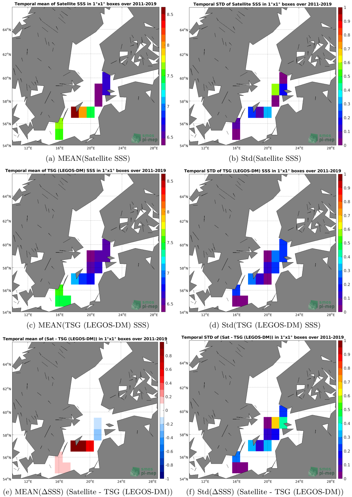
Figure 6: Temporal mean (left) and Std (right) of SSS from CCI SSS L4 Merged-OI v3.2 - 7-day running (ESA) (top), TSG (LEGOS-DM) (middle), and of \Delta SSS (Satellite - TSG (LEGOS-DM)). Only match-up pairs are used to generate these maps.
