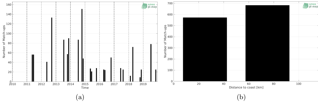
Figure 1: Number of match-ups between TSG (LEGOS-DM) and CCI SSS L4 Merged-OI v3.2 - 7-day running (ESA) SSS as a function of time (a) and as function of the distance to coast (b) over the Baltic Sea Pi-MEP region and for the full satellite product period.
