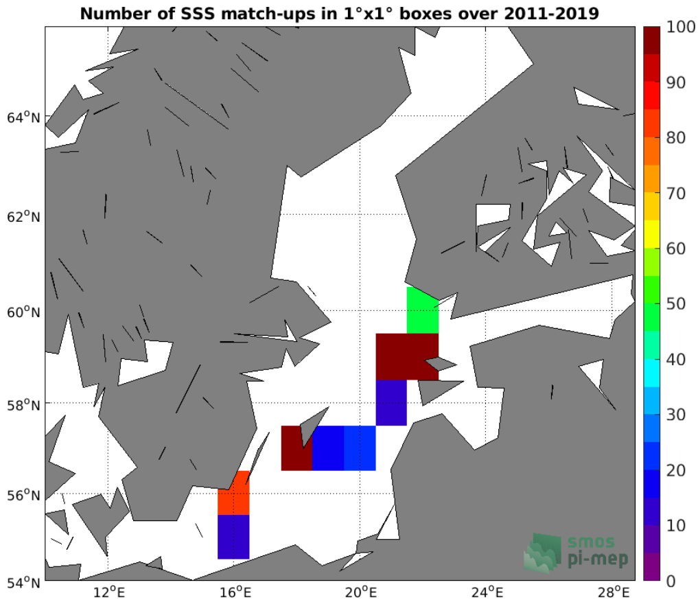
Figure 4: Number of SSS match-ups between TSG (LEGOS-DM) SSS and the CCI SSS L4 Merged-OI v3.2 - 7-day running (ESA) SSS product for the Baltic Sea Pi-MEP region over 1°x1° boxes and for the full satellite product period.
