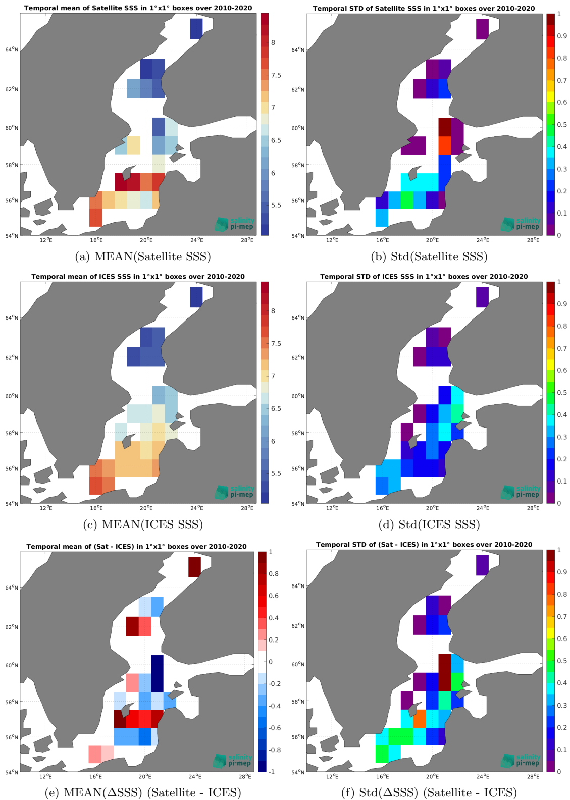
Figure 6: Temporal mean (left) and Std (right) of SSS from CCI SSS L4 Merged-OI v3.2 - 7-day running (ESA) (top), ICES (middle), and of \Delta SSS (Satellite - ICES). Only match-up pairs are used to generate these maps.
