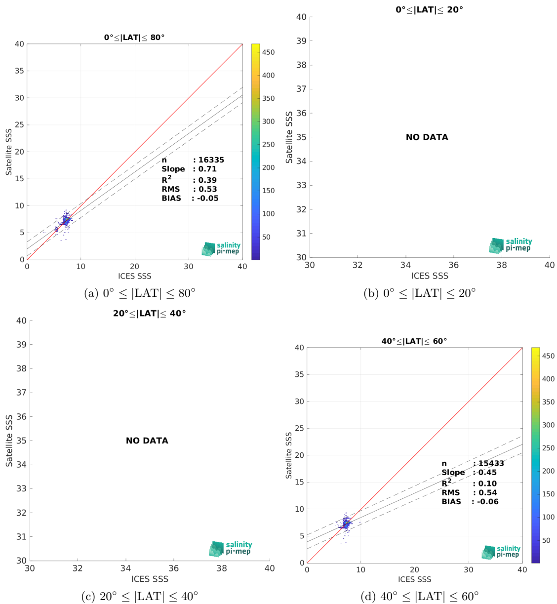
Figure 9: Contour maps of the concentration of CCI SSS L4 Merged-OI v3.2 - 7-day running (ESA) SSS (y-axis) versus ICES SSS (x-axis) at match-up pairs for different latitude bands. For each plot, the red line shows x=y . The black thin and dashed lines indicate a linear fit through the data cloud and the \pm 95\% confidence levels, respectively. The number match-up pairs n , the slope and R^2 coefficient of the linear fit, the root mean square (RMS) and the mean bias between satellite and in situ data are indicated for each latitude band in each plots.
