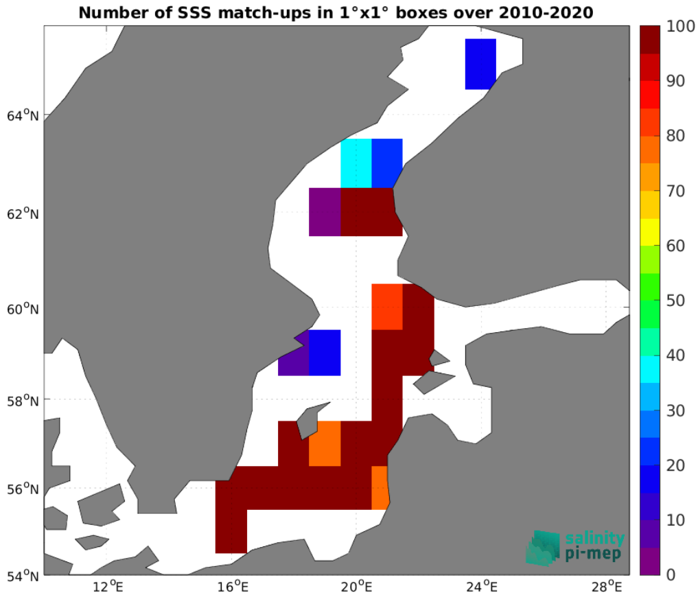
Figure 4: Number of SSS match-ups between ICES SSS and the CCI SSS L4 Merged-OI v3.2 - 7-day running (ESA) SSS product for the Baltic Sea Pi-MEP region over 1^\circ \times 1^\circ boxes and for the full satellite product period.
