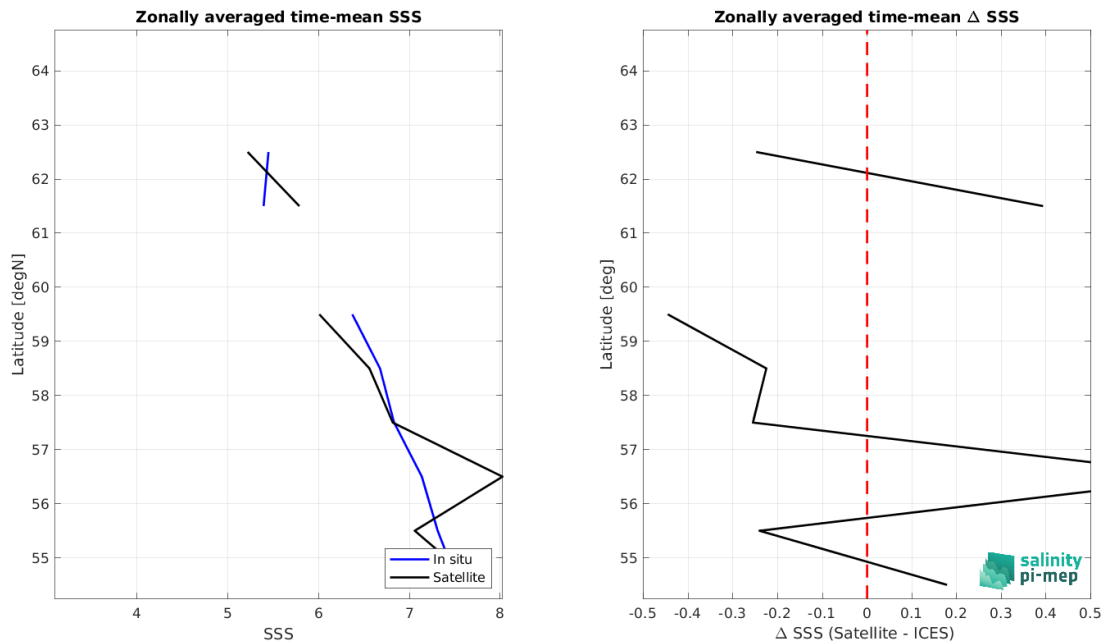
Figure 8: Left panel: Zonal mean SSS from CCI SSS L4 Merged-OI v3.2 - 7-day running (ESA) satellite product (black) and from ICES (blue). Right panel: Zonal mean of \Delta SSS (Satellite - ICES) for all the collected Pi-MEP match-up pairs estimated over the full satellite product period.
