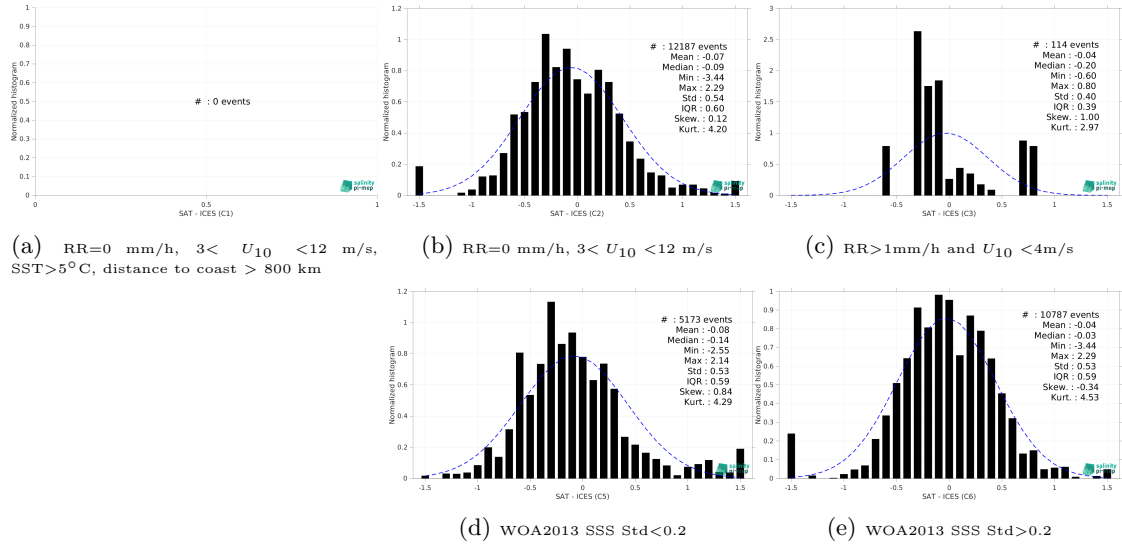
Figure 13: Normalized histogram of \Delta SSS (CCI SSS L4 Merged-OI v3.2 - 7-day running (ESA) - ICES) for 5 different subdatasets corresponding to: RR=0 mm/h, 3 < U_{10} < 12 m/s, SST > 5°C, distance to coast > 800 km (a), RR=0 mm/h, 3 < U_{10} < 12 m/s (b), RR > 1mm/h and U_{10} < 4 m/s (c), WOA2013 SSS Std < 0.2 (d), WOA2013 SSS Std > 0.2 (e).
