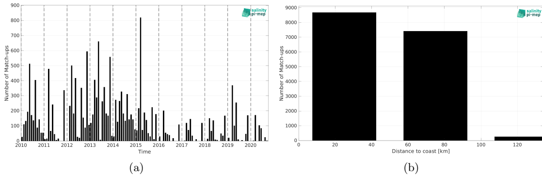
Figure 1: Number of match-ups between ICES and CCI SSS L4 Merged-OI v3.2 - 7-day running (ESA) SSS as a function of time (a) and as function of the distance to coast (b) over the Baltic Sea Pi-MEP region and for the full satellite product period.
