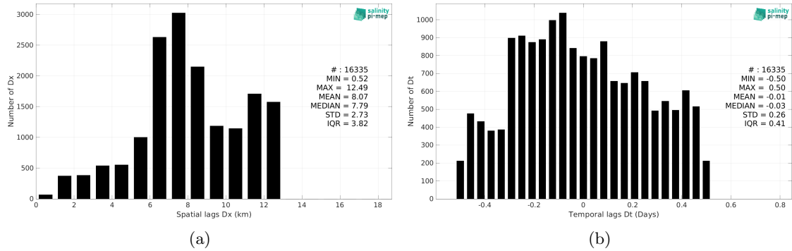
Figure 5: Histograms of the spatial (a) and temporal (b) lags between the location/time of the ICES measurement and the date of the corresponding CCI SSS L4 Merged-OI v3.2 - 7-day running (ESA) SSS pixel.
