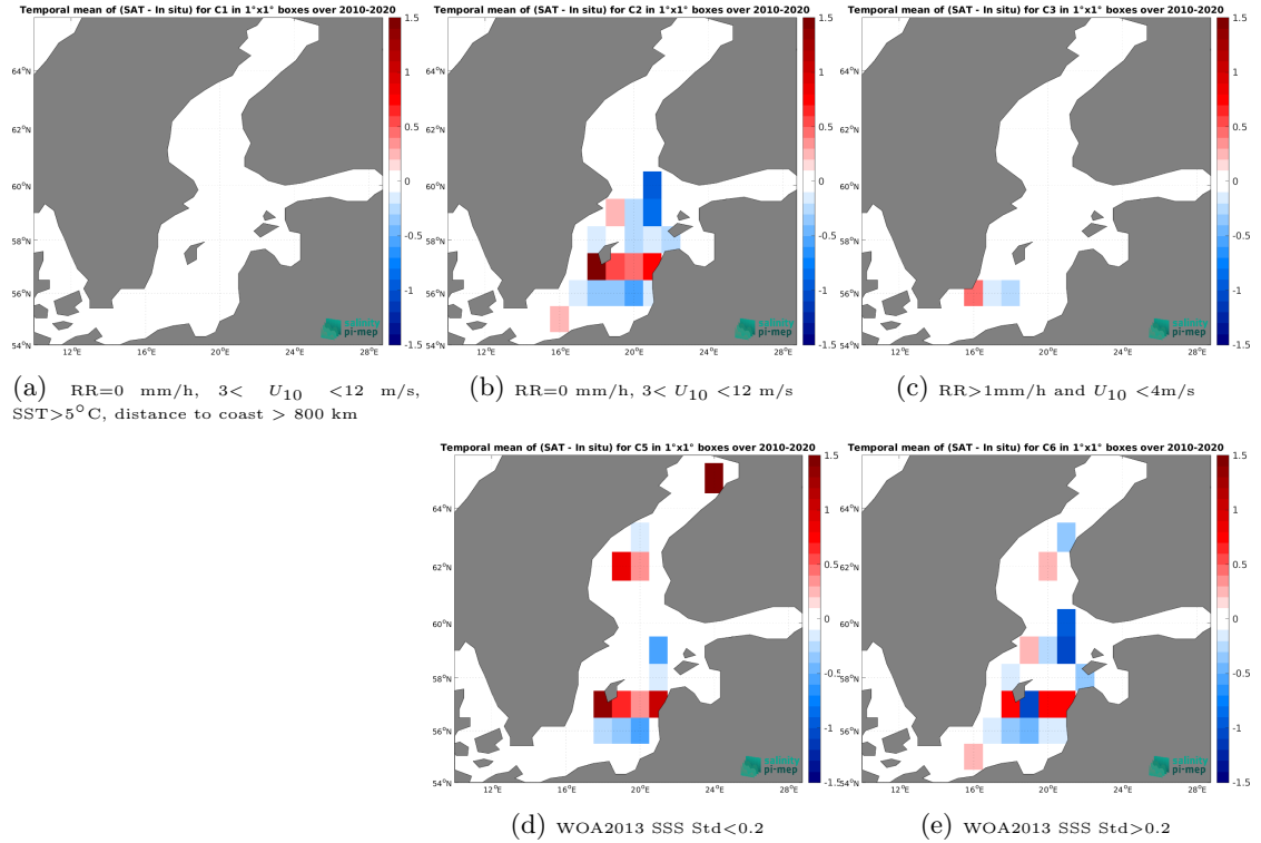
Figure 12: Temporal mean gridded over spatial boxes of size 1^{\circ}\times 1^{\circ} of \Delta\text{SSS} (CCI SSS L4 Merged-OI v3.2 - 7-day running (ESA) - ICES) for 5 different subdatasets corresponding to:RR=0 mm/h, 3 < U_{10} < 12 m/s, SST >5^{\circ}\text{C} , distance to coast > 800 km (a), RR=0 mm/h, 3 < U_{10} < 12 m/s (b), RR >1 mm/h and U_{10} < 4 m/s (c), WOA2013 SSS Std <0.2 (d), WOA2013 SSS Std >0.2 (e).
