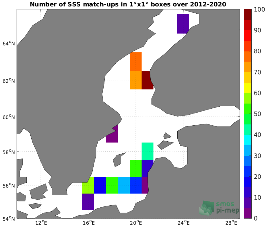
Figure 4: Number of SSS match-ups between Argo SSS and the CCI SSS L4 Merged-OI v3.2 - 7-day running (ESA) SSS product for the Baltic Sea Pi-MEP region over 1^\circ \times 1^\circ boxes and for the full satellite product period.
