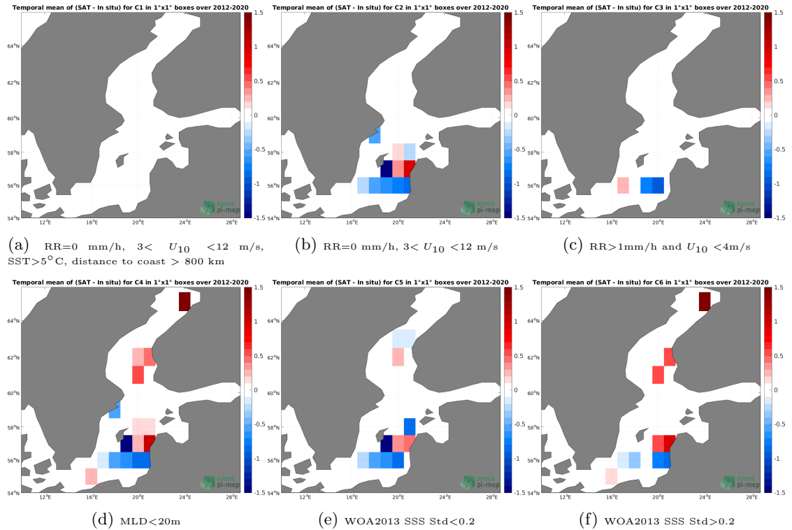
Figure 12: Temporal mean gridded over spatial boxes of size 1^{\circ}\times 1^{\circ} of \Delta\text{SSS} (CCI SSS L4 Merged-OI v3.2 - 7-day running (ESA) - Argo) for 6 different subdatasets corresponding to:RR=0 mm/h, 3 < U_{10} < 12 m/s, SST >5^{\circ}\text{C} , distance to coast > 800 km (a), RR=0 mm/h, 3 < U_{10} < 12 m/s (b), RR >1 mm/h and U_{10} < 4 m/s (c),MLD <20 m (d),WOA2013 SSS Std <0.2 (e),WOA2013 SSS Std >0.2 (f).
