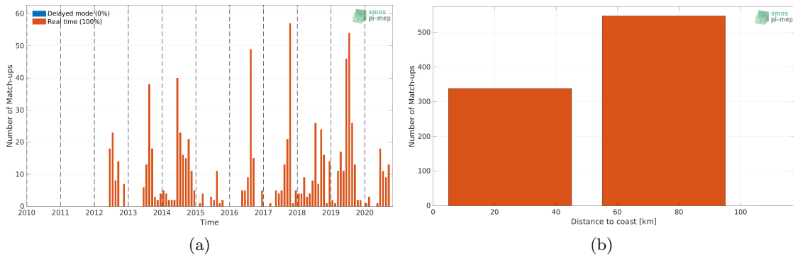
Figure 1: Number of match-ups between Argo and CCI SSS L4 Merged-OI v3.2 - 7-day running (ESA) SSS as a function of time (a) and as function of the distance to coast (b) over the Baltic Sea Pi-MEP region and for the full satellite product period.
