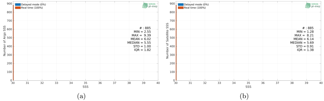
Figure 2: Histograms of SSS from Argo (a) and CCI SSS L4 Merged-OI v3.2 - 7-day running (ESA) (b) considering all match-up pairs per bins of 0.1 over the Baltic Sea Pi-MEP region and for the full satellite product period.
