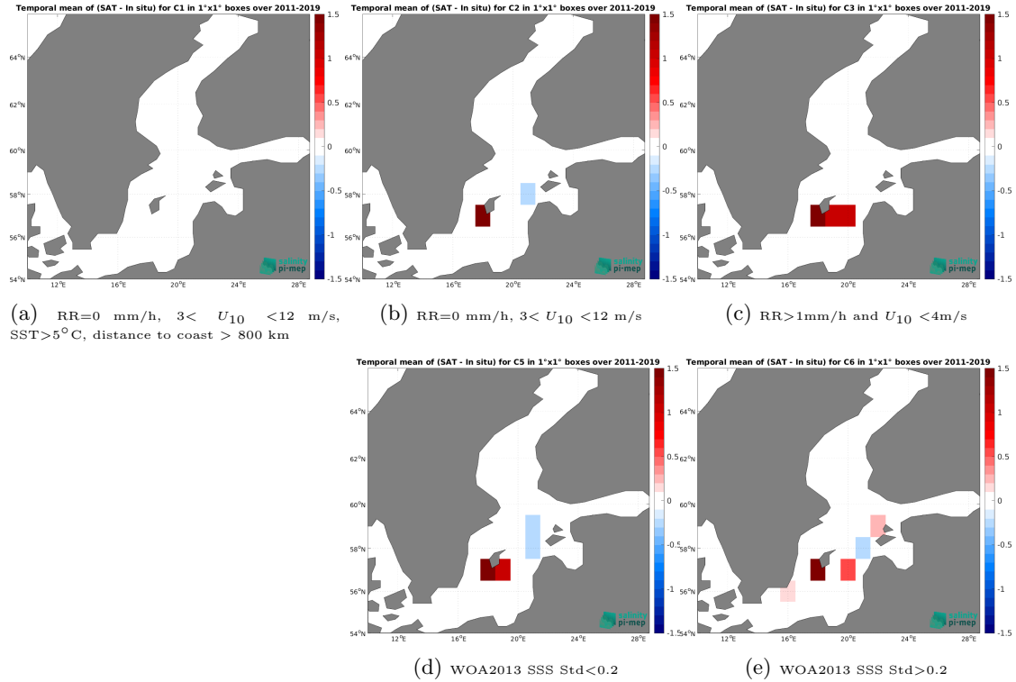
Figure 12: Temporal mean gridded over spatial boxes of size 1^{\circ}\times 1^{\circ} of \Delta\text{SSS} (CCI SSS L4 Merged-OI v3.2 - 30-day running (ESA) - TSG (LEGOS-DM)) for 5 different subdatasets corresponding to:RR=0 mm/h, 3 < U_{10} < 12 m/s, SST >5^{\circ}\text{C} , distance to coast > 800 km (a), RR=0 mm/h, 3 < U_{10} < 12 m/s (b), RR >1 mm/h and U_{10} < 4 m/s (c), WOA2013 SSS Std <0.2 (d), WOA2013 SSS Std >0.2 (e).
