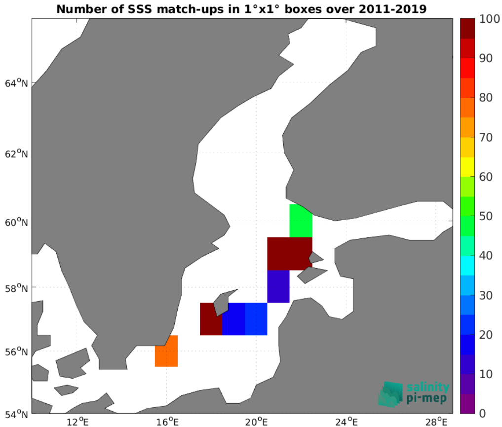
Figure 4: Number of SSS match-ups between TSG (LEGOS-DM) SSS and the CCI SSS L4 Merged-OI v3.2 - 30-day running (ESA) SSS product for the Baltic Sea Pi-MEP region over 1^\circ \times 1^\circ boxes and for the full satellite product period.
