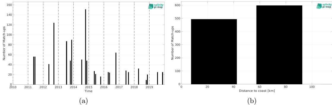
Figure 1: Number of match-ups between TSG (LEGOS-DM) and CCI SSS L4 Merged-OI v3.2 - 30-day running (ESA) SSS as a function of time (a) and as function of the distance to coast (b) over the Baltic Sea Pi-MEP region and for the full satellite product period.
