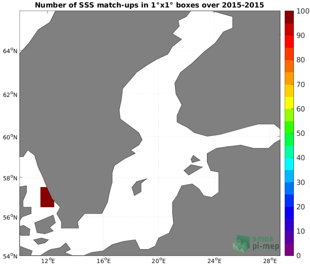
Figure 4: Number of SSS match-ups between TSG (GOSUD-Research-vessel) SSS and the CCI SSS L4 Merged-OI v3.2 - 30-day running (ESA) SSS product for the Baltic Sea Pi-MEP region over 1^\circ \times 1^\circ boxes and for the full satellite product period.
