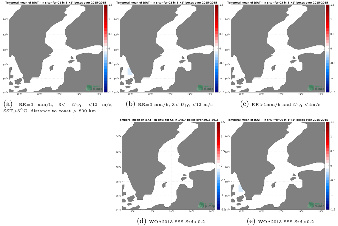
Figure 12: Temporal mean gridded over spatial boxes of size 1^{\circ}\times 1^{\circ} of \Delta SSS (CCI SSS L4 Merged-OI v3.2 - 30-day running (ESA) - TSG (GOSUD-Research-vessel)) for 5 different subdatasets corresponding to:RR=0 mm/h, 3 < U_{10} < 12 m/s, SST >5^{\circ}\text{C} , distance to coast > 800 km (a), RR=0 mm/h, 3 < U_{10} < 12 m/s (b), RR >1 mm/h and U_{10} < 4 m/s (c), WOA2013 SSS Std <0.2 (d), WOA2013 SSS Std >0.2 (e).
