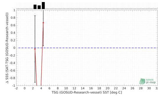
(b) TSG (GOSUD-Research-vessel) SST
