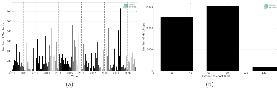
Figure 1: Number of match-ups between ICES and CCI SSS L4 Merged-OI v3.2 - 30-day running (ESA) SSS as a function of time (a) and as function of the distance to coast (b) over the Baltic Sea Pi-MEP region and for the full satellite product period.
