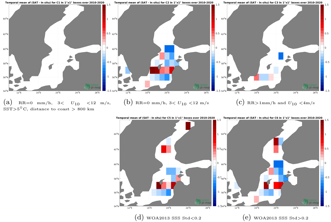
Figure 12: Temporal mean gridded over spatial boxes of size 1^{\circ}\times 1^{\circ} of \Delta\text{SSS} (CCI SSS L4 Merged-OI v3.2 - 30-day running (ESA) - ICES) for 5 different subdatasets corresponding to:RR=0 mm/h, 3 < U_{10} < 12 m/s, SST >5^{\circ}\text{C} , distance to coast > 800 km (a), RR=0 mm/h, 3 < U_{10} < 12 m/s (b), RR >1 mm/h and U_{10} < 4 m/s (c), WOA2013 SSS Std <0.2 (d), WOA2013 SSS Std >0.2 (e).
