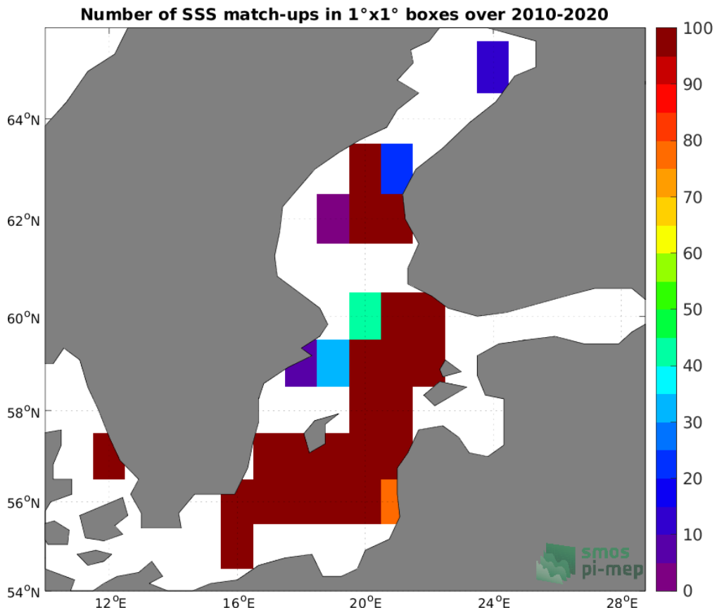
Figure 4: Number of SSS match-ups between ICES SSS and the CCI SSS L4 Merged-OI v3.2 - 30-day running (ESA) SSS product for the Baltic Sea Pi-MEP region over 1°×1° boxes and for the full satellite product period.
