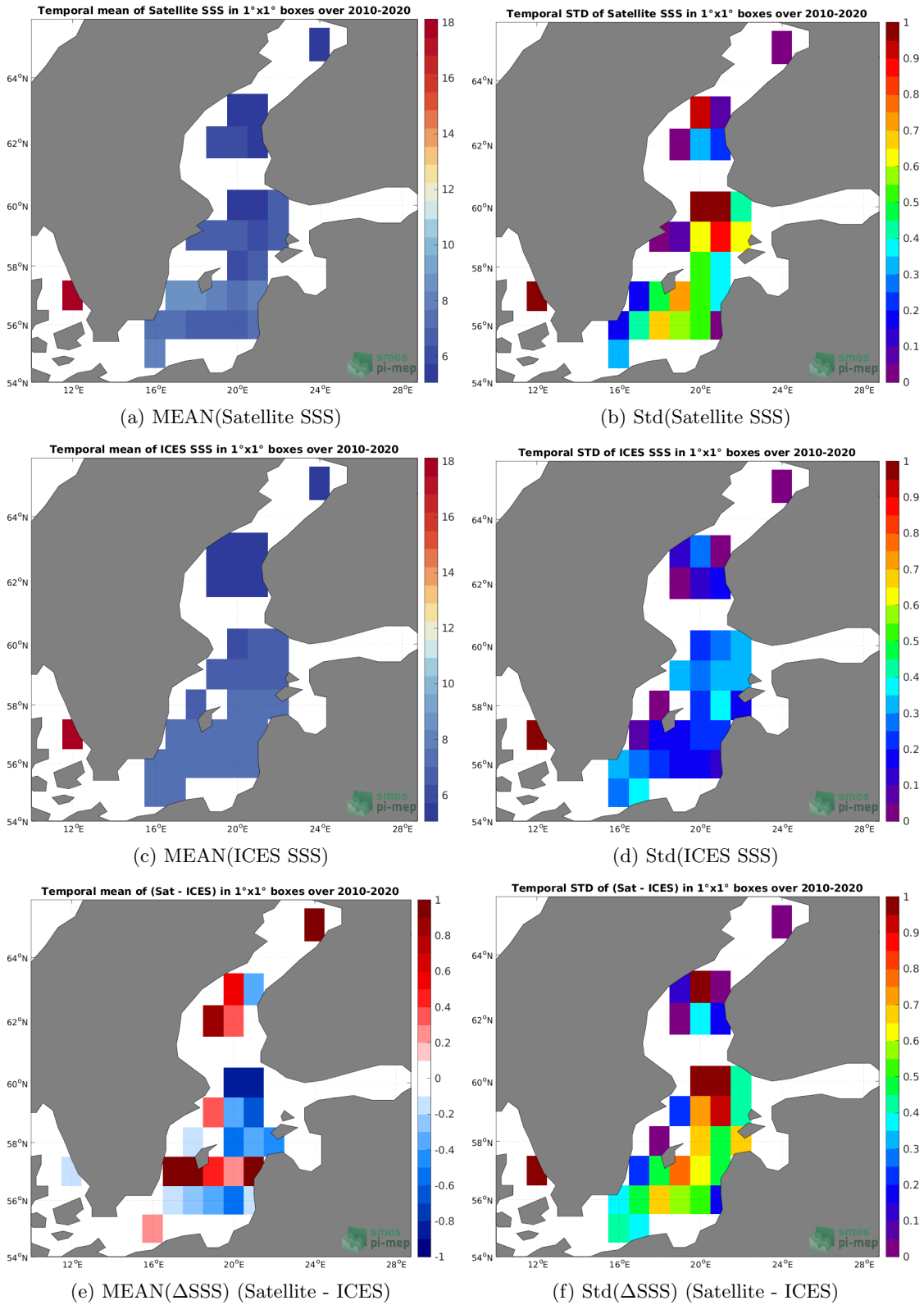
Figure 6: Temporal mean (left) and Std (right) of SSS from CCI SSS L4 Merged-OI v3.2 - 30-day running (ESA) (top), ICES (middle), and of \Delta SSS (Satellite - ICES). Only match-up pairs are used to generate these maps.
