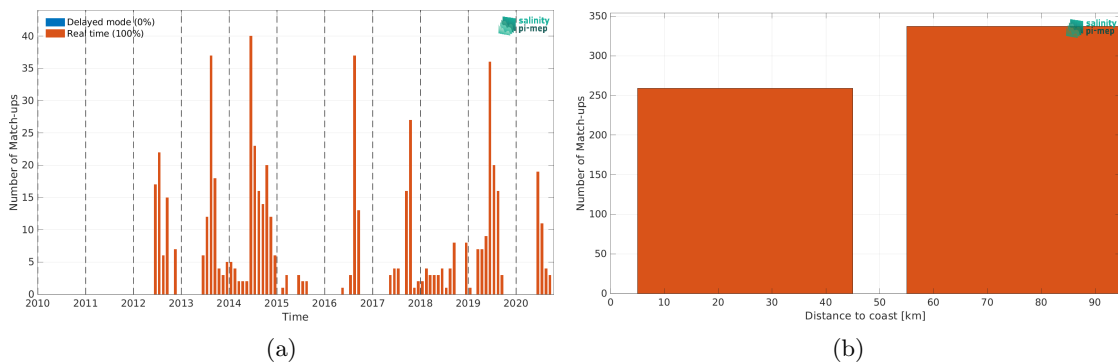
Figure 1: Number of match-ups between Argo and CCI SSS L4 Merged-OI v3.2 - 30-day running (ESA) SSS as a function of time (a) and as function of the distance to coast (b) over the Baltic Sea Pi-MEP region and for the full satellite product period.
