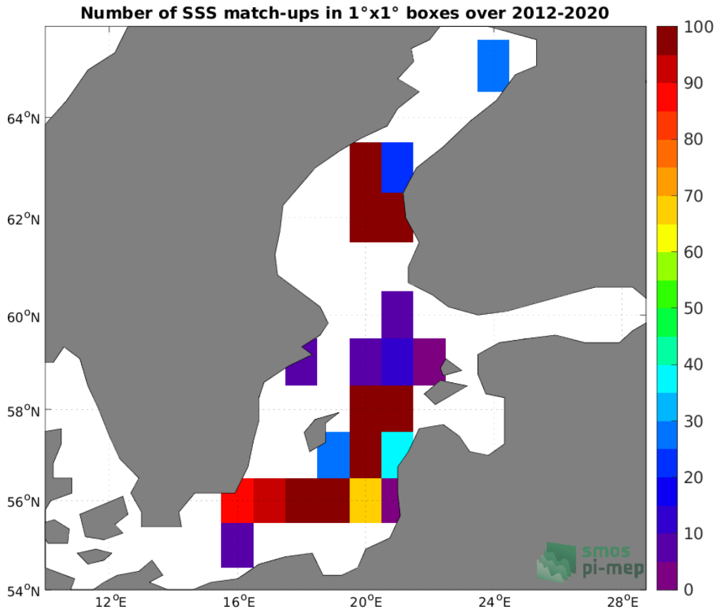
Figure 4: Number of SSS match-ups between Argo SSS and the CCI SSS L4 Merged-OI v3.2 - 30-day running (ESA) SSS product for the Baltic Sea Pi-MEP region over 1^\circ \times 1^\circ boxes and for the full satellite product period.
