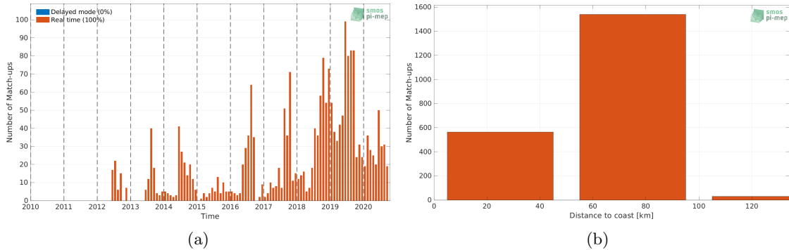
Figure 1: Number of match-ups between Argo and CCI SSS L4 Merged-OI v3.2 - 30-day running (ESA) SSS as a function of time (a) and as function of the distance to coast (b) over the Baltic Sea Pi-MEP region and for the full satellite product period.
