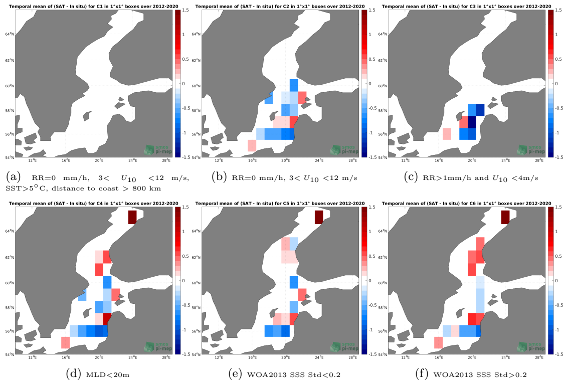
Figure 12: Temporal mean gridded over spatial boxes of size 1^{\circ}\times 1^{\circ} of \Delta\text{SSS} (CCI SSS L4 Merged-OI v3.2 - 30-day running (ESA) - Argo) for 6 different subdatasets corresponding to:RR=0 mm/h, 3 < U_{10} < 12 m/s, SST >5^{\circ}\text{C} , distance to coast > 800 km (a), RR=0 mm/h, 3 < U_{10} < 12 m/s (b), RR >1 mm/h and U_{10} < 4 m/s (c),MLD <20 m (d),WOA2013 SSS Std <0.2 (e),WOA2013 SSS Std >0.2 (f).
