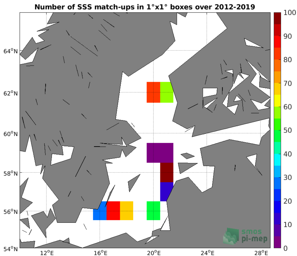
Figure 4: Number of SSS match-ups between Argo SSS and the CCI SSS L4 Merged-OI v2.31 - 7-day running (ESA) SSS product for the Baltic Sea Pi-MEP region over 1°x1° boxes and for the full satellite product period.
