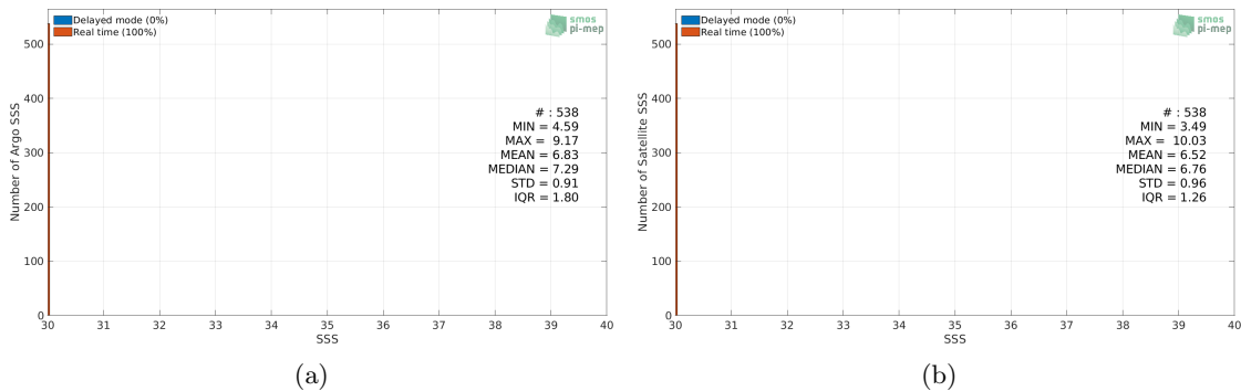
Figure 2: Histograms of SSS from Argo (a) and CCI SSS L4 Merged-OI v2.31 - 7-day running (ESA) (b) considering all match-up pairs per bins of 0.1 over the Baltic Sea Pi-MEP region and for the full satellite product period.
