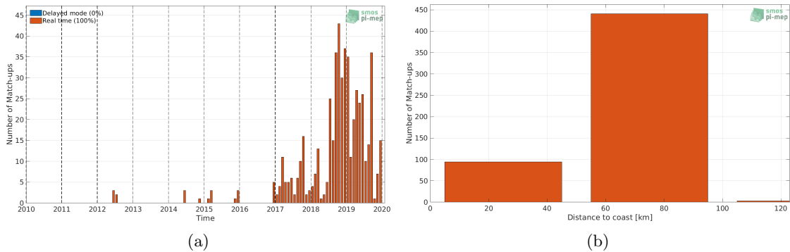
Figure 1: Number of match-ups between Argo and CCI SSS L4 Merged-OI v2.31 - 7-day running (ESA) SSS as a function of time (a) and as function of the distance to coast (b) over the Baltic Sea Pi-MEP region and for the full satellite product period.
