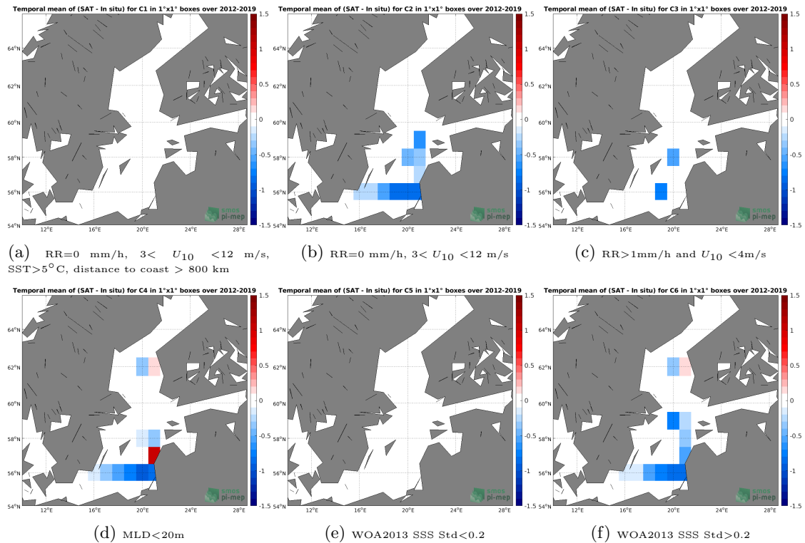
Figure 12: Temporal mean gridded over spatial boxes of size 1^{\circ}\times 1^{\circ} of \Delta\text{SSS} (CCI SSS L4 Merged-OI v2.31 - 7-day running (ESA) - Argo) for 6 different subdatasets corresponding to:RR=0 mm/h, 3 < U_{10} < 12 m/s, SST >5^{\circ}\text{C} , distance to coast > 800 km (a), RR=0 mm/h, 3 < U_{10} < 12 m/s (b), RR >1 mm/h and U_{10} < 4 m/s (c),MLD <20 m (d),WOA2013 SSS Std <0.2 (e),WOA2013 SSS Std >0.2 (f).
