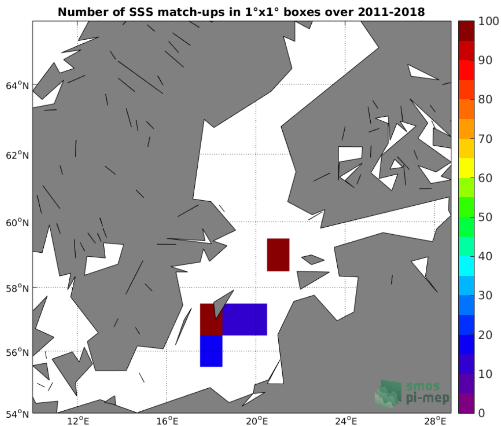
Figure 4: Number of SSS match-ups between TSG-LEGOS-DM SSS and the CCI L4 Merged-OI v1.8 - 7-day running (ESA) SSS product for the Baltic Sea Pi-MEP region over 1°x1° boxes and for the full satellite product period.
