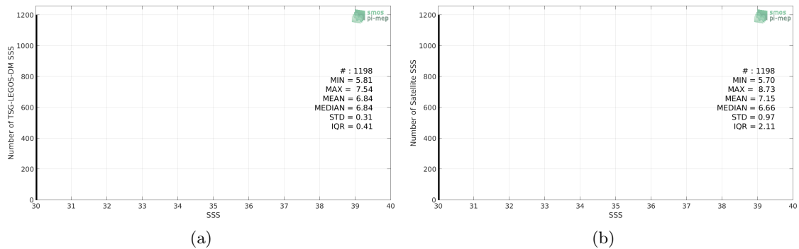
Figure 2: Histograms of SSS from TSG-LEGOS-DM (a) and CCI L4 Merged-OI v1.8 - 7-day running (ESA) (b) considering all match-up pairs per bins of 0.1 over the Baltic Sea Pi-MEP region and for the full satellite product period.
