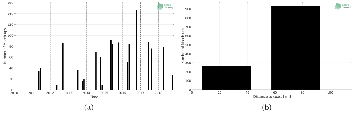
Figure 1: Number of match-ups between TSG-LEGOS-DM and CCI L4 Merged-OI v1.8 - 7-day running (ESA) SSS as a function of time (a) and as function of the distance to coast (b) over the Baltic Sea Pi-MEP region and for the full satellite product period.
