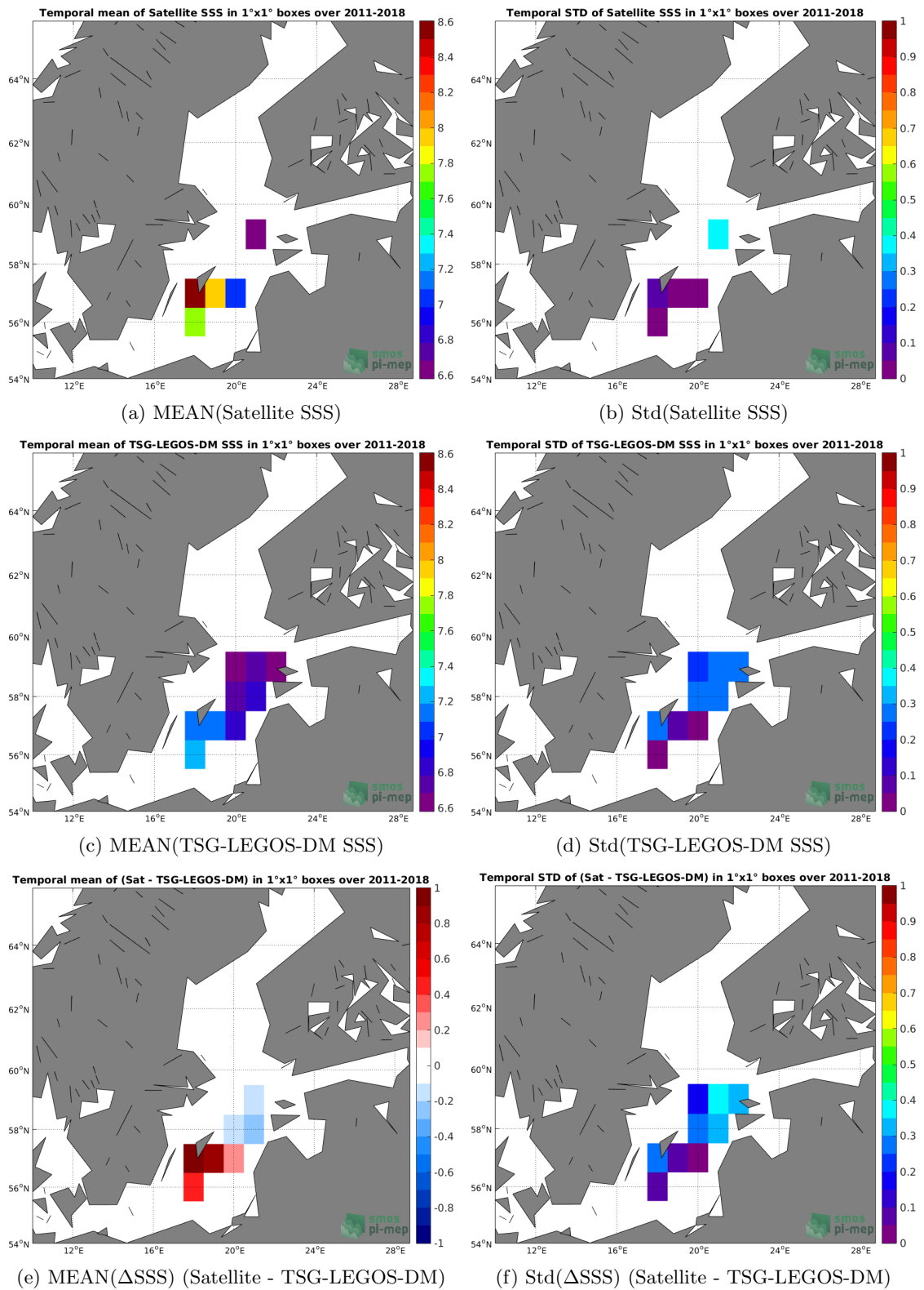
Figure 6: Temporal mean (left) and Std (right) of SSS from CCI L4 Merged-OI v1.8 - 7-day running (ESA) (top), TSG-LEGOS-DM (middle), and of \Delta SSS (Satellite - TSG-LEGOS-DM). Only match-up pairs are used to generate these maps.
