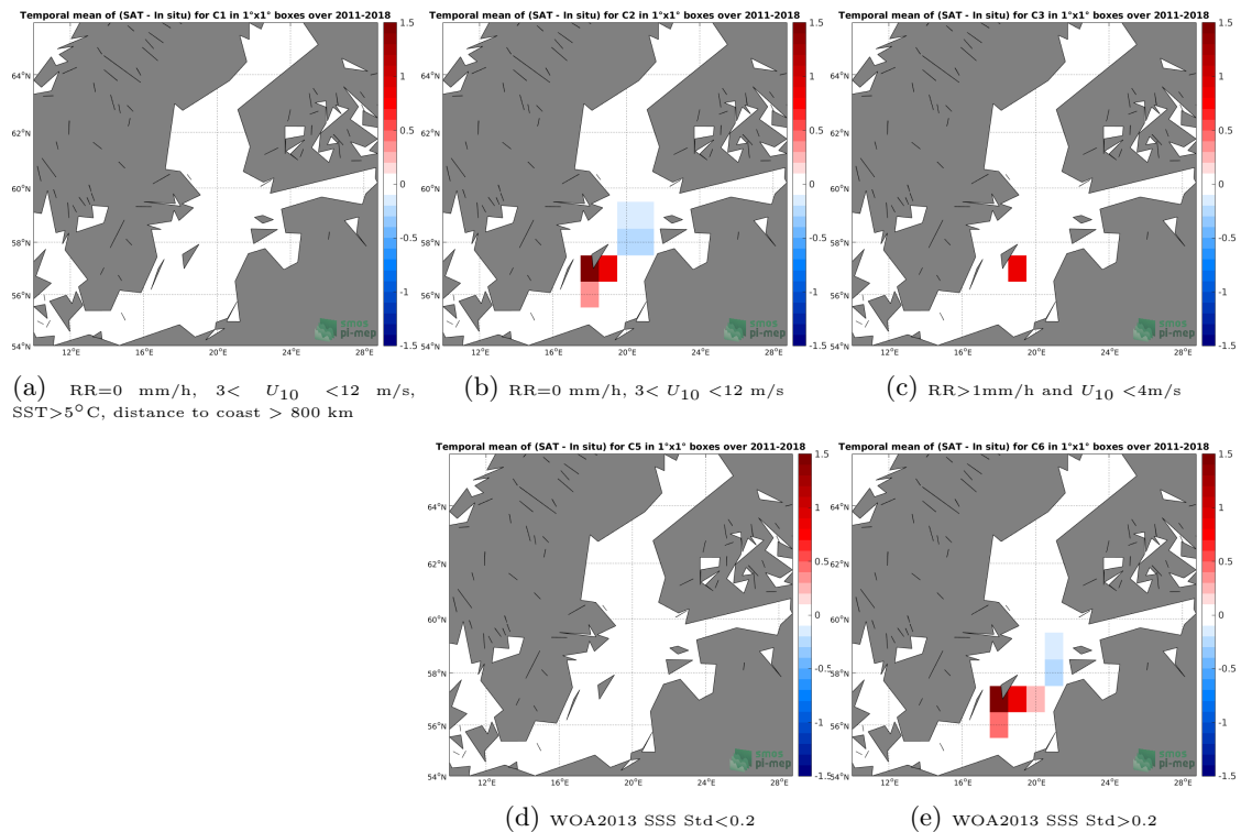
Figure 12: Temporal mean gridded over spatial boxes of size 1^{\circ}\times 1^{\circ} of \Delta\text{SSS} (CCI L4 Merged-OI v1.8 - 7-day running (ESA) - TSG-LEGOS-DM) for 5 different subdatasets corresponding to:RR=0 mm/h, 3 < U_{10} < 12 m/s, SST >5^{\circ}\text{C} , distance to coast > 800 km (a), RR=0 mm/h, 3 < U_{10} < 12 m/s (b), RR >1 mm/h and U_{10} < 4 m/s (c), WOA2013 SSS Std <0.2 (d), WOA2013 SSS Std >0.2 (e).
