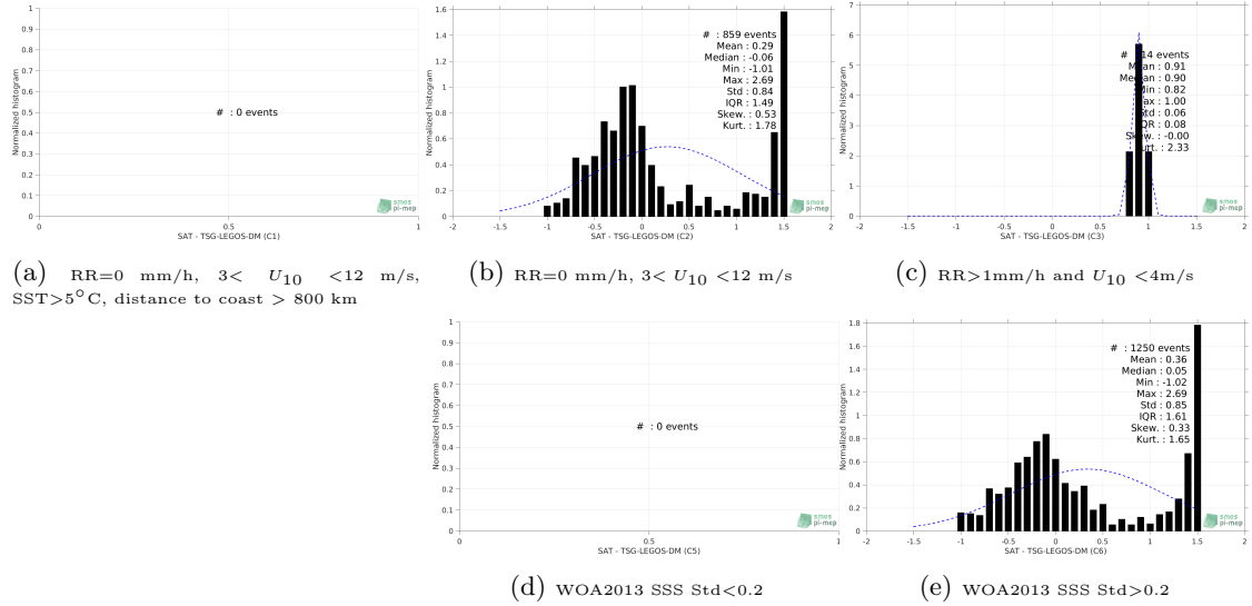
Figure 13: Normalized histogram of \Delta SSS (CCI L4 Merged-OI v1.8 - 30-day running (ESA) - TSG-LEGOS-DM) for 5 different subdatasets corresponding to: RR=0 mm/h, 3 < U_{10} < 12 m/s, SST >5^{\circ} C, distance to coast > 800 km (a), RR=0 mm/h, 3 < U_{10} < 12 m/s (b), RR >1 mm/h and U_{10} < 4 m/s (c), WOA2013 SSS Std <0.2 (d), WOA2013 SSS Std >0.2 (e).
