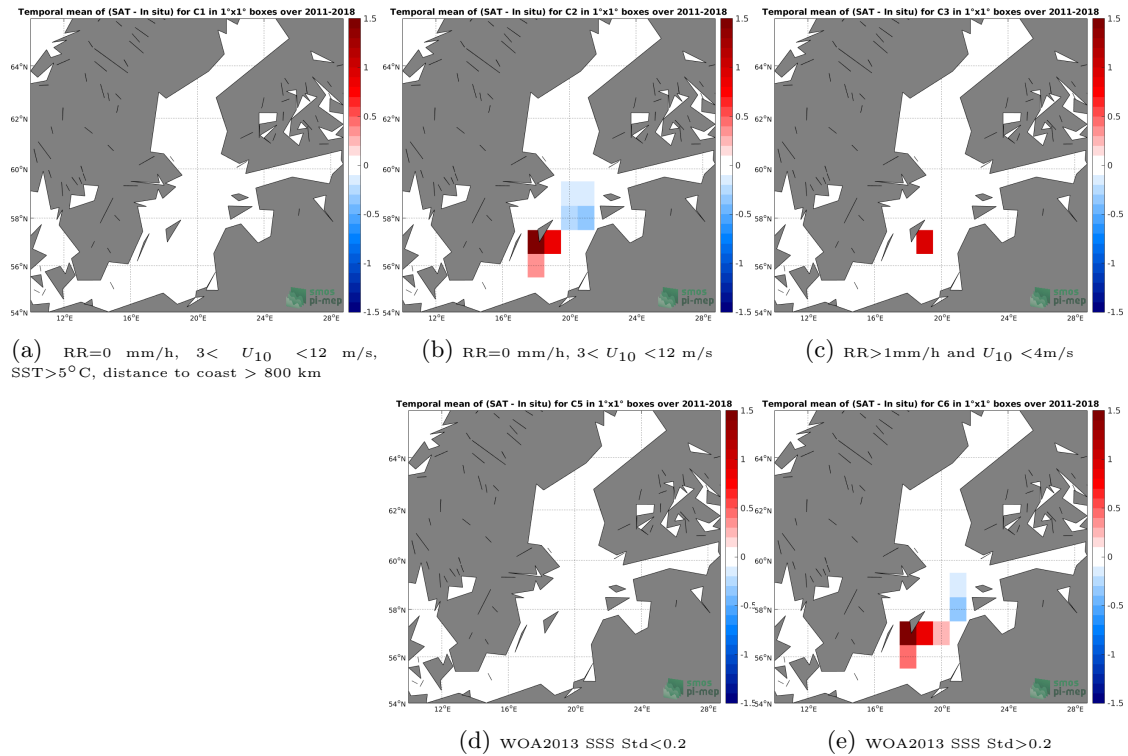
Figure 12: Temporal mean gridded over spatial boxes of size 1^{\circ}\times 1^{\circ} of \Delta\text{SSS} (CCI L4 Merged-OI v1.8 - 30-day running (ESA) - TSG-LEGOS-DM) for 5 different subdatasets corresponding to:RR=0 mm/h, 3 < U_{10} < 12 m/s, SST >5^{\circ}\text{C} , distance to coast > 800 km (a), RR=0 mm/h, 3 < U_{10} < 12 m/s (b), RR >1 mm/h and U_{10} < 4 m/s (c), WOA2013 SSS Std <0.2 (d), WOA2013 SSS Std >0.2 (e).
