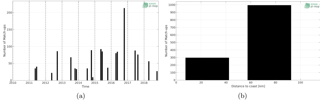
Figure 1: Number of match-ups between TSG-LEGOS-DM and CCI L4 Merged-OI v1.8 - 30-day running (ESA) SSS as a function of time (a) and as function of the distance to coast (b) over the Baltic Sea Pi-MEP region and for the full satellite product period.
