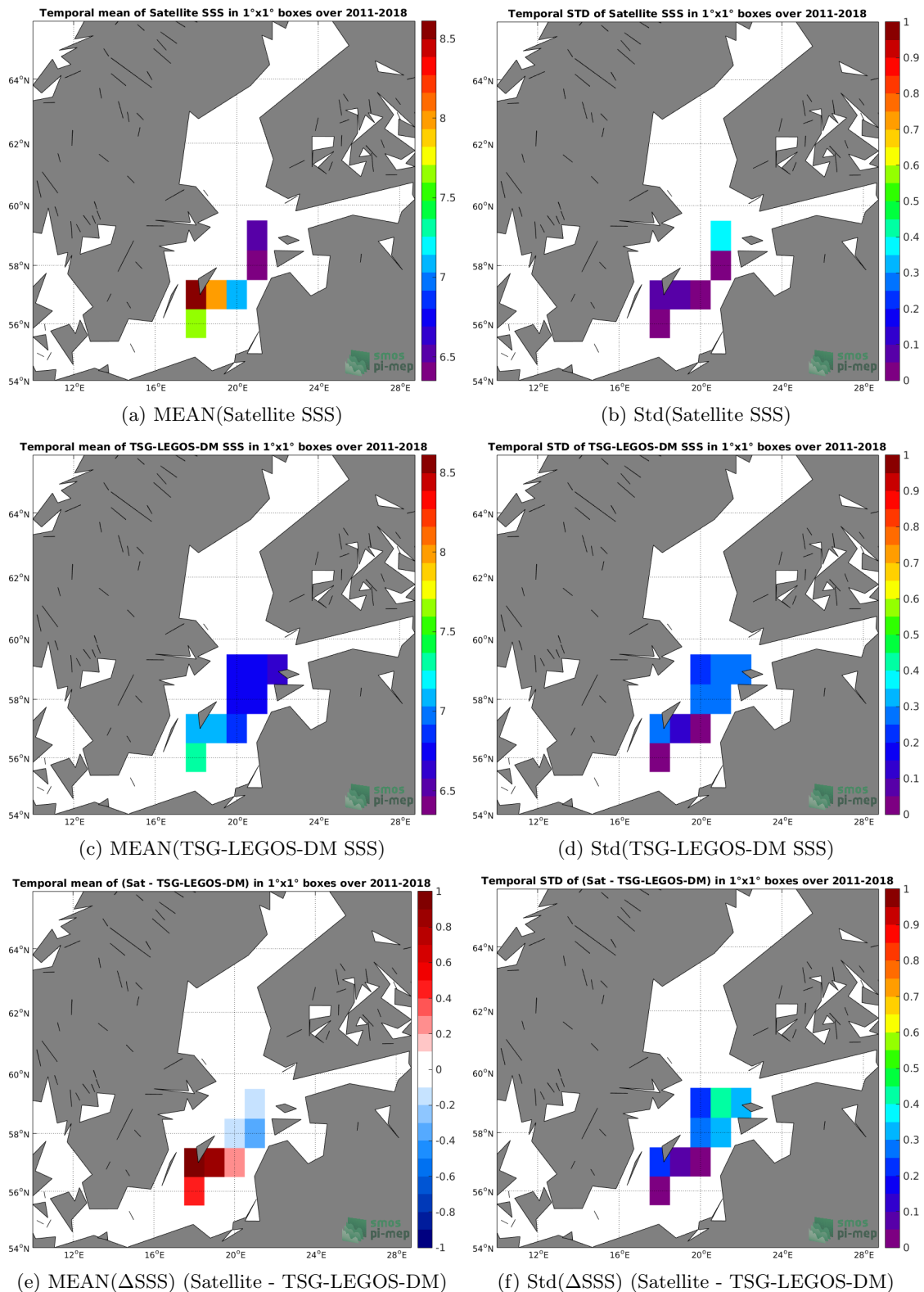
Figure 6: Temporal mean (left) and Std (right) of SSS from CCI L4 Merged-OI v1.8 - 30-day running (ESA) (top), TSG-LEGOS-DM (middle), and of \Delta SSS (Satellite - TSG-LEGOS-DM). Only match-up pairs are used to generate these maps.
