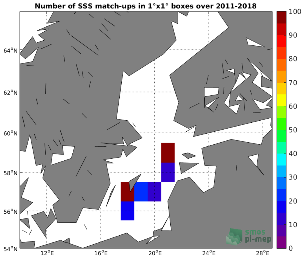
Figure 4: Number of SSS match-ups between TSG-LEGOS-DM SSS and the CCI L4 Merged-OI v1.8 - 30-day running (ESA) SSS product for the Baltic Sea Pi-MEP region over 1°x1° boxes and for the full satellite product period.
